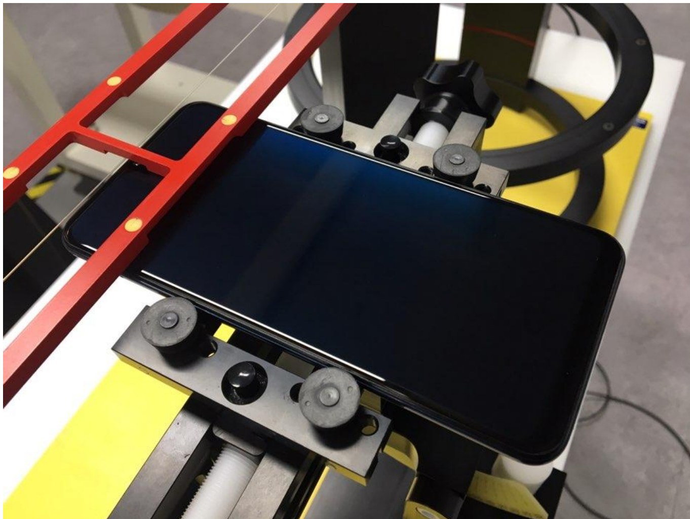
Setup Photo Front View of the DUT
