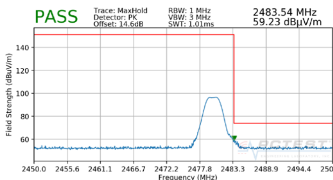
Plot 7-30. Radiated Restricted Upper Band Edge Measurement (Peak)
