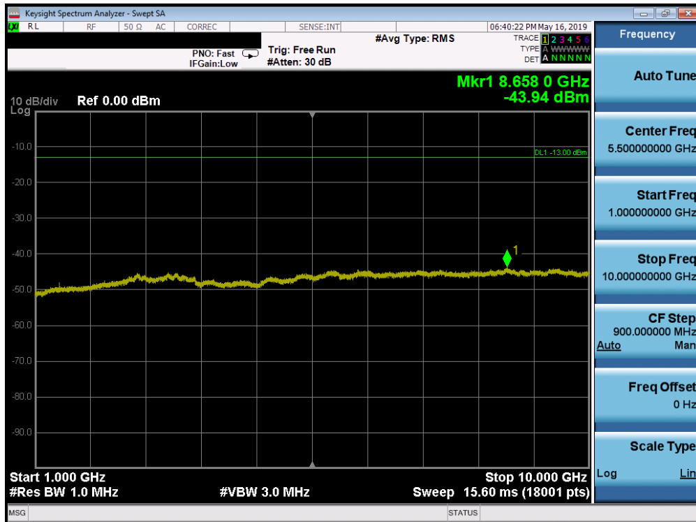
Plot 7-129. Conducted Spurious Plot (Band 12/17 - 10.0MHz QPSK - RB Size 1, RB Offset 0 - Low Channel)
