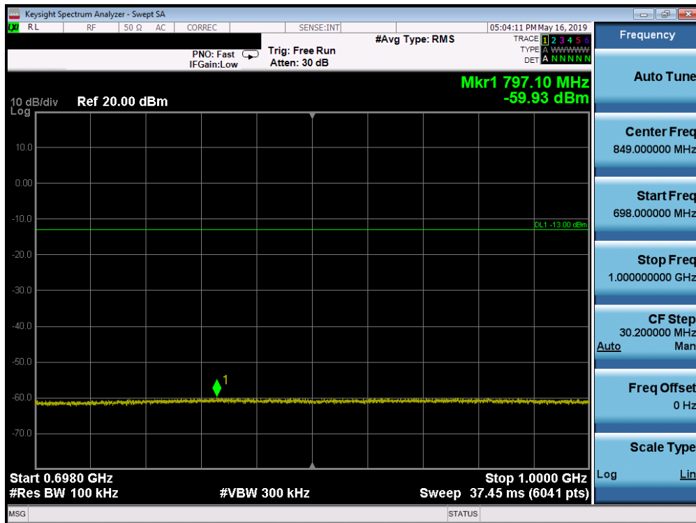
Plot 7-119. Conducted Spurious Plot (Band 71 - 5.0MHz QPSK - RB Size 1, RB Offset 0 - Low Channel)
