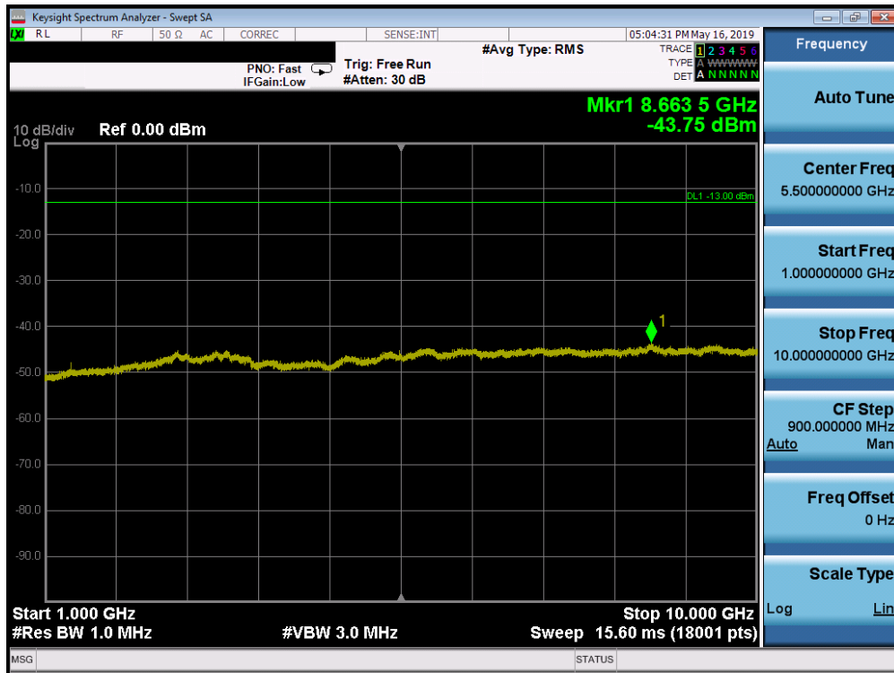
Plot 7-120. Conducted Spurious Plot (Band 71 - 5.0MHz QPSK - RB Size 1, RB Offset 0 - Low Channel)
