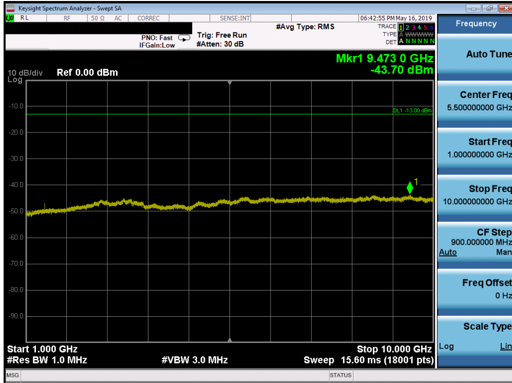
Plot 7-135. Conducted Spurious Plot (Band 12/17 - 10.0MHz QPSK - RB Size 1, RB Offset 0 - High Channel)
