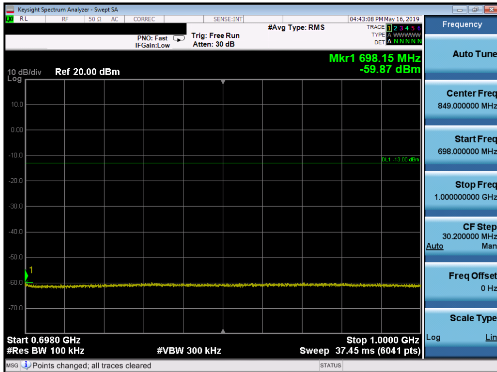
Plot 7-122. Conducted Spurious Plot (Band 71 - 5.0MHz QPSK - RB Size 1, RB Offset 0 - Mid Channel)
