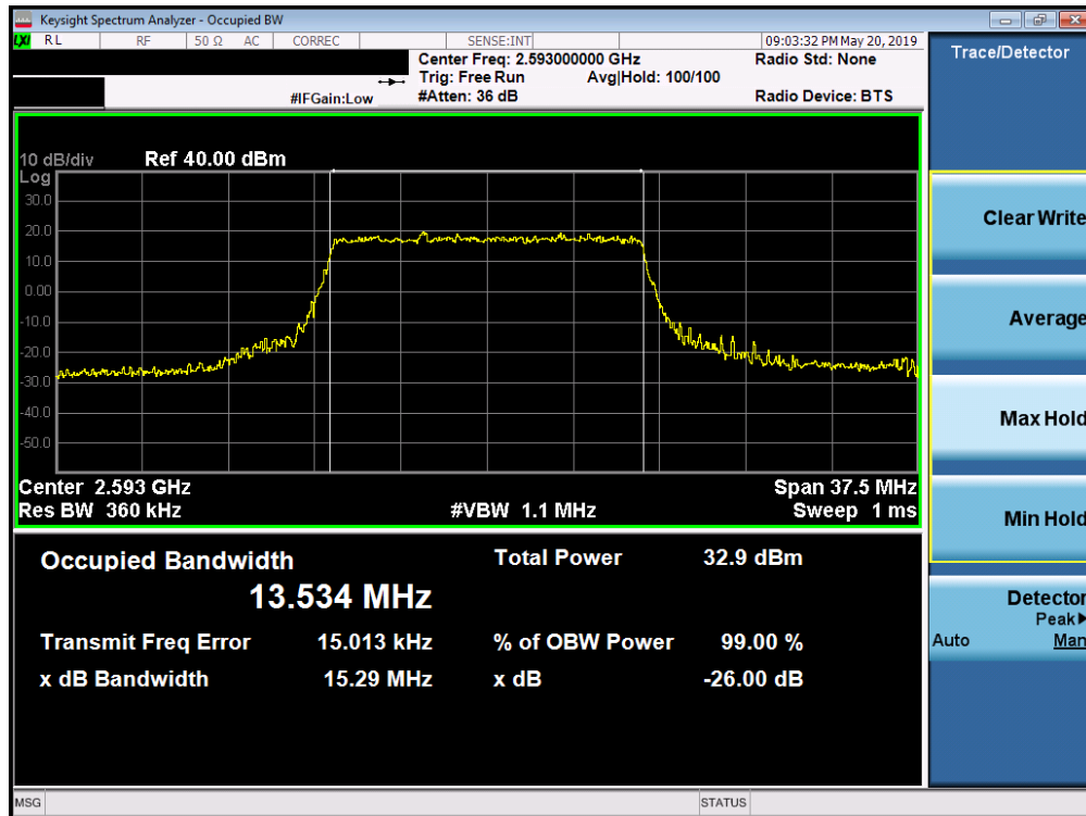
Plot 7-114. Occupied Bandwidth Plot (Band41 PC3 - 15.0MHz 64-QAM - Full RB Configuration)
