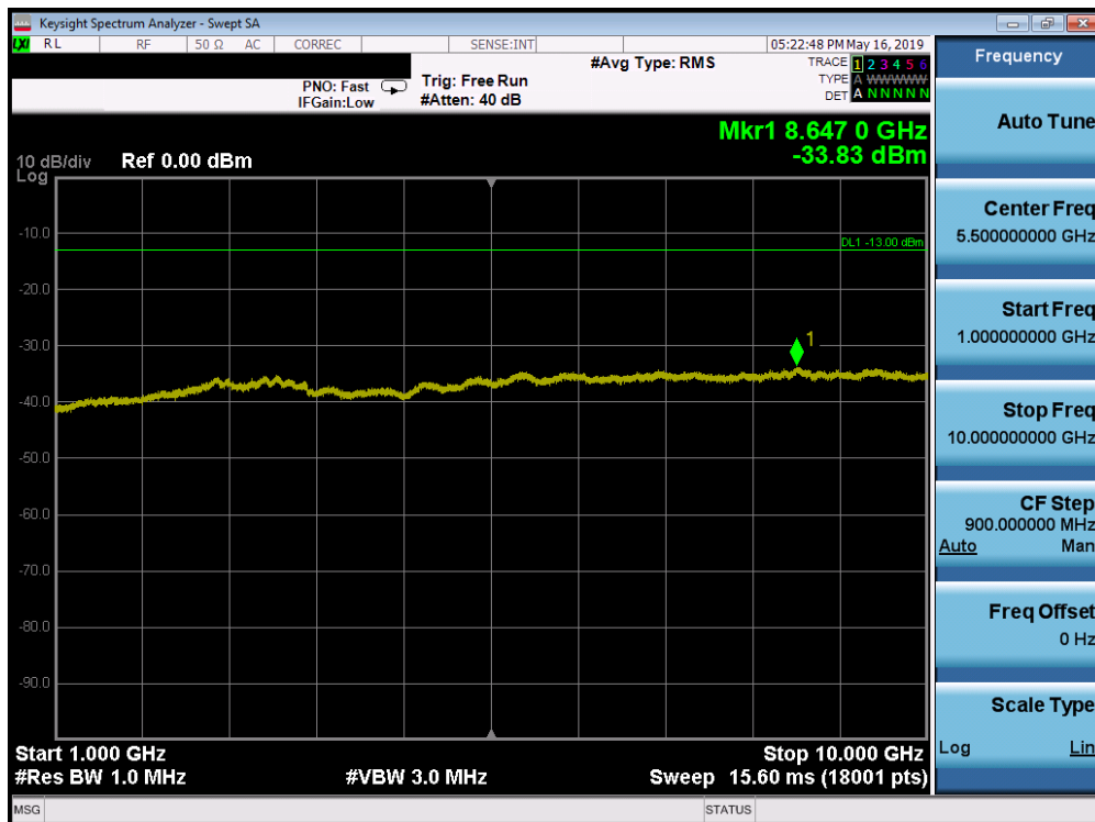
Plot 7-132. Conducted Spurious Plot (Band 12/17 - 10.0MHz QPSK - RB Size 1, RB Offset 0 - Mid Channel)
