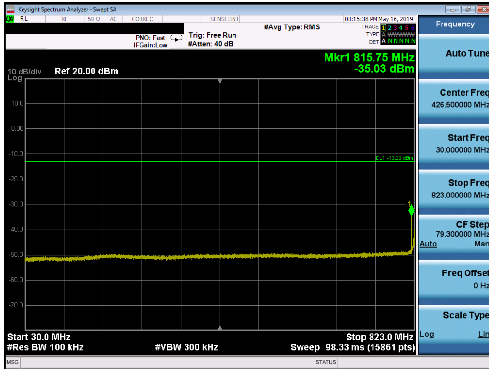
Plot 7-145. Conducted Spurious Plot (Band 26/5 - 5.0MHz QPSK - RB Size 1, RB Offset 0 – Low Channel)
