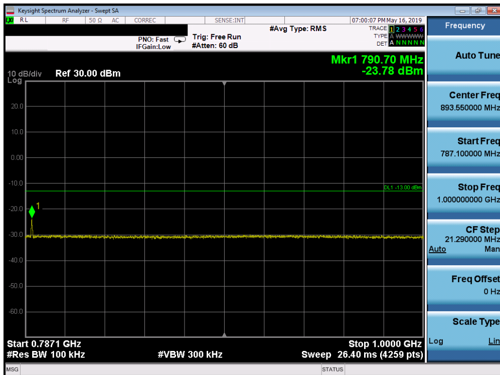
Plot 7-143. Conducted Spurious Plot (Band 13 - 5.0MHz QPSK - RB Size 1, RB Offset 0 - High Channel)
