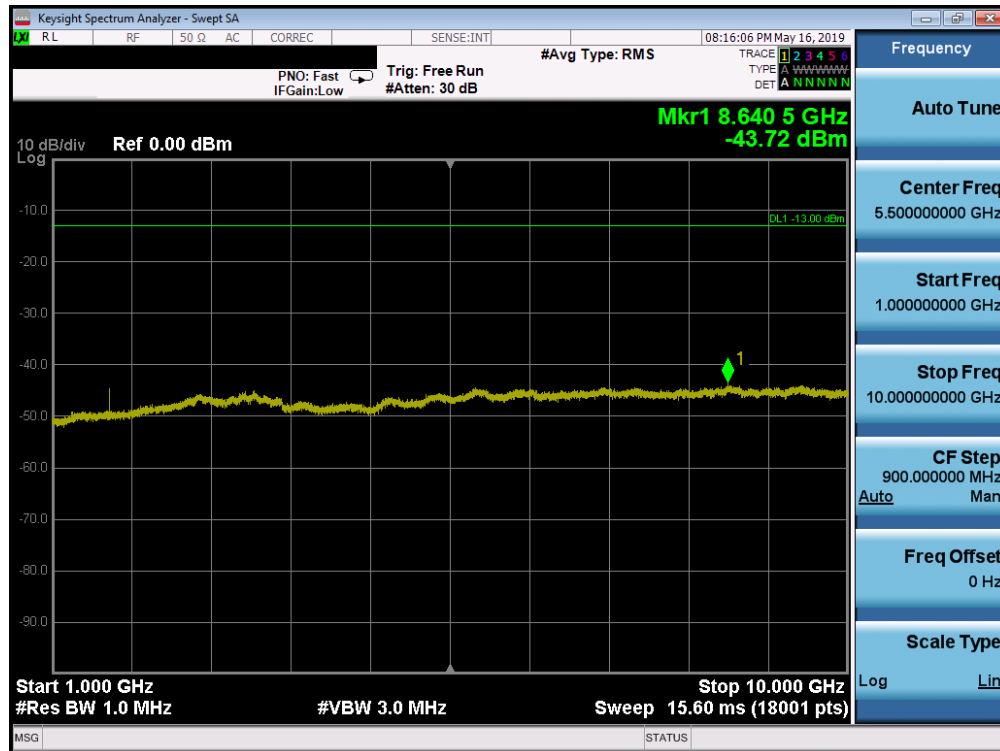
Plot 7-147. Conducted Spurious Plot (Band 26/5 - 5.0MHz QPSK - RB Size 1, RB Offset 0 – Low Channel)
