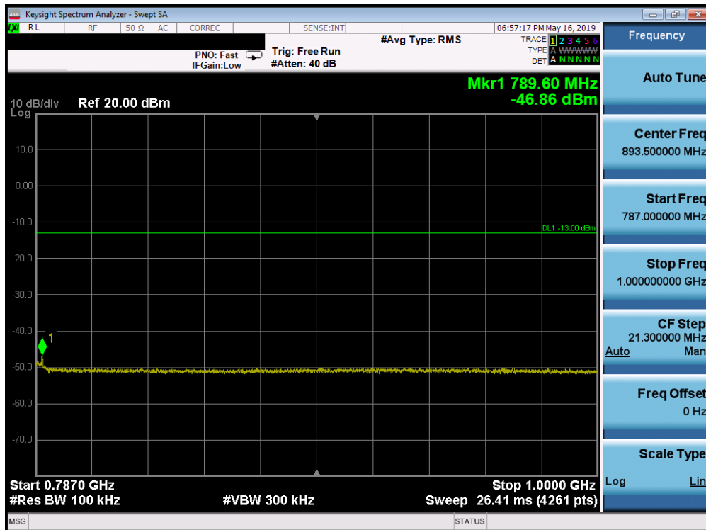
Plot 7-137. Conducted Spurious Plot (Band 13 - 5.0MHz QPSK - RB Size 1, RB Offset 0 - Low Channel)
