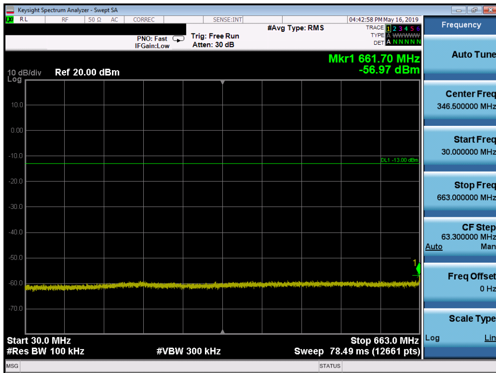
Plot 7-121. Conducted Spurious Plot (Band 71 - 5.0MHz QPSK - RB Size 1, RB Offset 0 - Mid Channel)
