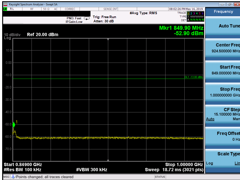
Plot 7-149. Conducted Spurious Plot (Band 26/5 - 5.0MHz QPSK - RB Size 1, RB Offset 0 – Mid Channel)
