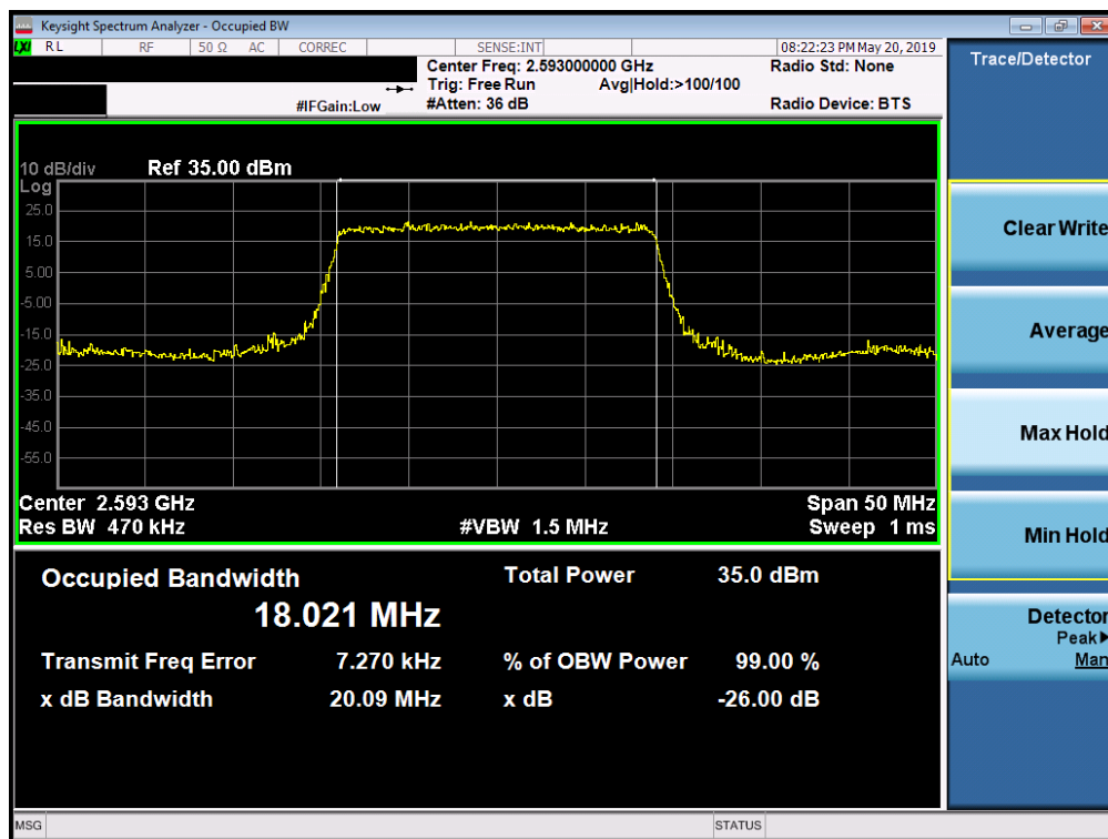
Plot 7-115. Occupied Bandwidth Plot (Band 41 PC3 - 20.0MHz QPSK - Full RB Configuration)
