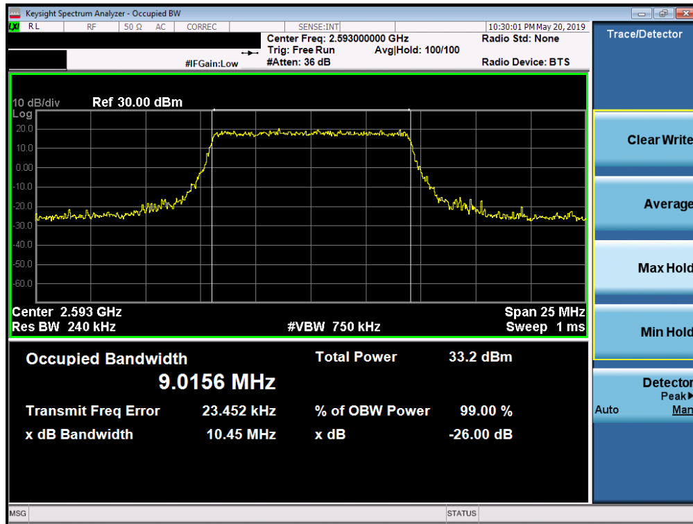
Plot 7-110. Occupied Bandwidth Plot (Band 41 PC3 - 10.0MHz 16-QAM - Full RB Configuration)
