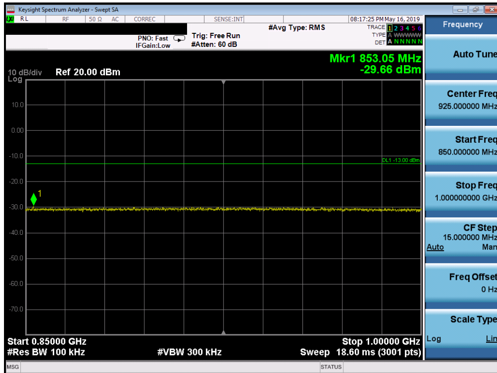
Plot 7-152. Conducted Spurious Plot (Band 26/5 - 5.0MHz QPSK - RB Size 1, RB Offset 0 – High Channel)
