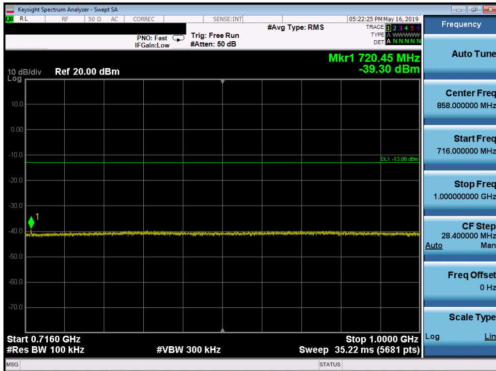
Plot 7-131. Conducted Spurious Plot (Band 12/17 - 10.0MHz QPSK - RB Size 1, RB Offset 0 - Mid Channel)
