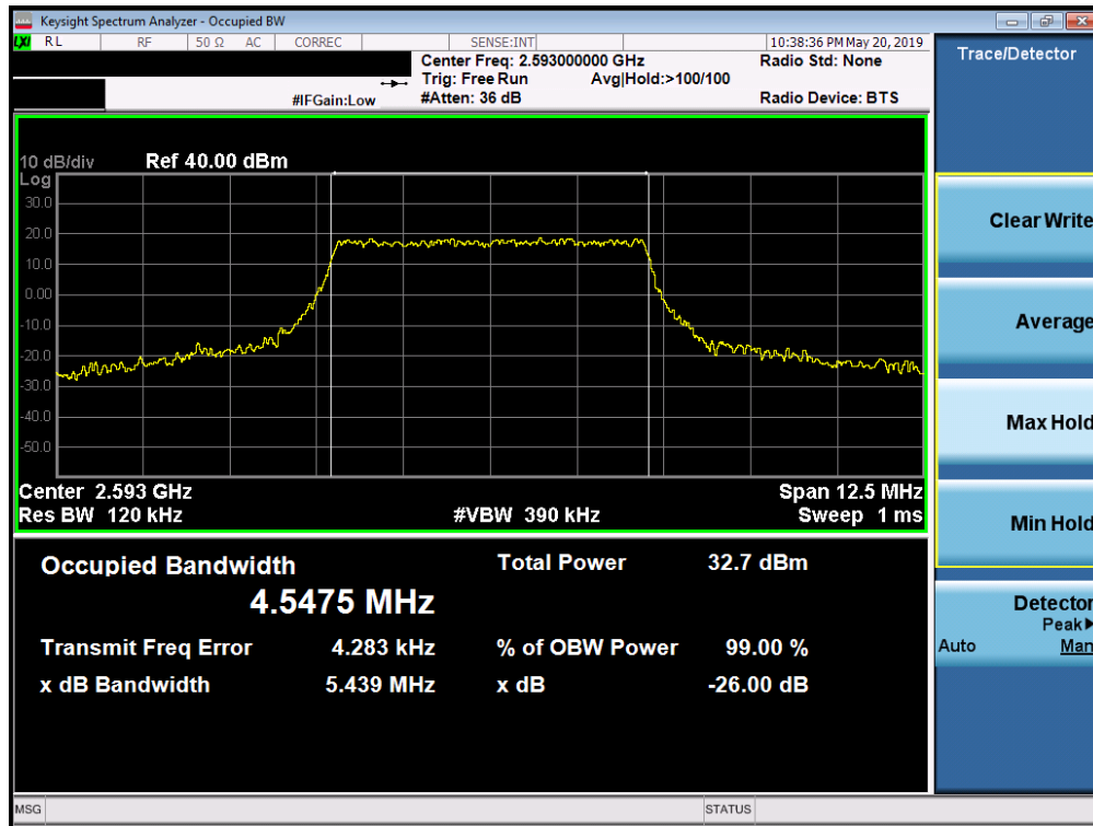
Plot 7-108. Occupied Bandwidth Plot (Band41 PC3 - 5.0MHz 64-QAM - Full RB Configuration)
