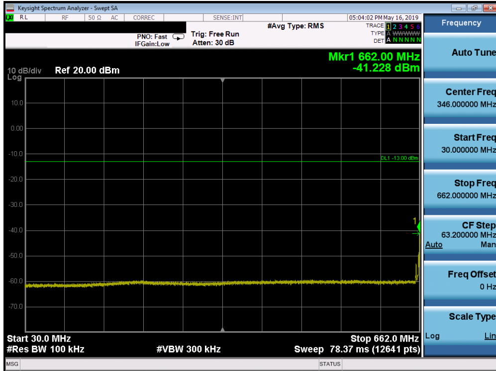
Plot 7-118. Conducted Spurious Plot (Band 71 - 5.0MHz QPSK - RB Size 1, RB Offset 0 - Low Channel)
