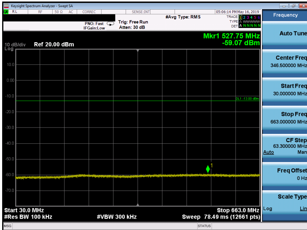
Plot 7-124. Conducted Spurious Plot (Band 71 - 5.0MHz QPSK - RB Size 1, RB Offset 0 - High Channel)
