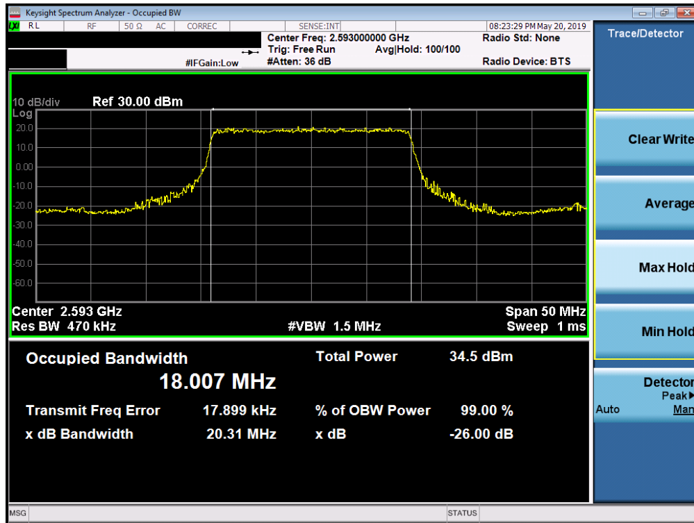
Plot 7-116. Occupied Bandwidth Plot (Band 41 PC3 - 20.0MHz 16-QAM - Full RB Configuration)
