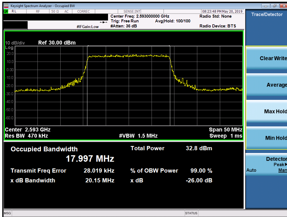
Plot 7-117. Occupied Bandwidth Plot (Band41 PC3 - 20.0MHz 64-QAM - Full RB Configuration)
