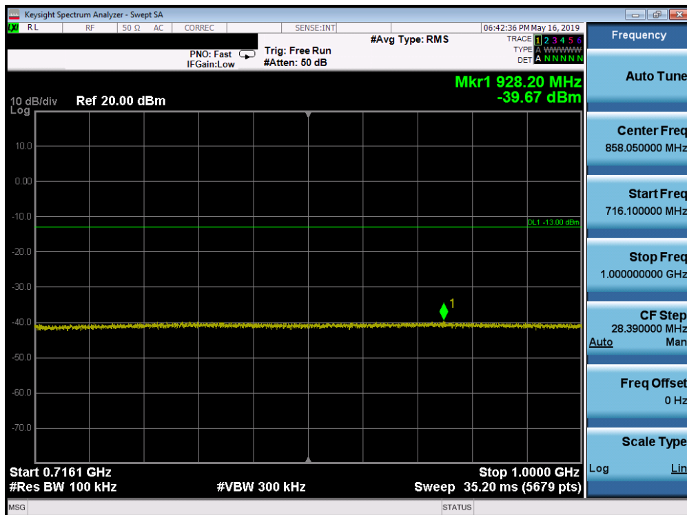
Plot 7-134. Conducted Spurious Plot (Band 12/17 - 10.0MHz QPSK - RB Size 1, RB Offset 0 - High Channel)
