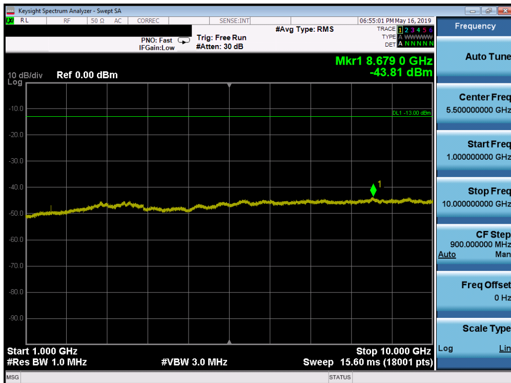
Plot 7-141. Conducted Spurious Plot (Band 13 - 5.0MHz QPSK - RB Size 1, RB Offset 0 - Mid Channel)
