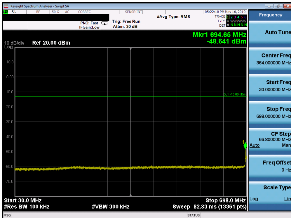
Plot 7-130. Conducted Spurious Plot (Band 12/17 - 10.0MHz QPSK - RB Size 1, RB Offset 0 - Mid Channel)
