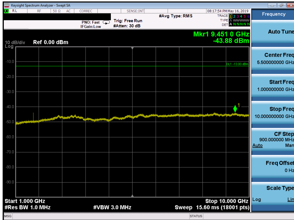
Plot 7-153. Conducted Spurious Plot (Band 26/5 - 5.0MHz QPSK - RB Size 1, RB Offset 0 – High Channel)
