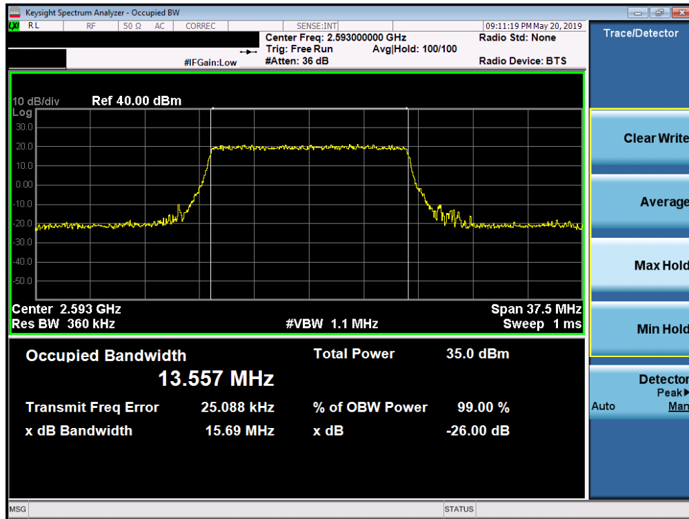
Plot 7-112. Occupied Bandwidth Plot (Band 41 PC3 - 15.0MHz QPSK - Full RB Configuration)
