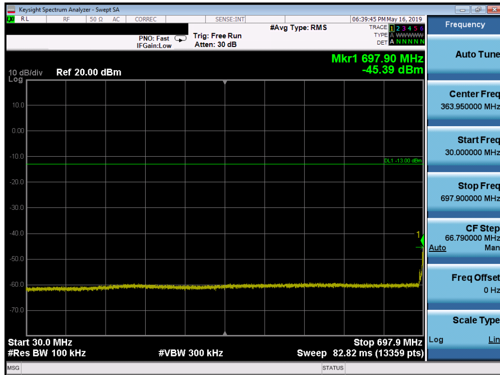
Plot 7-127. Conducted Spurious Plot (Band 12/17 - 10.0MHz QPSK - RB Size 1, RB Offset 0 - Low Channel)
