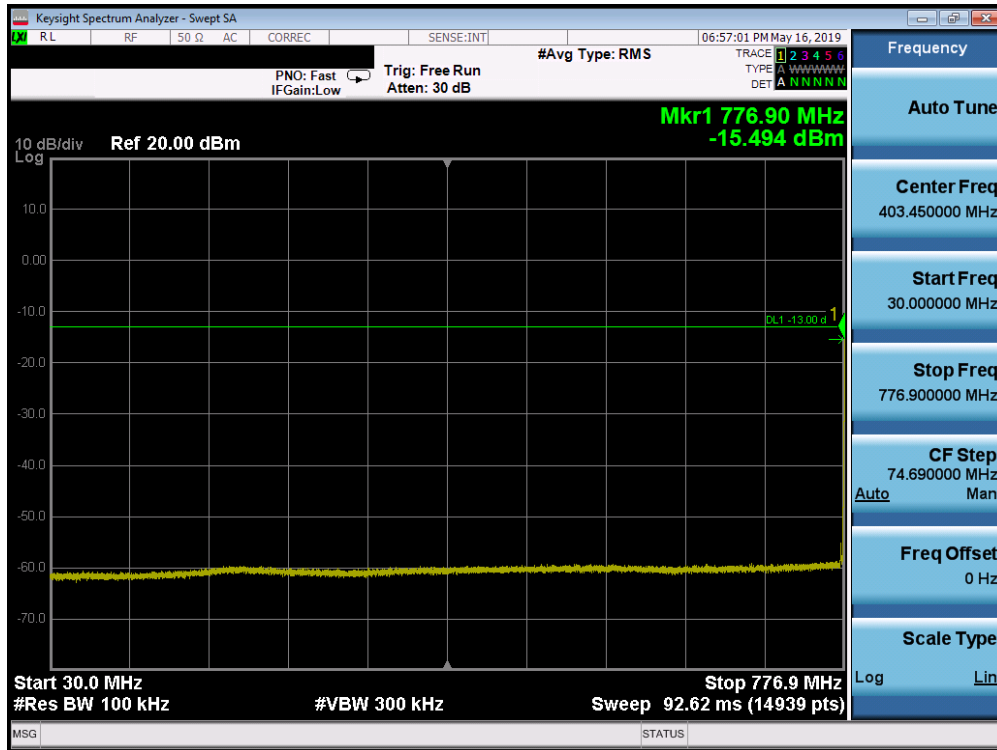
Plot 7-136. Conducted Spurious Plot (Band 13 - 5.0MHz QPSK - RB Size 1, RB Offset 0 - Low Channel)
