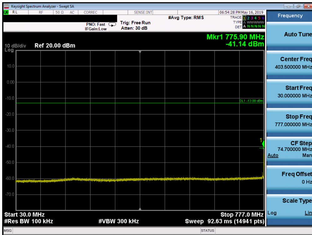
Plot 7-139. Conducted Spurious Plot (Band 13 - 5.0MHz QPSK - RB Size 1, RB Offset 0 - Mid Channel)
