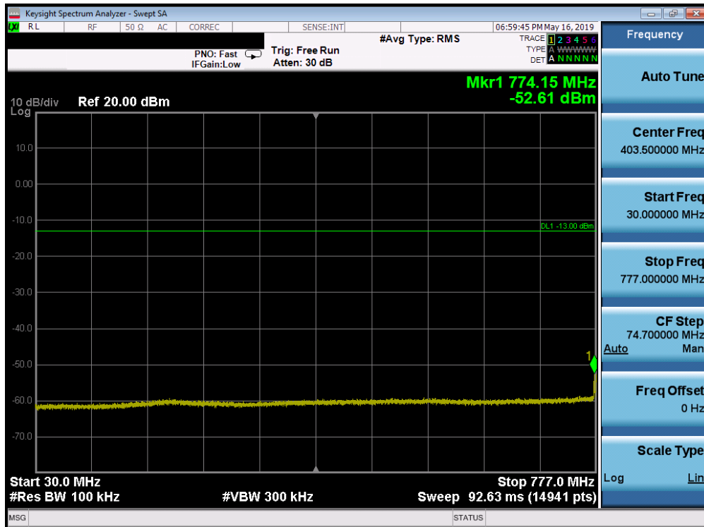
Plot 7-142. Conducted Spurious Plot (Band 13 - 5.0MHz QPSK - RB Size 1, RB Offset 0 - High Channel)
