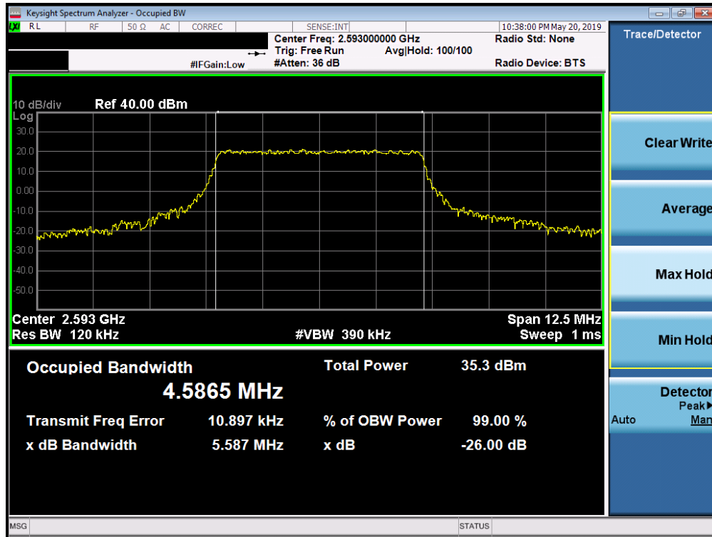
Plot 7-106. Occupied Bandwidth Plot (Band 41 PC3 - 5.0MHz QPSK - Full RB Configuration)
