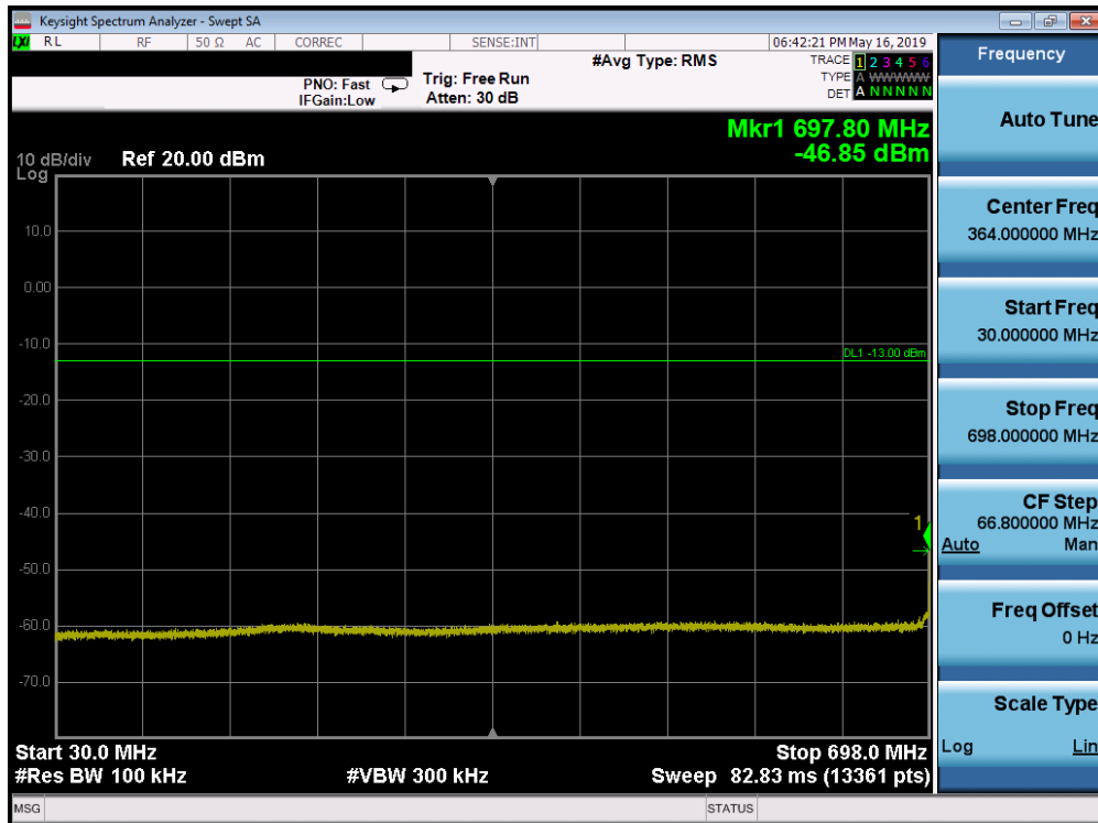
Plot 7-133. Conducted Spurious Plot (Band 12/17 - 10.0MHz QPSK - RB Size 1, RB Offset 0 - High Channel)
