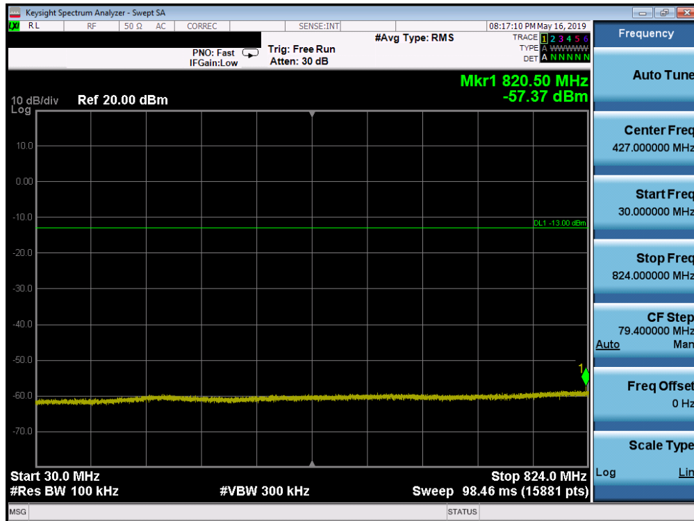
Plot 7-151. Conducted Spurious Plot (Band 26/5 - 5.0MHz QPSK - RB Size 1, RB Offset 0 – High Channel)
