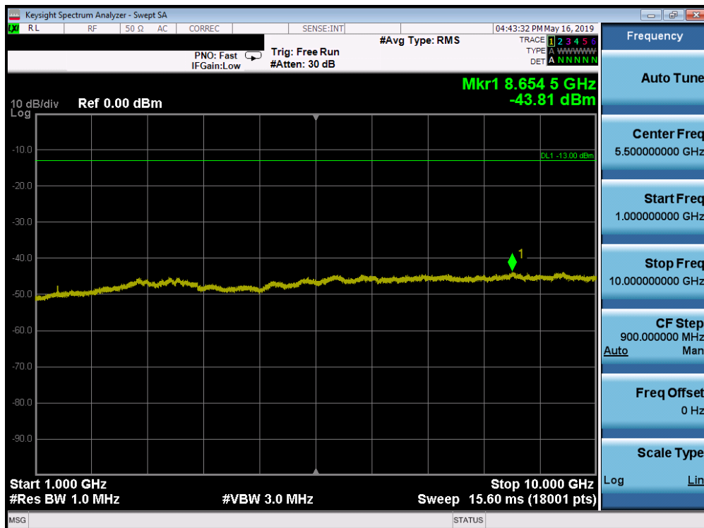
Plot 7-123. Conducted Spurious Plot (Band 71 - 5.0MHz QPSK - RB Size 1, RB Offset 0 - Mid Channel)
