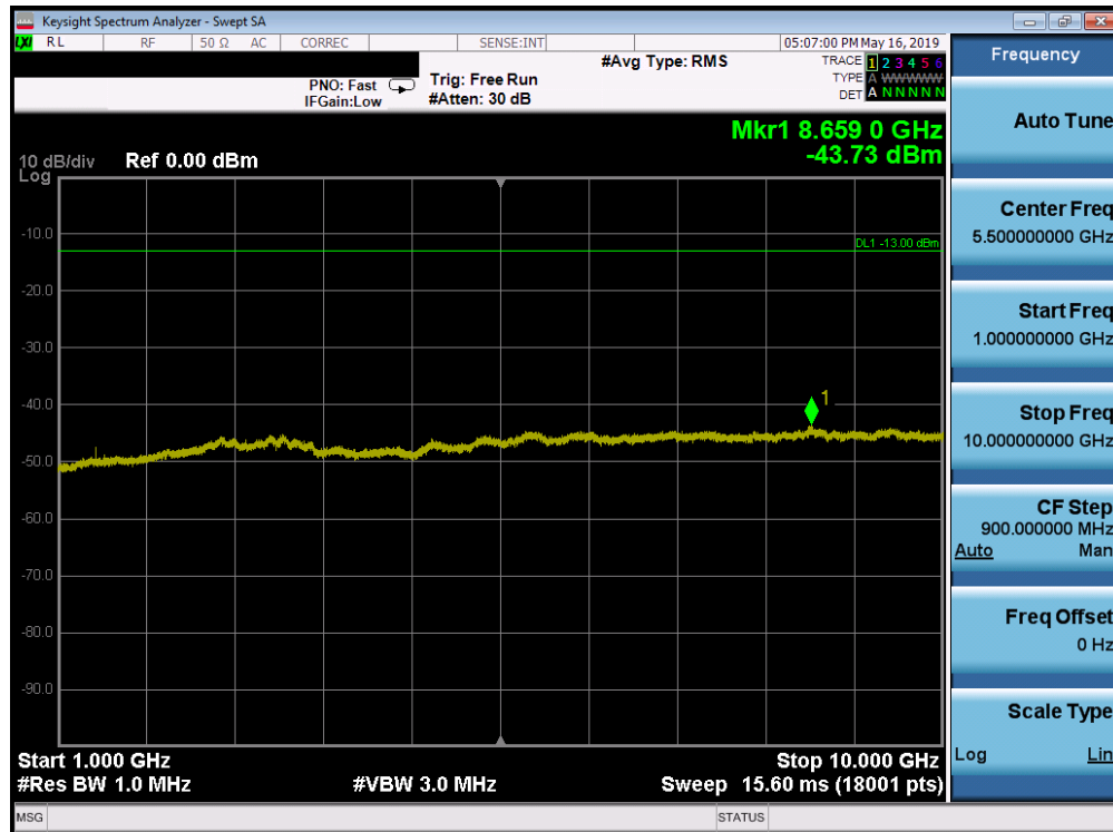
Plot 7-126. Conducted Spurious Plot (Band 71 - 5.0MHz QPSK - RB Size 1, RB Offset 0 - High Channel)
