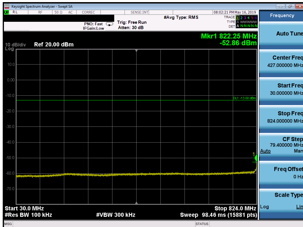
Plot 7-148. Conducted Spurious Plot (Band 26/5 - 5.0MHz QPSK - RB Size 1, RB Offset 0 – Mid Channel)
