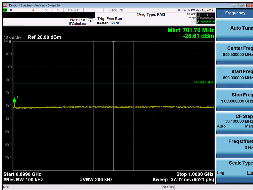
Plot 7-125. Conducted Spurious Plot (Band 71 - 5.0MHz QPSK - RB Size 1, RB Offset 0 - High Channel)
