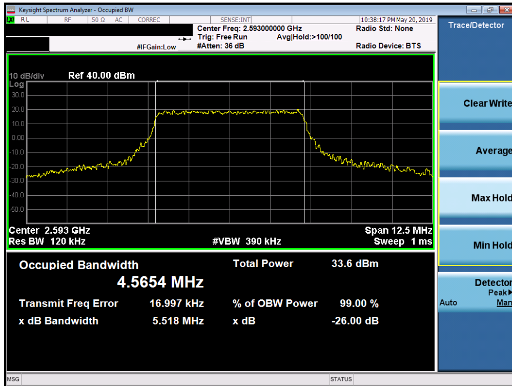
Plot 7-107. Occupied Bandwidth Plot (Band 41 PC3 - 5.0MHz 16-QAM - Full RB Configuration)
