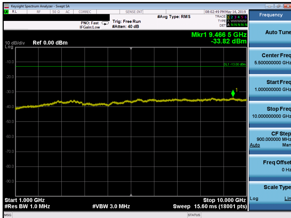
Plot 7-150. Conducted Spurious Plot (Band 26/5 - 5.0MHz QPSK - RB Size 1, RB Offset 0 – Mid Channel)
