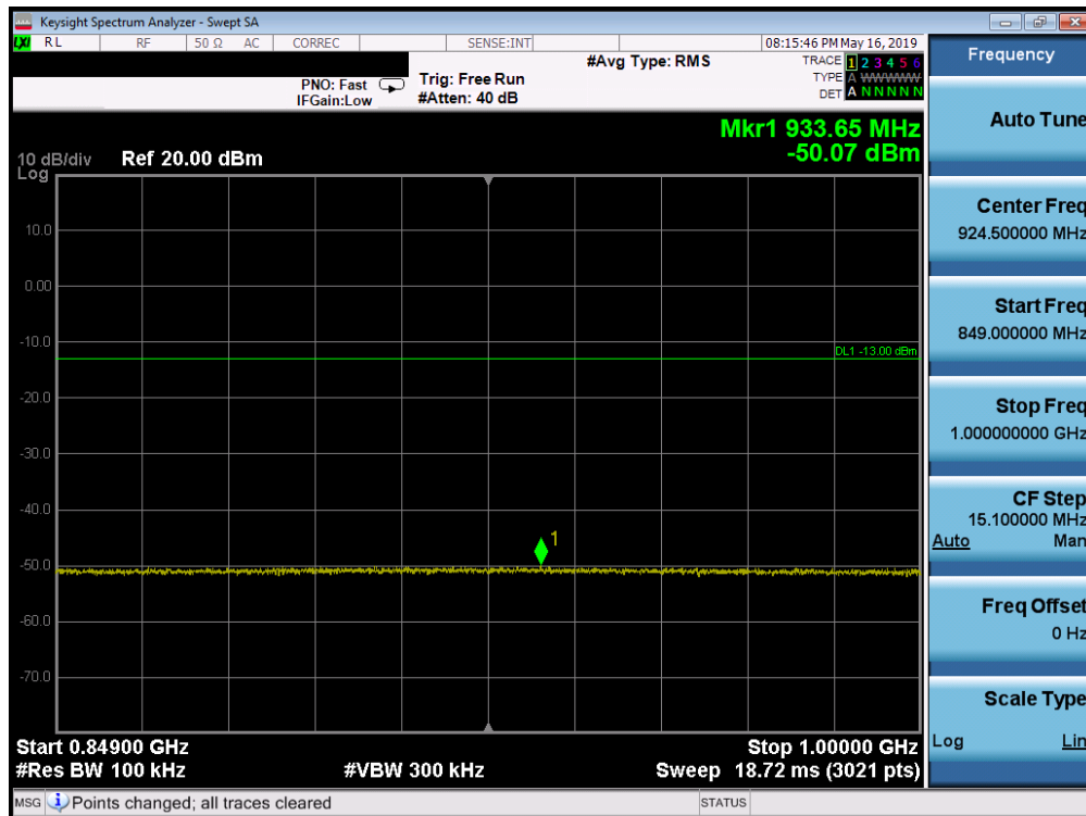
Plot 7-146. Conducted Spurious Plot (Band 26/5 - 5.0MHz QPSK - RB Size 1, RB Offset 0 – Low Channel)
