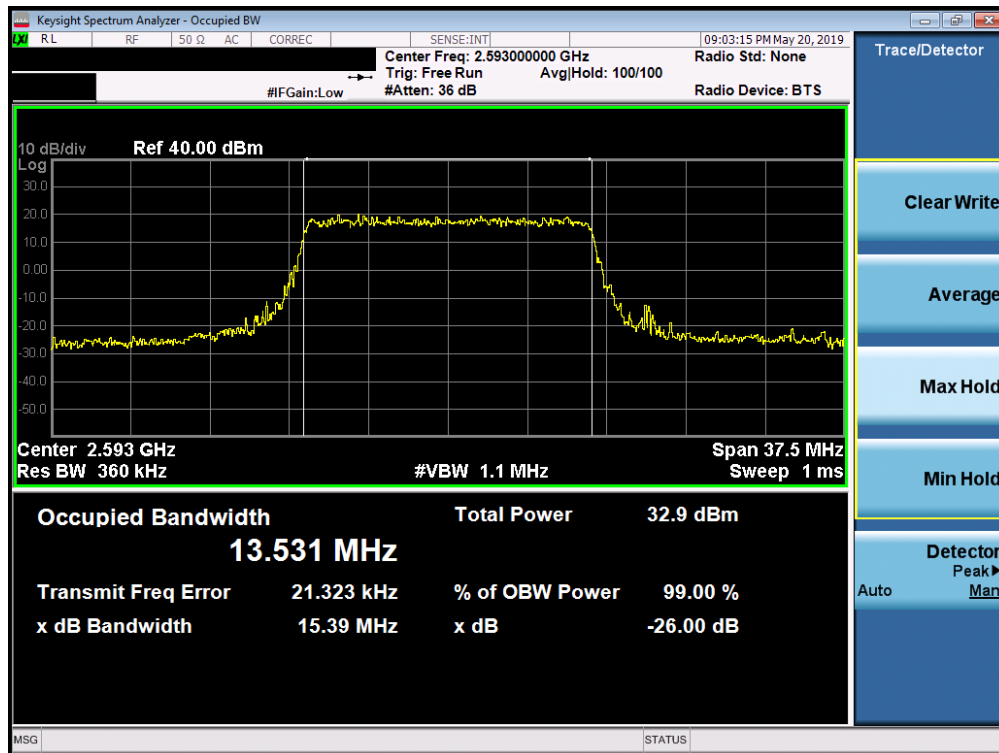
Plot 7-113. Occupied Bandwidth Plot (Band 41 PC3 - 15.0MHz 16-QAM - Full RB Configuration)
