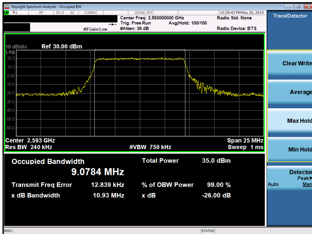
Plot 7-109. Occupied Bandwidth Plot (Band 41 PC3 - 10.0MHz QPSK - Full RB Configuration)
