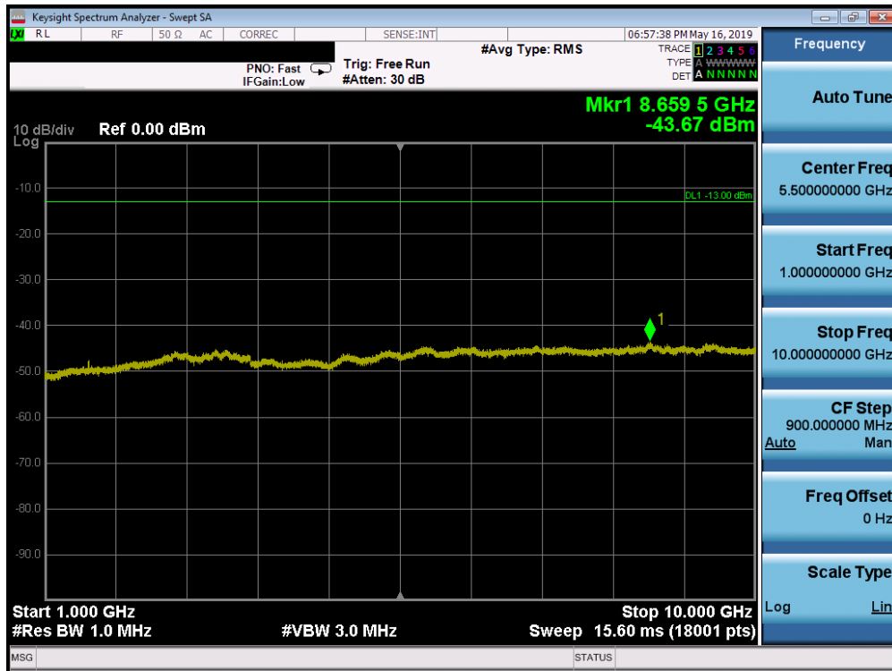
Plot 7-138. Conducted Spurious Plot (Band 13 - 5.0MHz QPSK - RB Size 1, RB Offset 0 - Low Channel)
