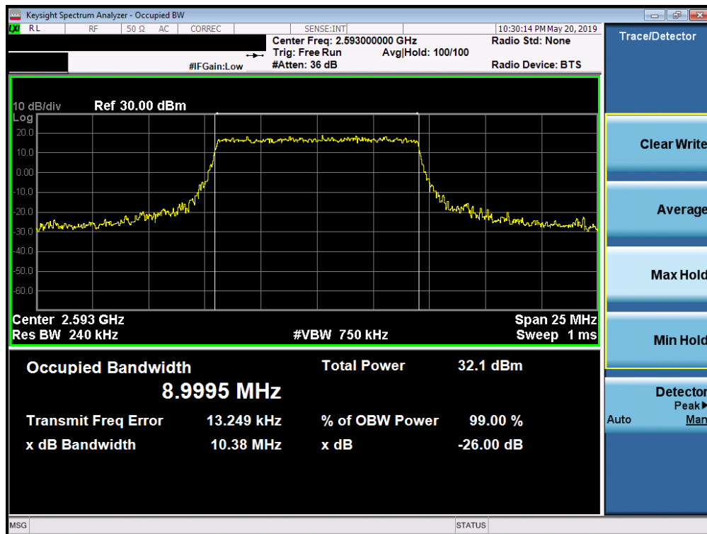
Plot 7-111. Occupied Bandwidth Plot (Band 41 PC3 - 10.0MHz 64-QAM - Full RB Configuration)
