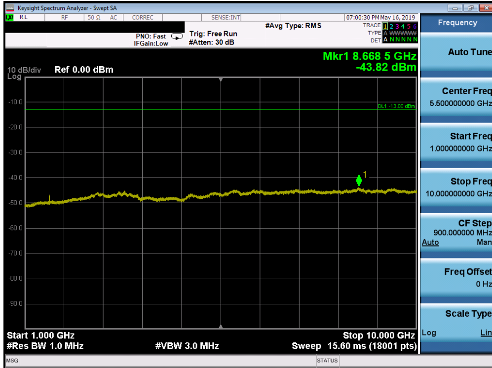
Plot 7-144. Conducted Spurious Plot (Band 13 - 5.0MHz QPSK - RB Size 1, RB Offset 0 - High Channel)
