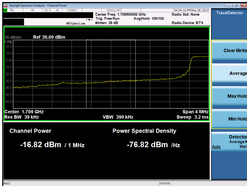
Plot 7-233. Lower Extended Band Edge Plot (Band 66/4 - 3.0MHz QPSK - Full RB Configuration)
