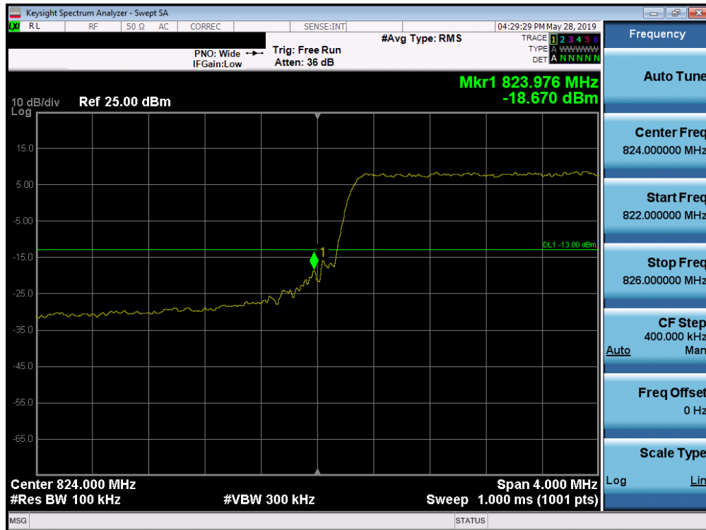
Plot 7-220. Lower Band Edge Plot (Band 26/5 – 5.0MHz QPSK - Full RB Configuration)
