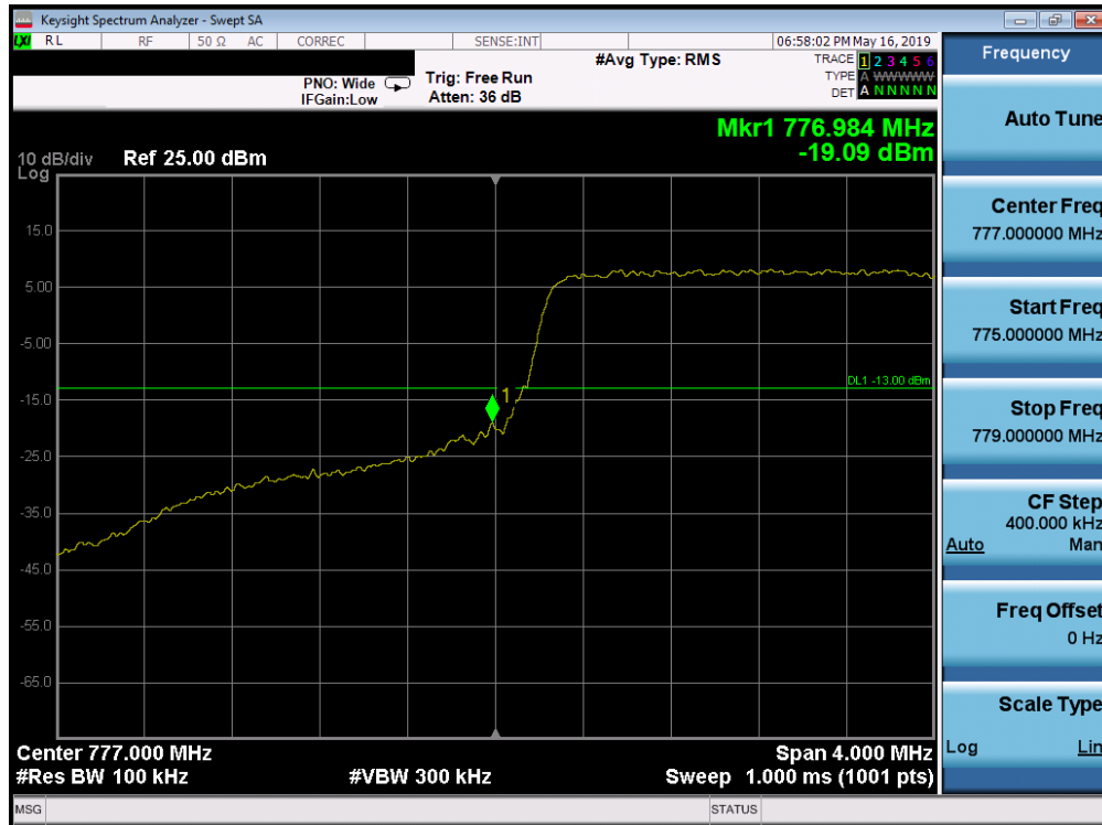
Plot 7-208. Lower Band Edge Plot (Band 13 - 5.0MHz QPSK - Full RB Configuration)
