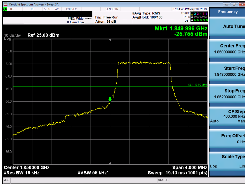
Plot 7-262. Lower Band Edge Plot (Band 25/2 - 1.4MHz QPSK - Full RB Configuration)
