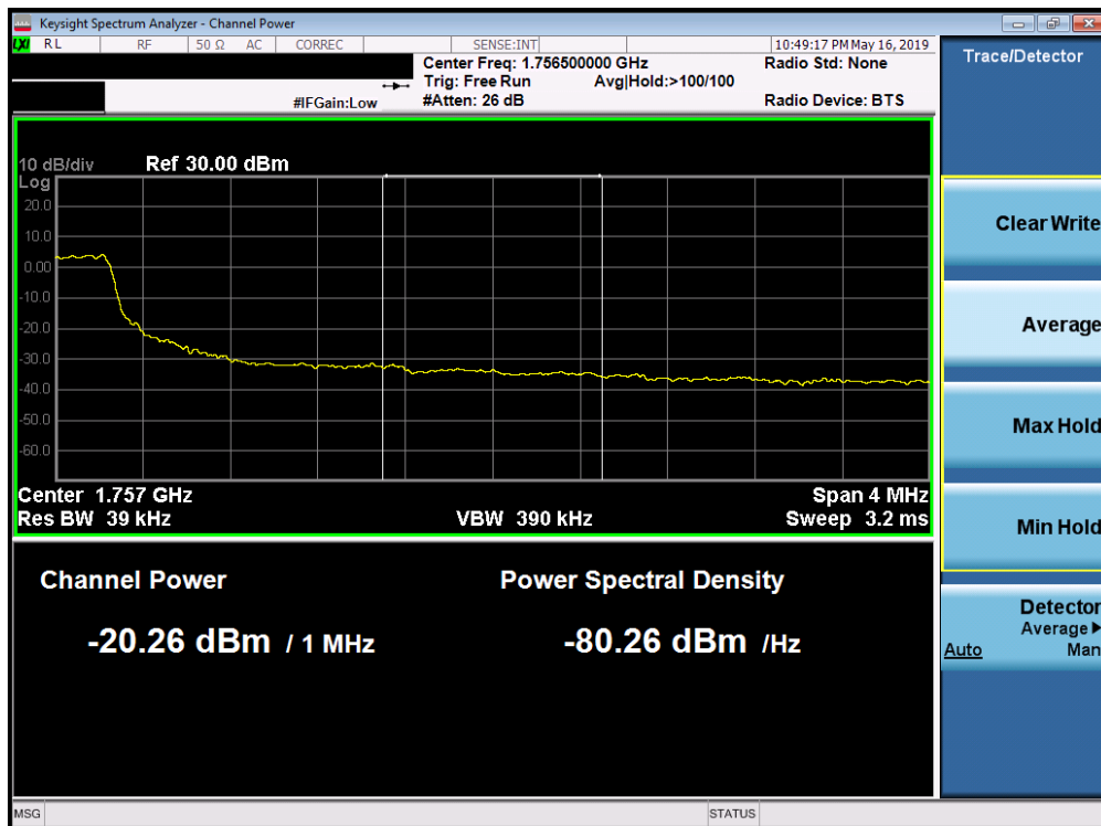
Plot 7-241. Upper Extended Band Edge Plot (Band 4 - 5.0MHz QPSK - Full RB Configuration)
