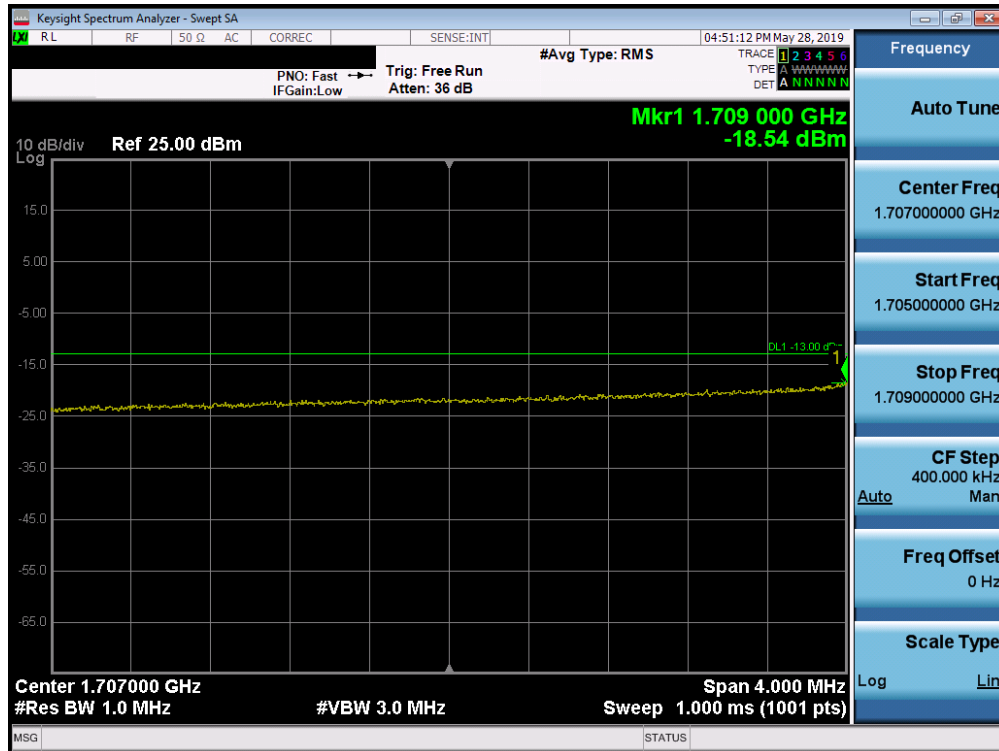
Plot 7-245. Lower Extended Band Edge Plot (Band 66/4 - 10.0MHz QPSK - Full RB Configuration)
