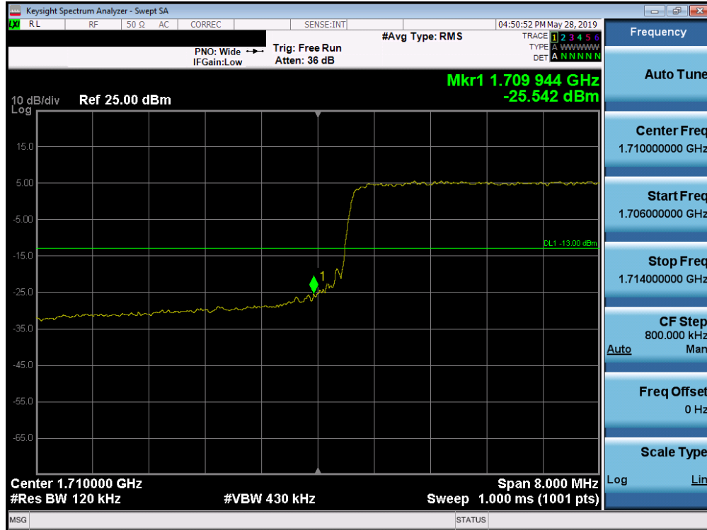
Plot 7-244. Lower Band Edge Plot (Band 66/4 - 10.0MHz QPSK - Full RB Configuration)
