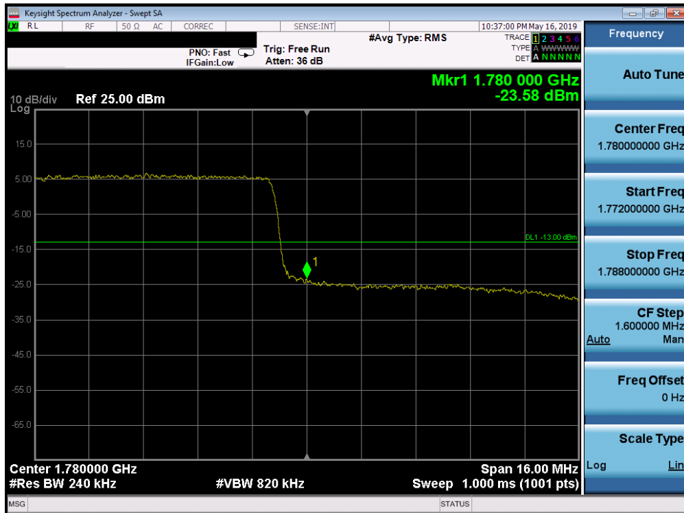
Plot 7-260. Upper Band Edge Plot (Band 66 - 20.0MHz QPSK - Full RB Configuration)
