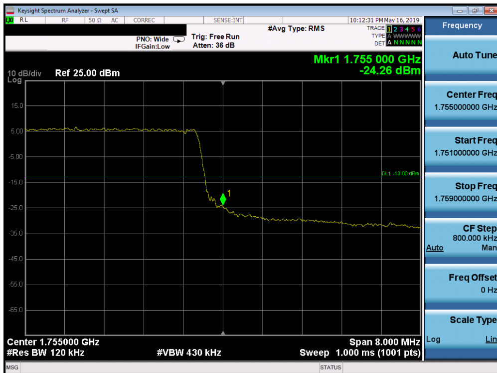
Plot 7-246. Upper Band Edge Plot (Band 4 - 10.0MHz QPSK - Full RB Configuration)
