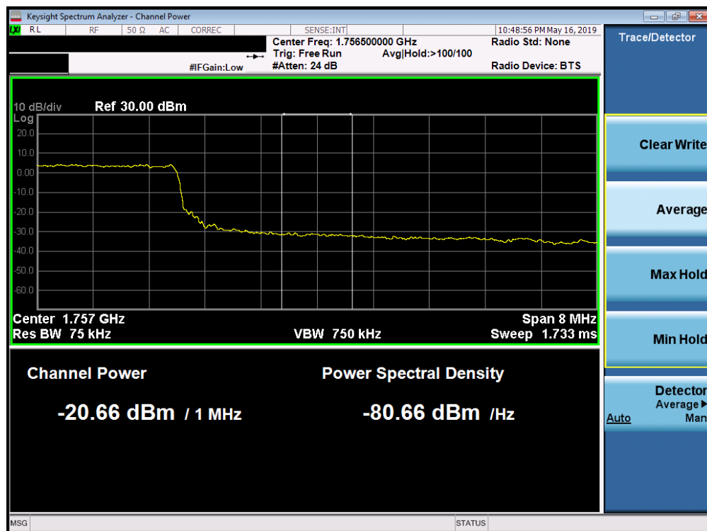
Plot 7-247. Upper Extended Band Edge Plot (Band 4 - 10.0MHz QPSK - Full RB Configuration)
