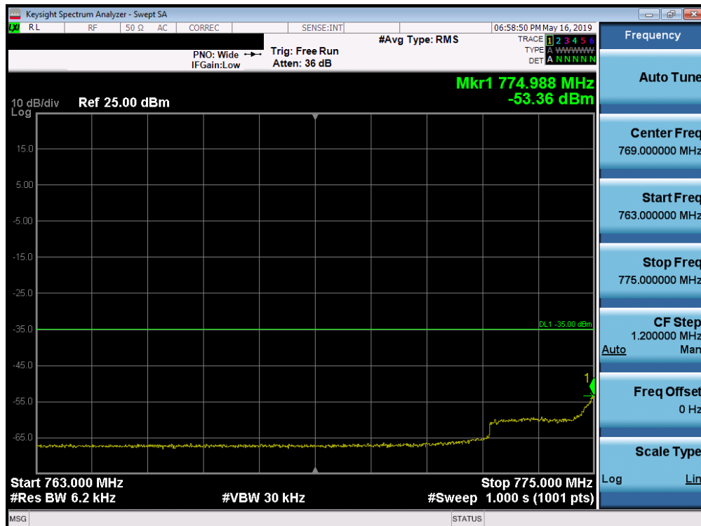
Plot 7-209. Lower Emission Mask Plot (Band 13 - 5.0MHz QPSK - Full RB Configuration)
