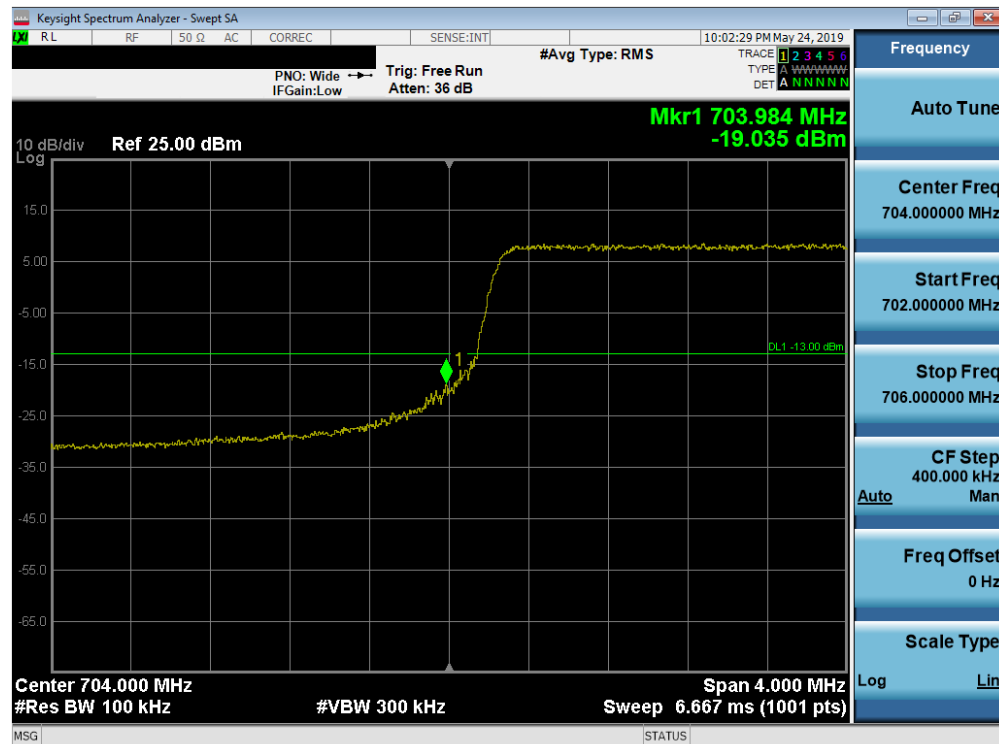
Plot 7-203. Lower Band Edge Plot (Band 17 - 5.0MHz QPSK - Full RB Configuration)
