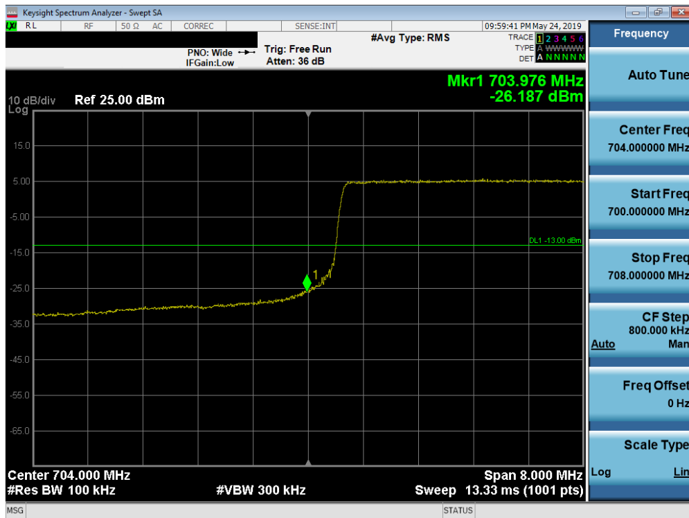
Plot 7-206. Lower Band Edge Plot (Band 17 - 10.0MHz QPSK - Full RB Configuration)
