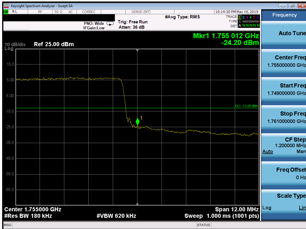
Plot 7-252. Upper Band Edge Plot (Band 4 - 15.0MHz QPSK - Full RB Configuration)
