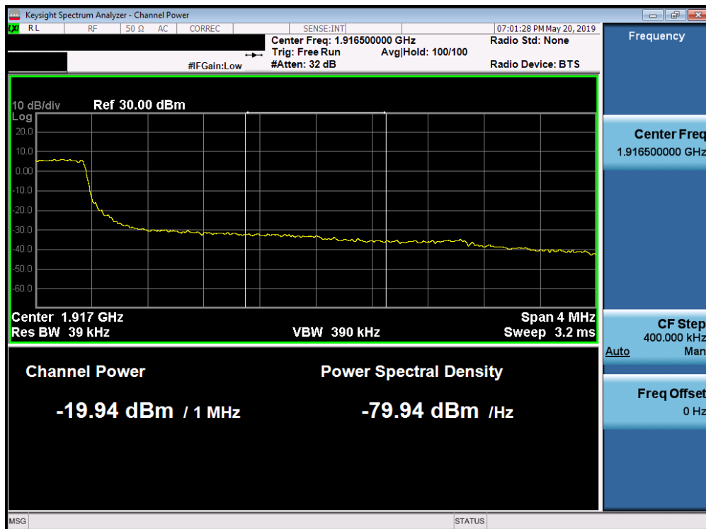
Plot 7-273. Upper Extended Band Edge Plot (Band 25 - 3.0MHz QPSK - Full RB Configuration)
