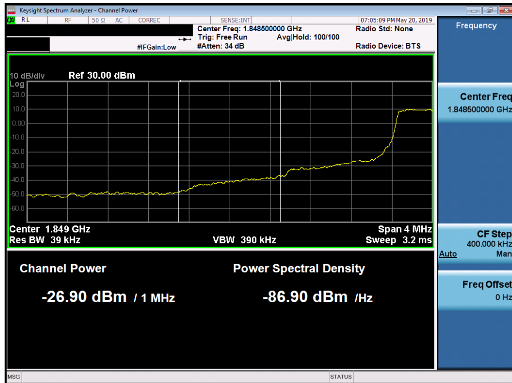
Plot 7-263. Lower Extended Band Edge Plot (Band 25/2 - 1.4MHz QPSK - Full RB Configuration)
