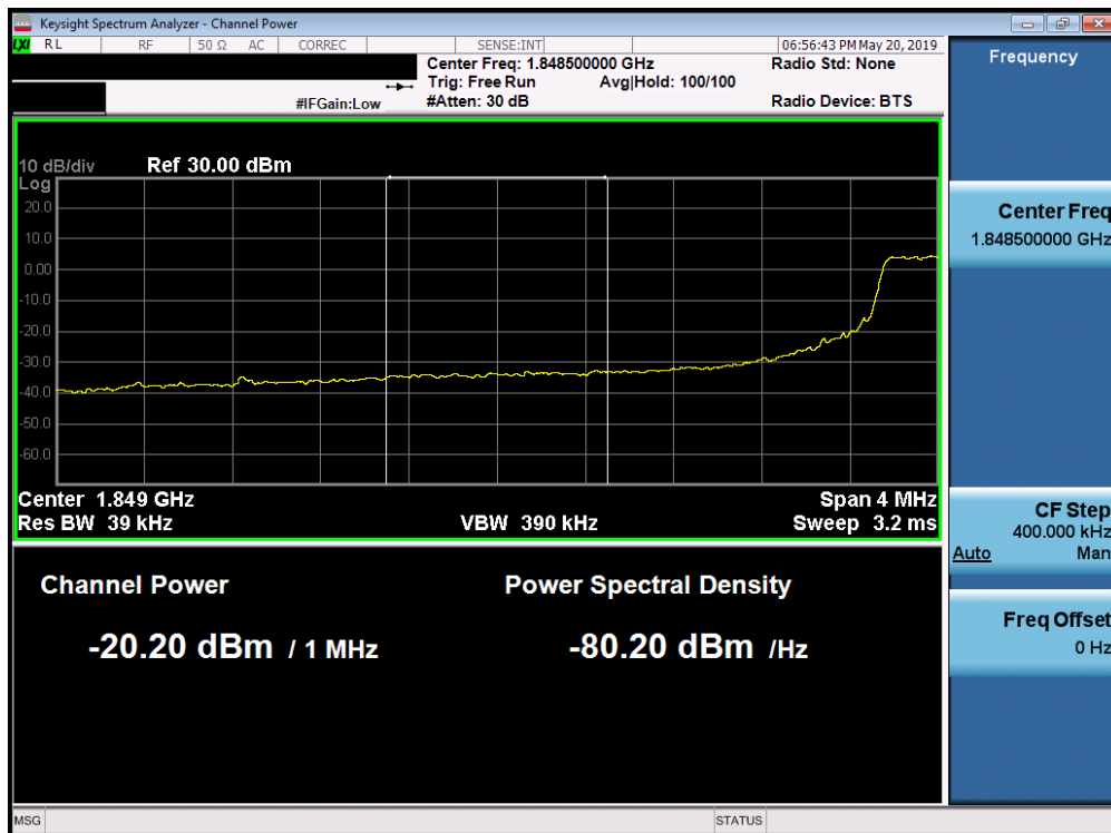
Plot 7-275. Lower Extended Band Edge Plot (Band 25/2 - 5.0MHz QPSK - Full RB Configuration)
