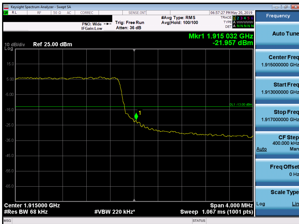
Plot 7-278. Upper Band Edge Plot (Band 25 - 5.0MHz QPSK - Full RB Configuration)
