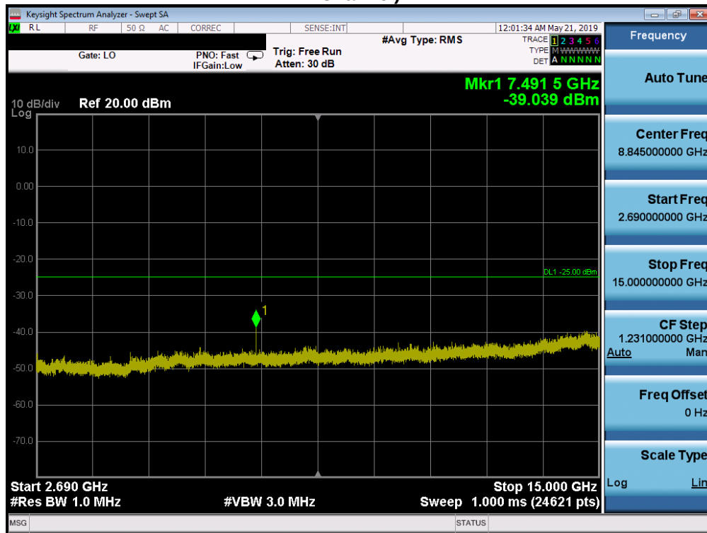
Plot 7-182. Conducted Spurious Plot (Band 41 PC2 - 20.0MHz QPSK - RB Size 1, RB Offset 0 - Low Channel)
