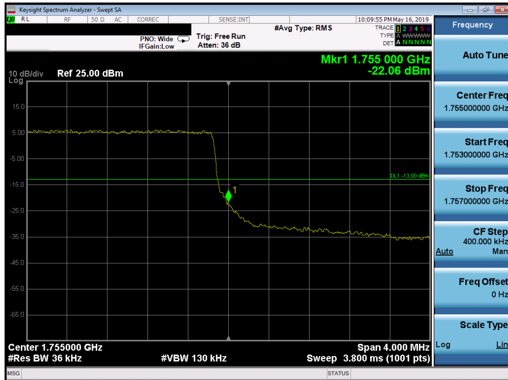
Plot 7-234. Upper Band Edge Plot (Band 4 - 3.0MHz QPSK - Full RB Configuration)
