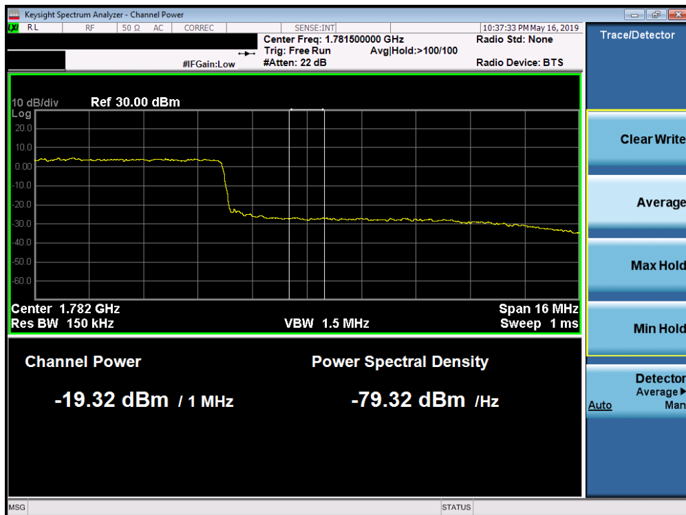
Plot 7-261. Upper Extended Band Edge Plot (Band 66 - 20.0MHz QPSK - Full RB Configuration)
