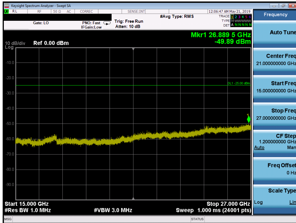
Plot 7-189. Conducted Spurious Plot (Band 41 PC2 - 20.0MHz QPSK - RB Size 1, RB Offset 0 - High Channel)
