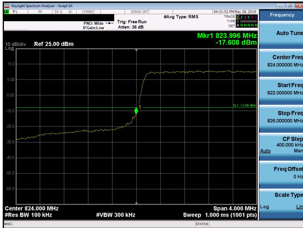
Plot 7-218. Lower Band Edge Plot (Band 26/5 - 3.0MHz QPSK - Full RB Configuration)
