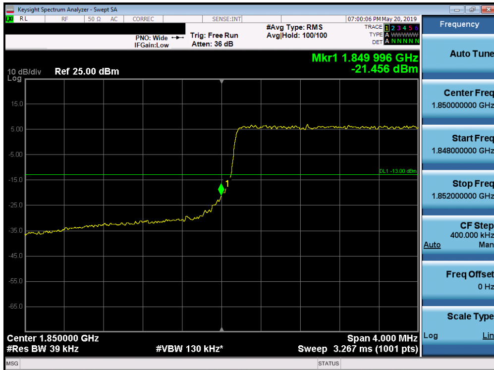
Plot 7-268. Lower Band Edge Plot (Band 25/2 - 3.0MHz QPSK - Full RB Configuration)
