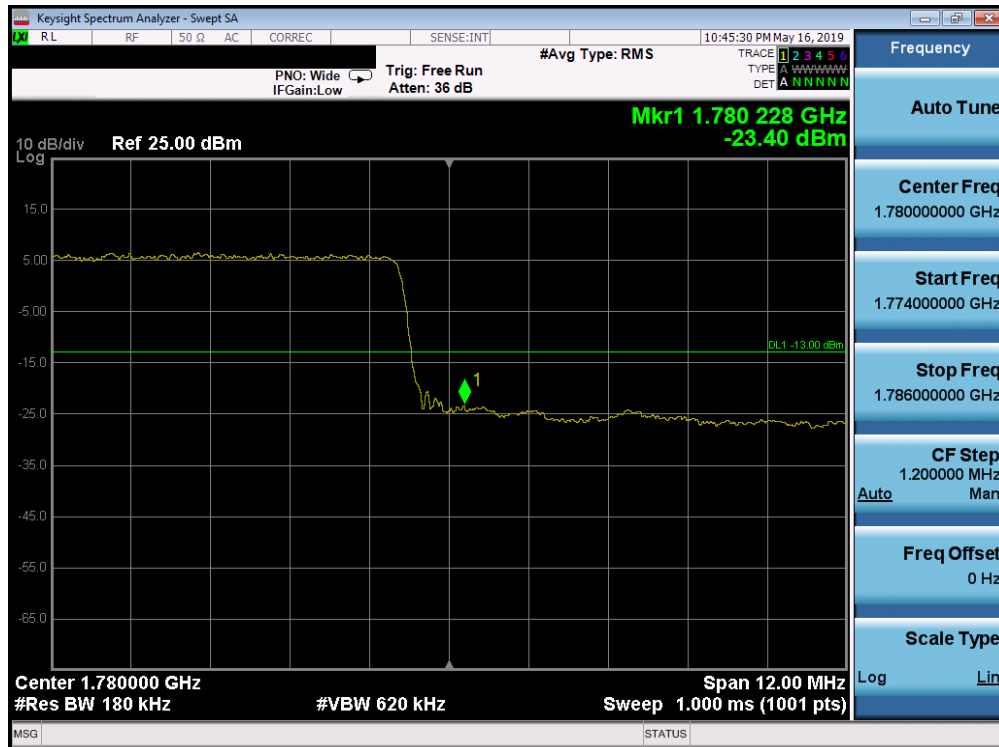
Plot 7-254. Upper Band Edge Plot (Band 66 - 15.0MHz QPSK - Full RB Configuration)
