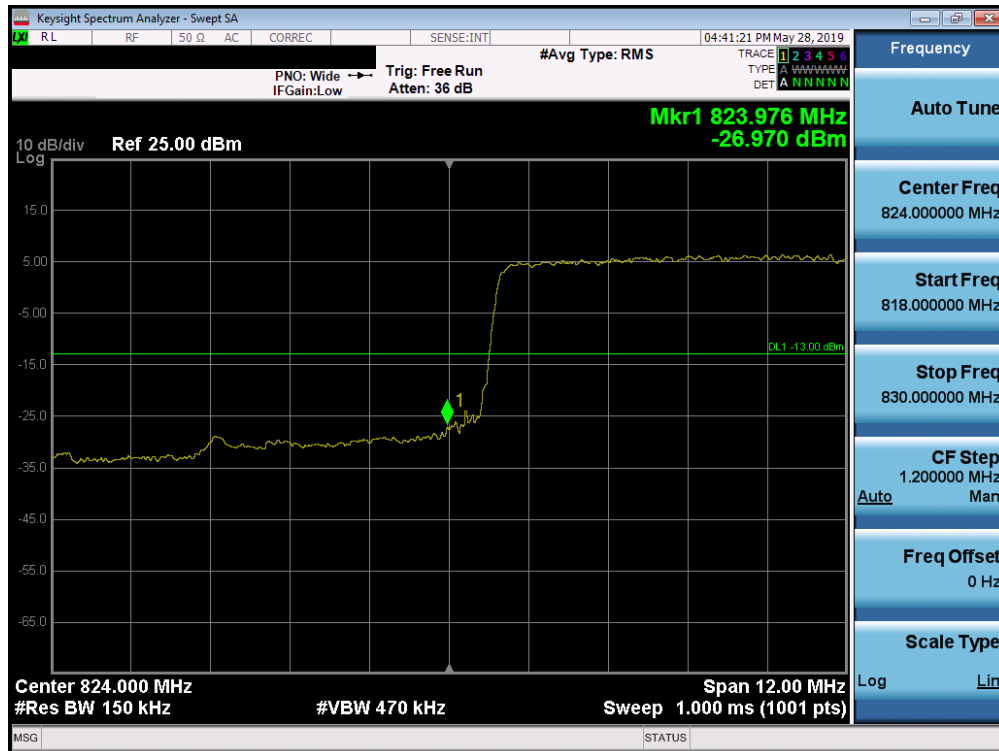
Plot 7-224. Lower Band Edge Plot (Band 26 – 15.0MHz QPSK - Full RB Configuration)
