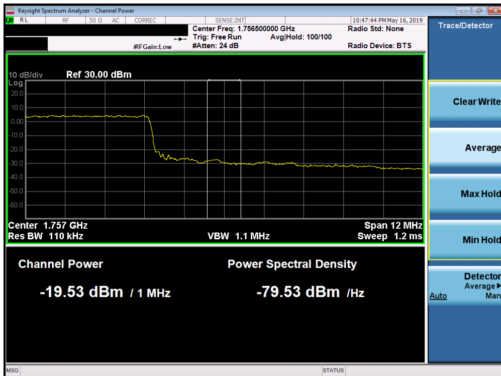
Plot 7-253. Upper Extended Band Edge Plot (Band 4 - 15.0MHz QPSK - Full RB Configuration)
