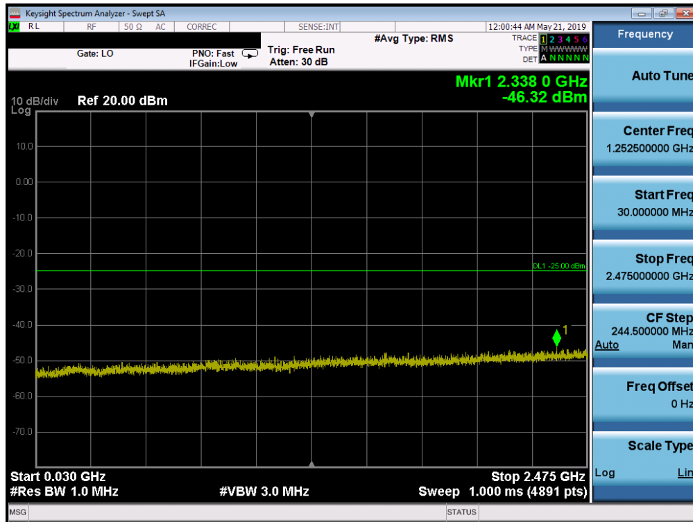
Plot 7-181. Conducted Spurious Plot (Band 41 PC2 - 20.0MHz QPSK - RB Size 1, RB Offset 0 - Low Channel)
