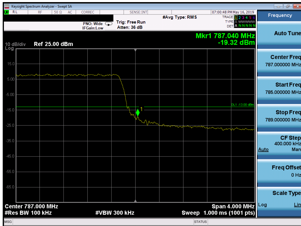
Plot 7-210. Upper Band Edge Plot (Band 13 - 5.0MHz QPSK - Full RB Configuration)
