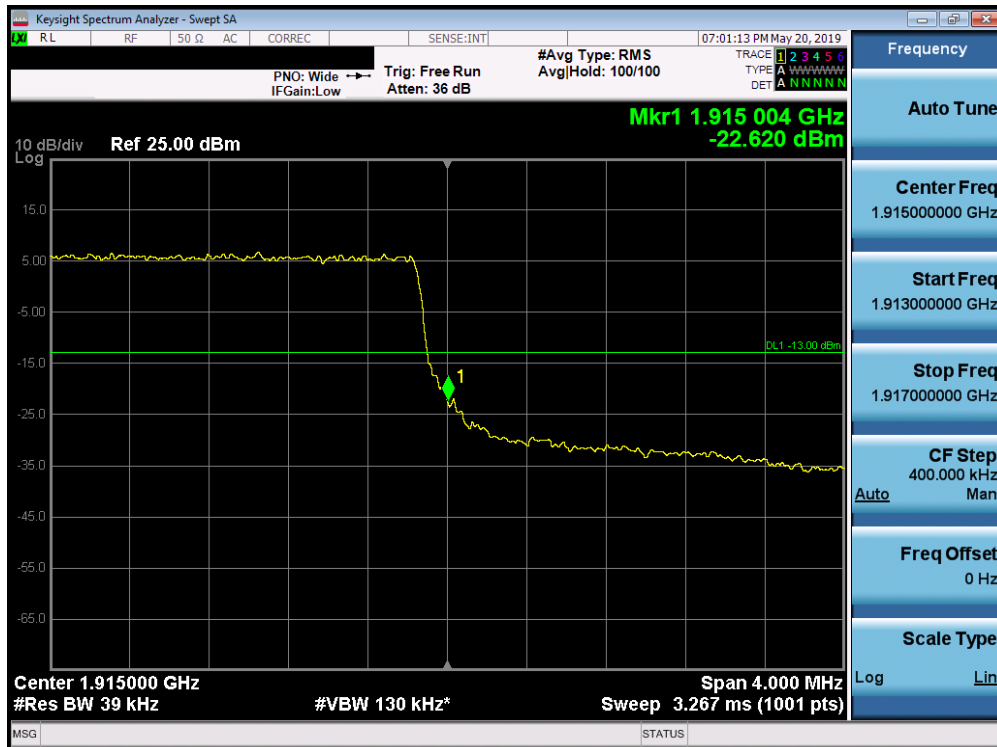
Plot 7-272. Upper Band Edge Plot (Band 25 - 3.0MHz QPSK - Full RB Configuration)
