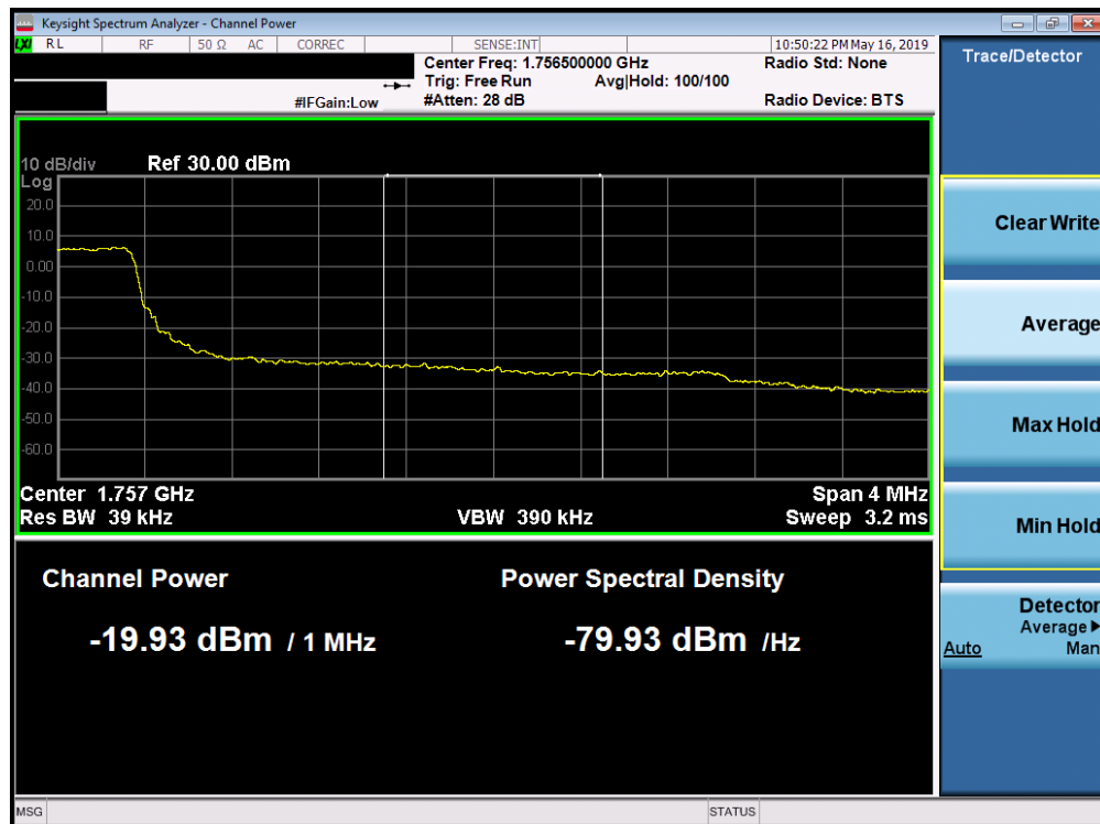
Plot 7-235. Upper Extended Band Edge Plot (Band 4 - 3.0MHz QPSK - Full RB Configuration)
