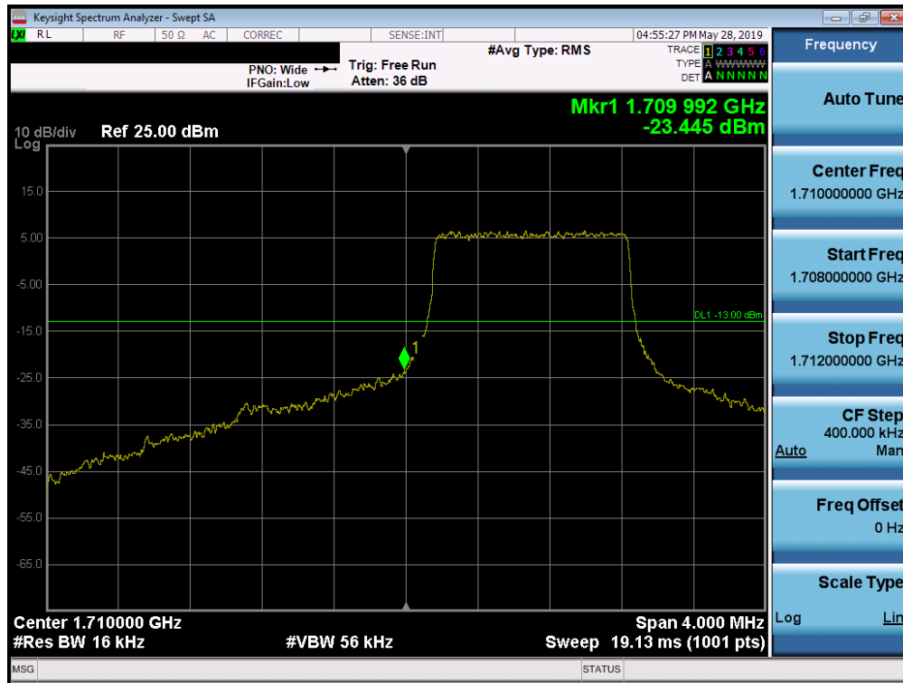
Plot 7-226. Lower Band Edge Plot (Band 66/4 – 1.4MHz QPSK - Full RB Configuration)
