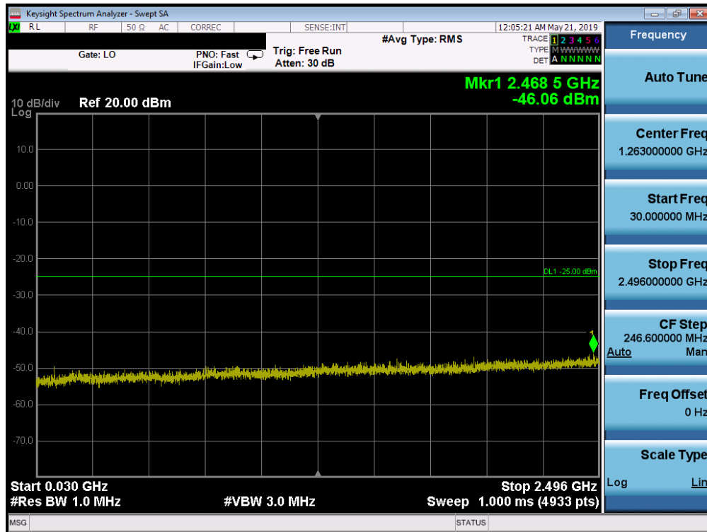
Plot 7-187. Conducted Spurious Plot (Band 41 PC2 - 20.0MHz QPSK - RB Size 1, RB Offset 0 - High Channel)
