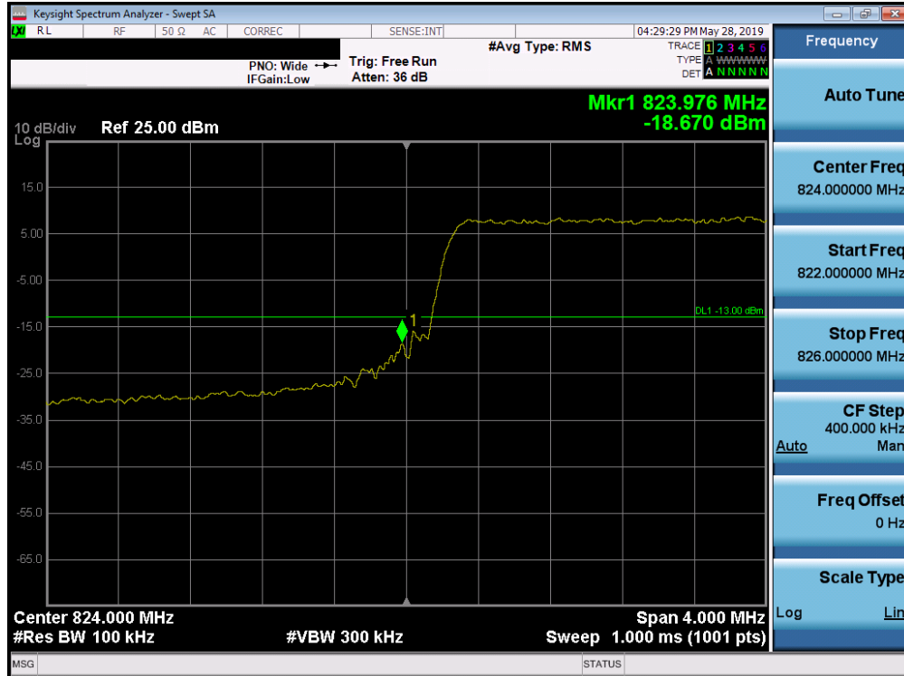
Plot 7-222. Lower Band Edge Plot (Band 26/5 – 10.0MHz QPSK - Full RB Configuration)
