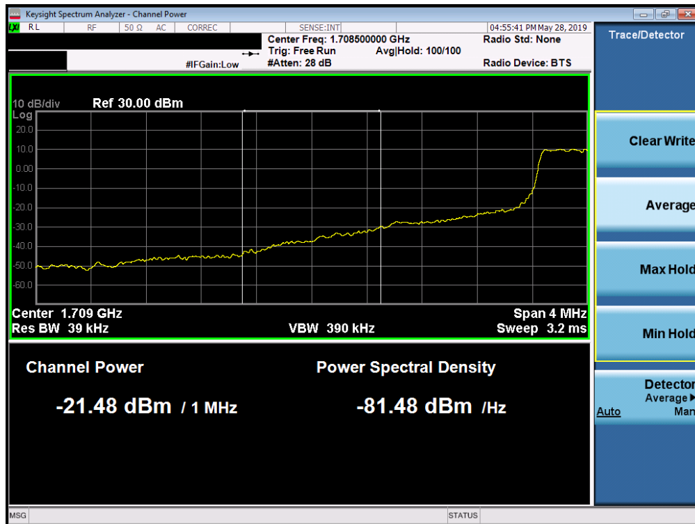
Plot 7-227. Lower Extended Band Edge Plot (Band 66/4 – 1.4MHz QPSK - Full RB Configuration)
