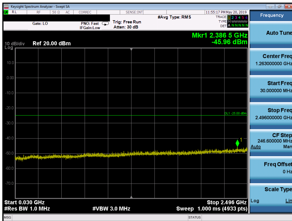
Plot 7-184. Conducted Spurious Plot (Band 41 PC2 - 20.0MHz QPSK - RB Size 1, RB Offset 0 - Mid Channel)
