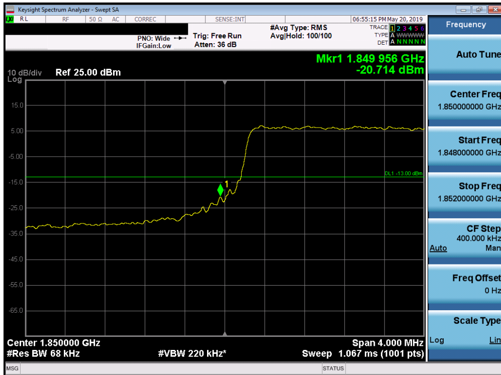
Plot 7-274. Lower Band Edge Plot (Band 25/2 - 5.0MHz QPSK - Full RB Configuration)
