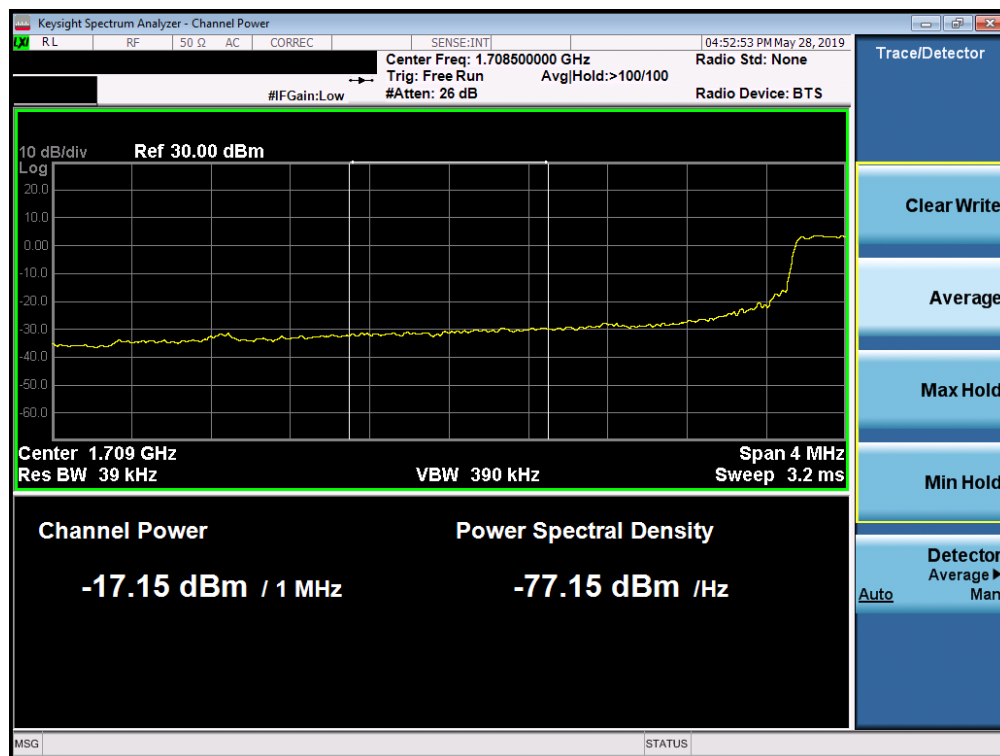
Plot 7-239. Lower Extended Band Edge Plot (Band 66/4 - 5.0MHz QPSK - Full RB Configuration)
