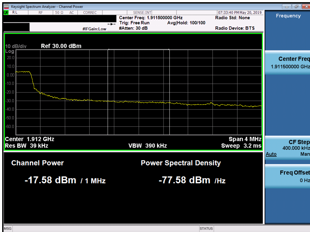
Plot 7-277. Upper Extended Band Edge Plot (Band 2 - 5.0MHz QPSK - Full RB Configuration)
