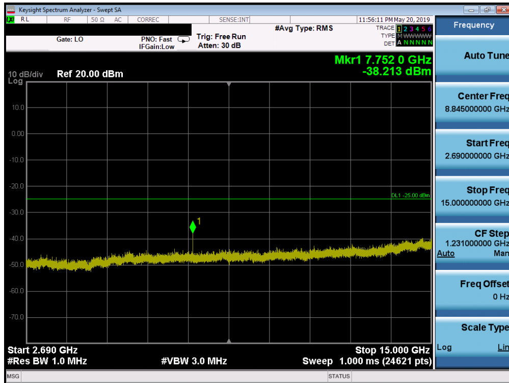
Plot 7-185. Conducted Spurious Plot (Band 41 PC2 - 20.0MHz QPSK - RB Size 1, RB Offset 0 - Mid Channel)
