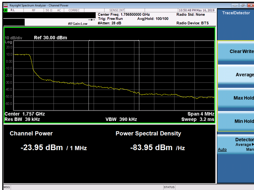
Plot 7-229. Upper Extended Band Edge Plot (Band 4 - 1.4MHz QPSK - Full RB Configuration)
