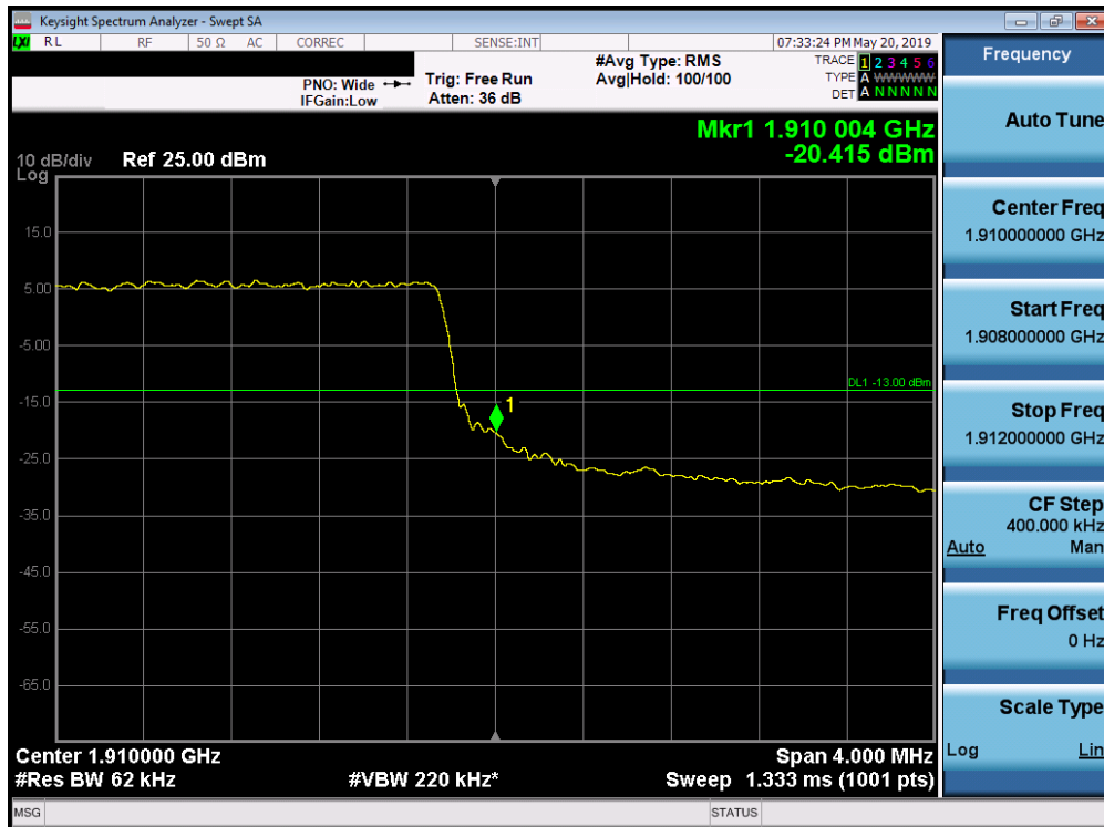
Plot 7-276. Upper Band Edge Plot (Band 2 - 5.0MHz QPSK - Full RB Configuration)
