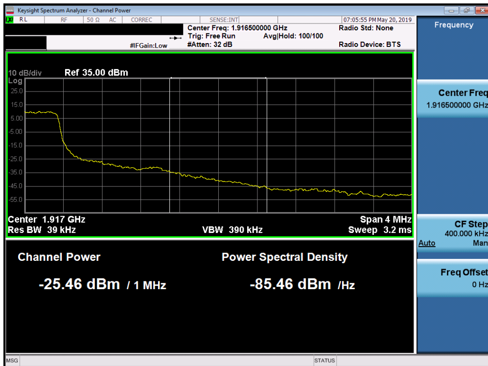
Plot 7-267. Upper Extended Band Edge Plot (Band 25 - 1.4MHz QPSK - Full RB Configuration)
