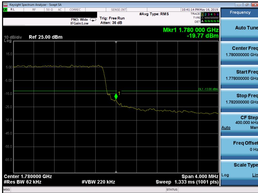
Plot 7-242. Upper Band Edge Plot (Band 66 - 5.0MHz QPSK - Full RB Configuration)
