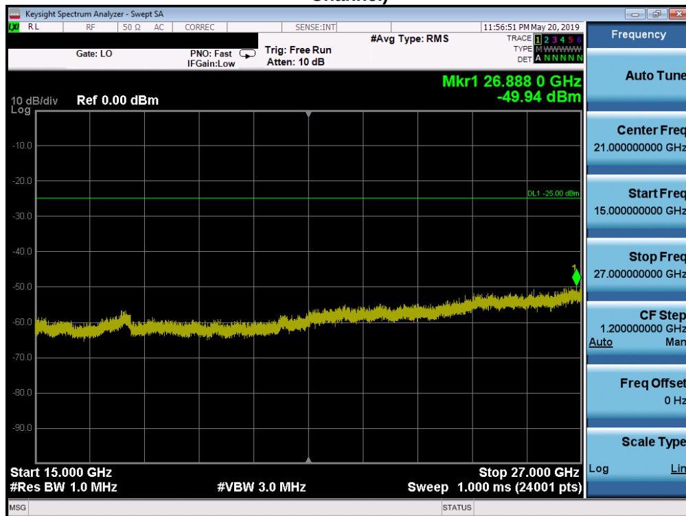
Plot 7-186. Conducted Spurious Plot (Band 41 PC2 - 20.0MHz QPSK - RB Size 1, RB Offset 0 - Mid Channel)
