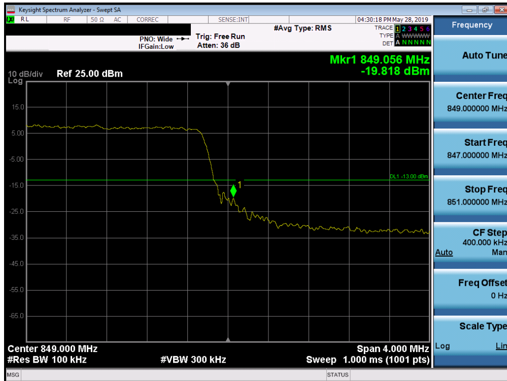
Plot 7-223. Upper Band Edge Plot (Band 26/5 - 10.0MHz QPSK - Full RB Configuration)
