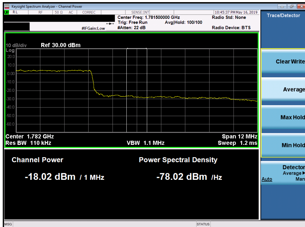
Plot 7-255. Upper Extended Band Edge Plot (Band 66 - 15.0MHz QPSK - Full RB Configuration)
