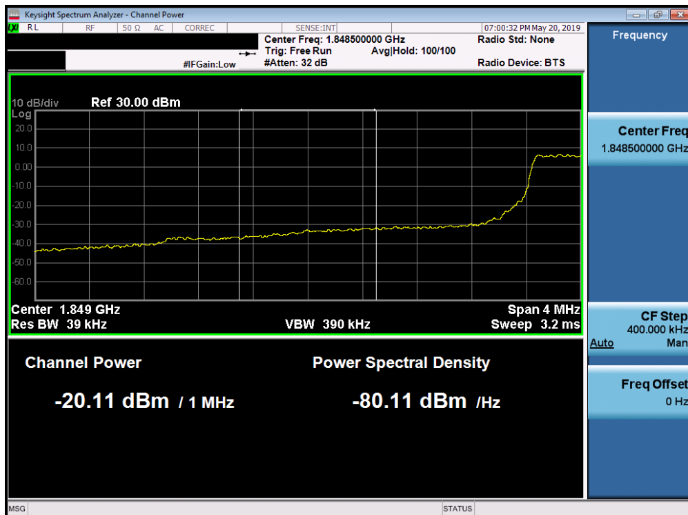
Plot 7-269. Lower Extended Band Edge Plot (Band 25/2 - 3.0MHz QPSK - Full RB Configuration)
