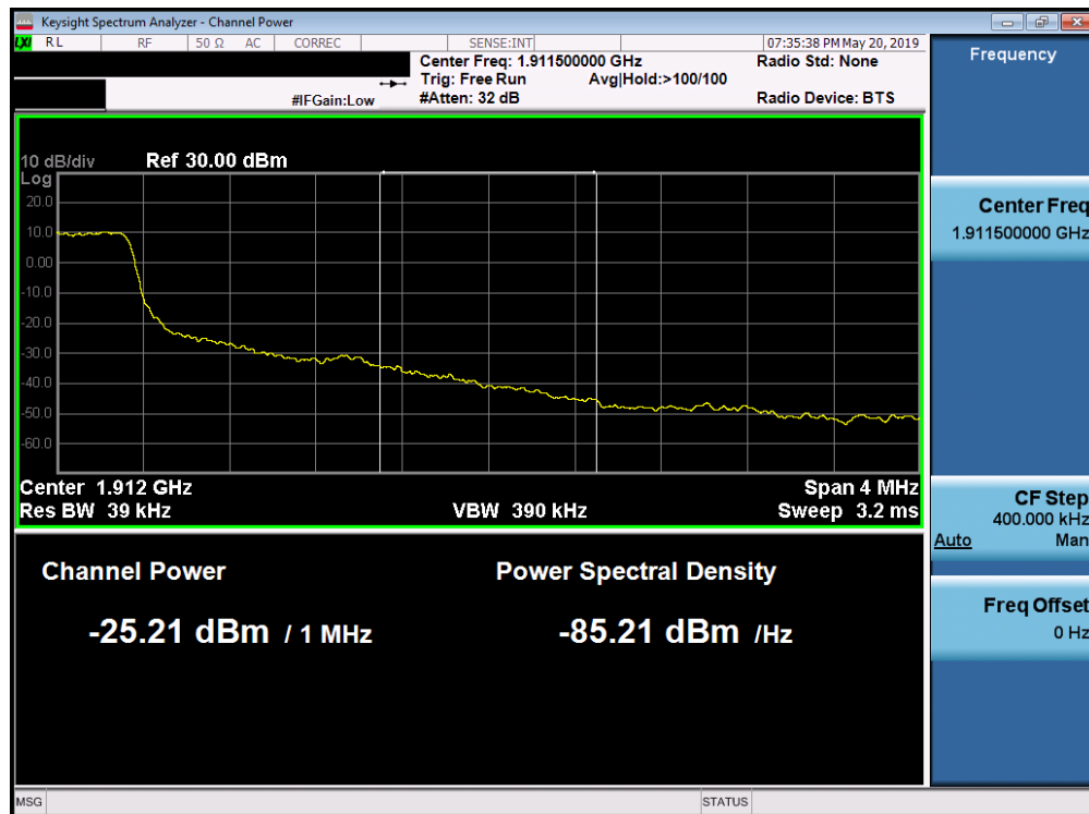
Plot 7-265. Upper Extended Band Edge Plot (Band 2 - 1.4MHz QPSK - Full RB Configuration)
