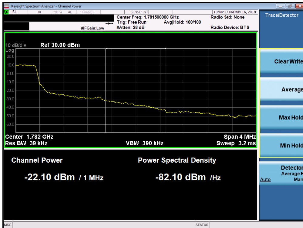
Plot 7-231. Upper Extended Band Edge Plot (Band 66 - 1.4MHz QPSK - Full RB Configuration)
