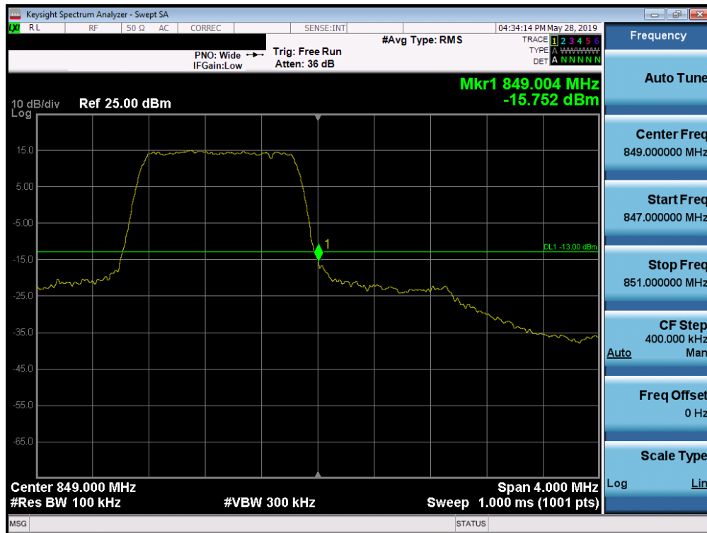
Plot 7-217. Upper Band Edge Plot (Band 26/5 - 1.4MHz QPSK - Full RB Configuration)
