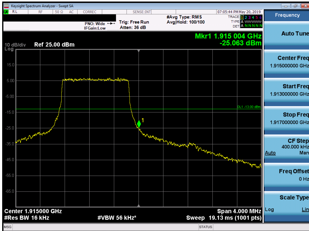
Plot 7-266. Upper Band Edge Plot (Band 25 - 1.4MHz QPSK - Full RB Configuration)
