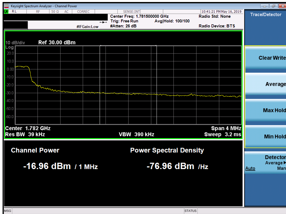
Plot 7-243. Upper Extended Band Edge Plot (Band 66 - 5.0MHz QPSK - Full RB Configuration)
