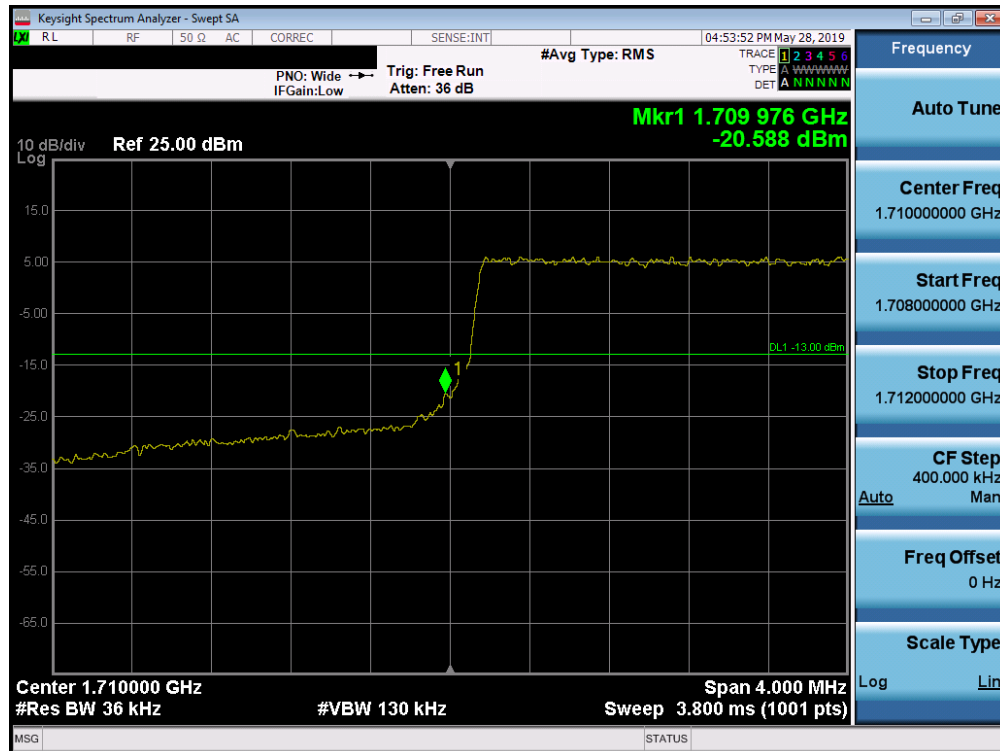
Plot 7-232. Lower Band Edge Plot (Band 66/4 - 3.0MHz QPSK - Full RB Configuration)
