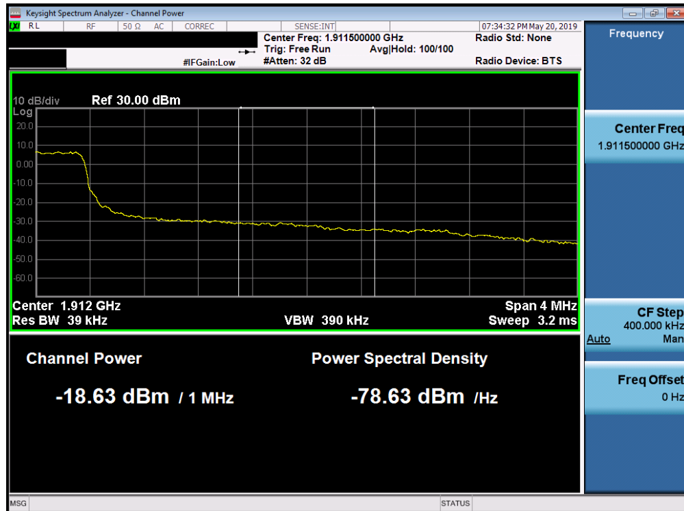
Plot 7-271. Upper Extended Band Edge Plot (Band 2 - 3.0MHz QPSK - Full RB Configuration)
