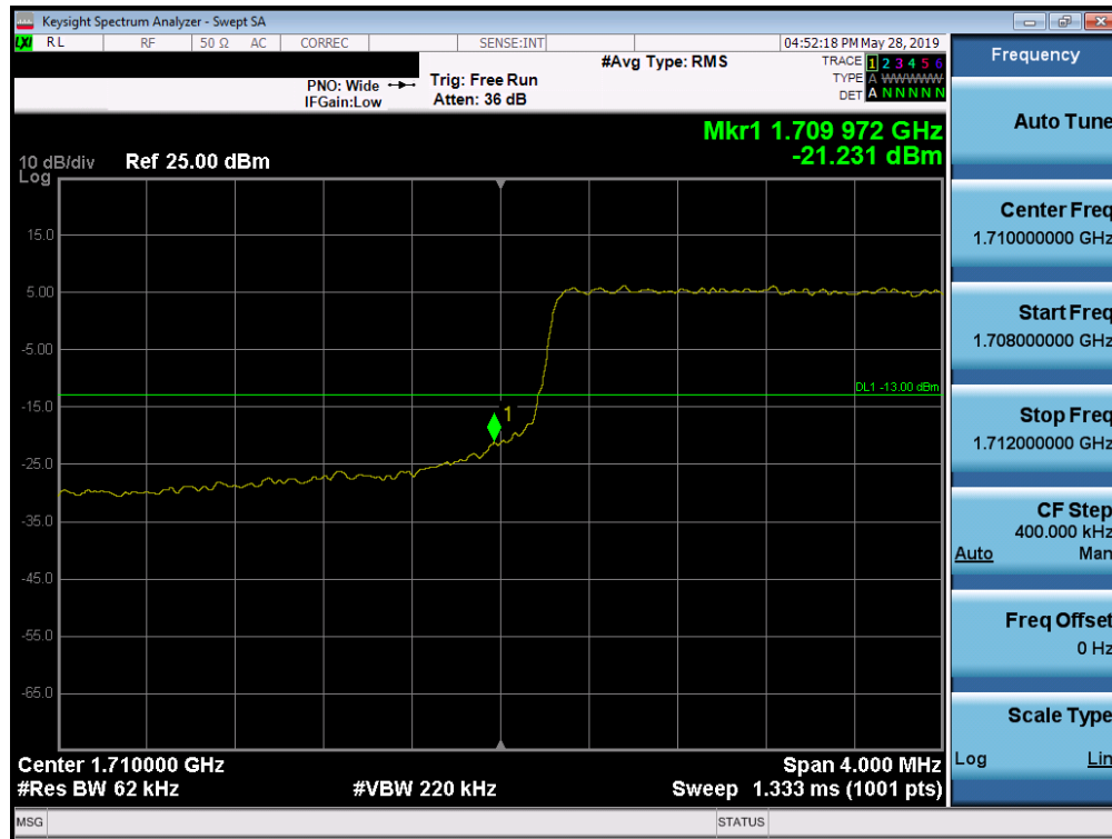
Plot 7-238. Lower Band Edge Plot (Band 66/4 - 5.0MHz QPSK - Full RB Configuration)
