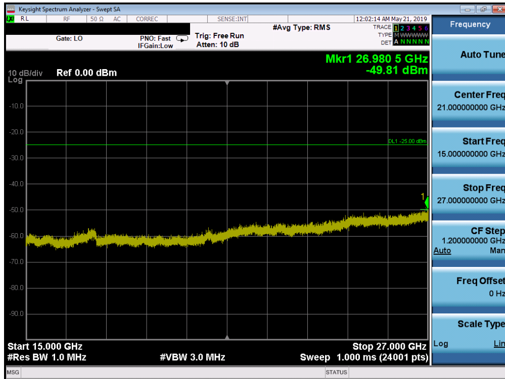
Plot 7-183. Conducted Spurious Plot (Band 41 PC2 - 20.0MHz QPSK - RB Size 1, RB Offset 0 - Low Channel)
