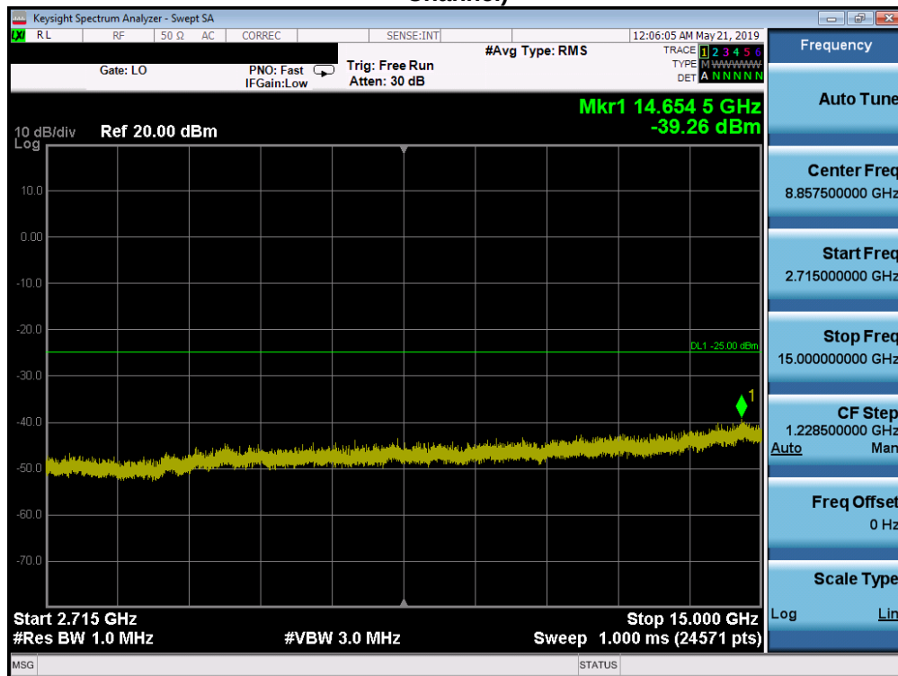
Plot 7-188. Conducted Spurious Plot (Band 41 PC2 - 20.0MHz QPSK - RB Size 1, RB Offset 0 - High Channel)
