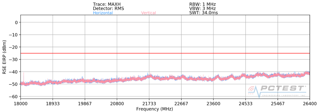
Plot 7-373. Radiated Spurious Plot 18GHz - 26.5GHz (Band 41 PC2)
