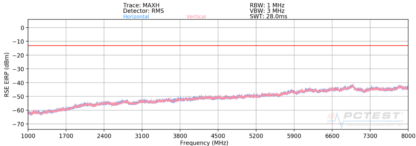
Plot 7-367. Radiated Spurious Plot above 1GHz (Band 12/17)
