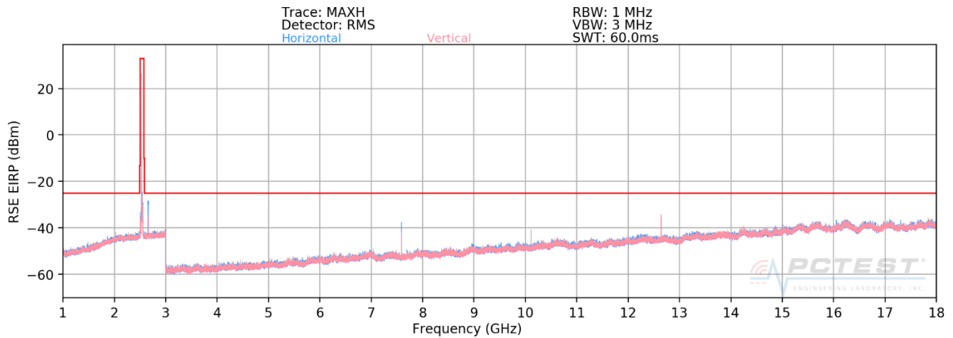
Plot 7-370. Radiated Spurious Plot 1GHz - 18GHz (Band 7)
