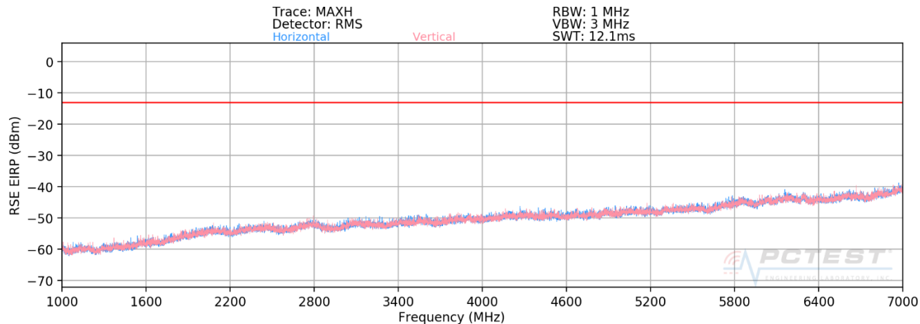
Plot 7-366. Radiated Spurious Plot above 1GHz (Band 71)
