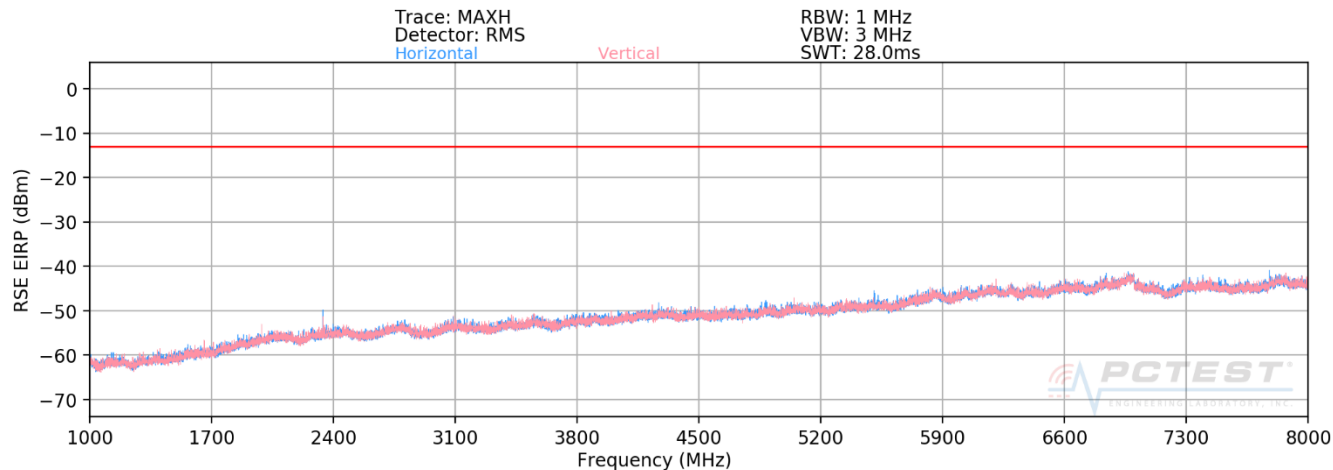
Plot 7-368. Radiated Spurious Plot above 1GHz (Band 13)
