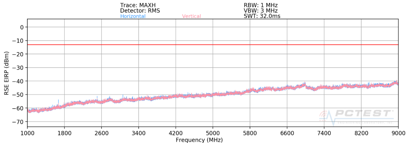
Plot 7-369. Radiated Spurious Plot above 1GHz (Band 26/5)
