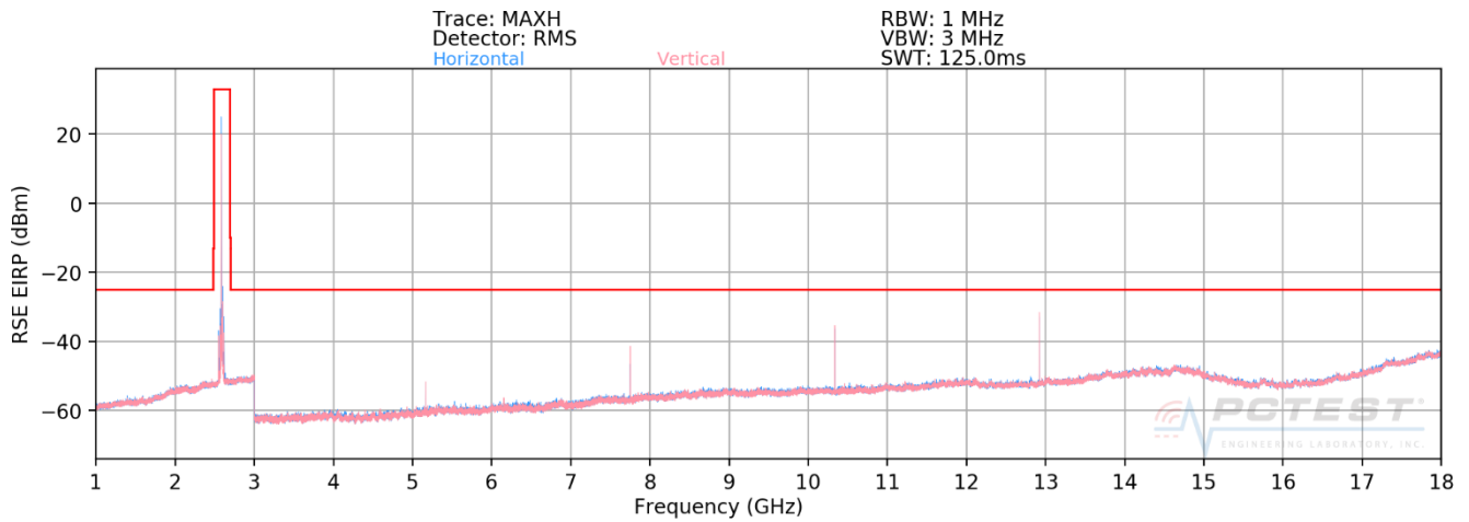
Plot 7-372. Radiated Spurious Plot 1GHz - 18GHz (Band 41 PC2)
