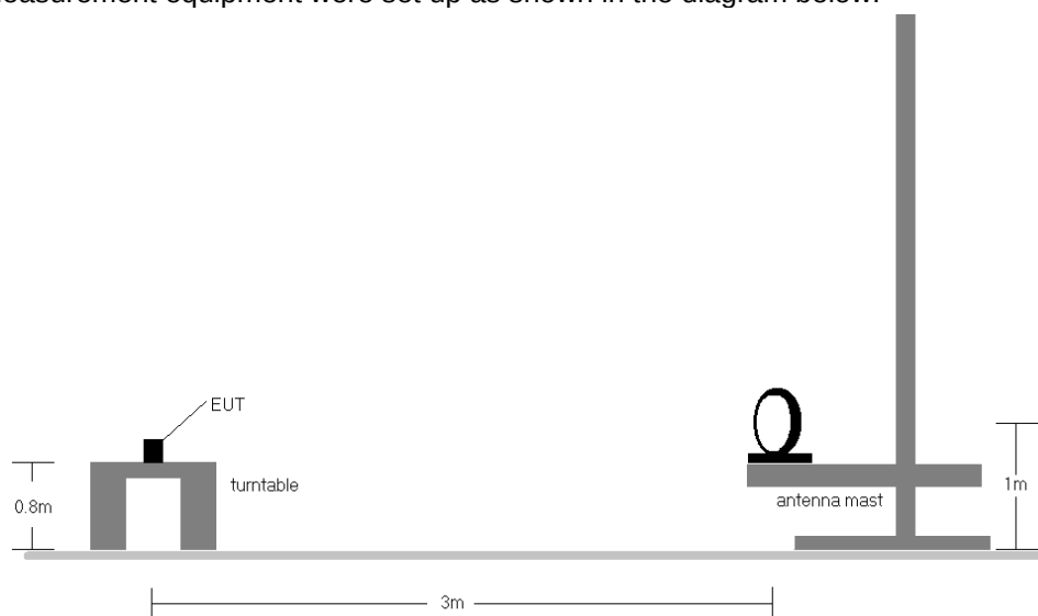
Figure 7-3. Radiated Test Setup
