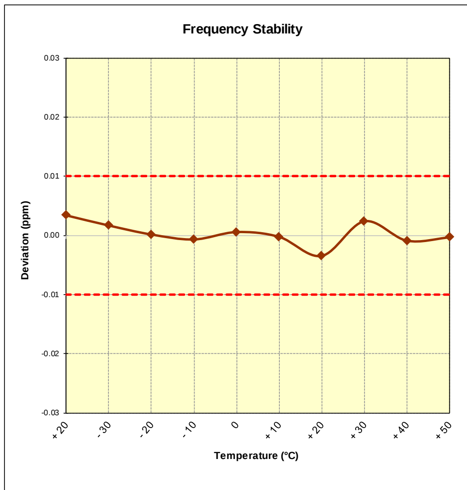
Figure 7-2. Frequency Stability Plot
