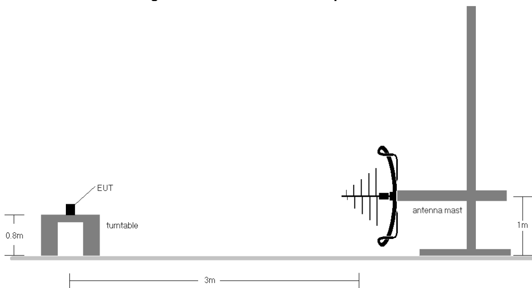
Figure 7-5. Radiated Test Setup > 30MHz
