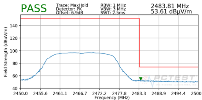
Plot 7-46. Radiated Restricted Upper Band Edge Measurement (Peak)
