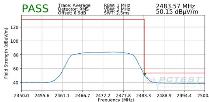
Plot 7-47. Radiated Restricted Upper Band Edge Measurement (Average)
