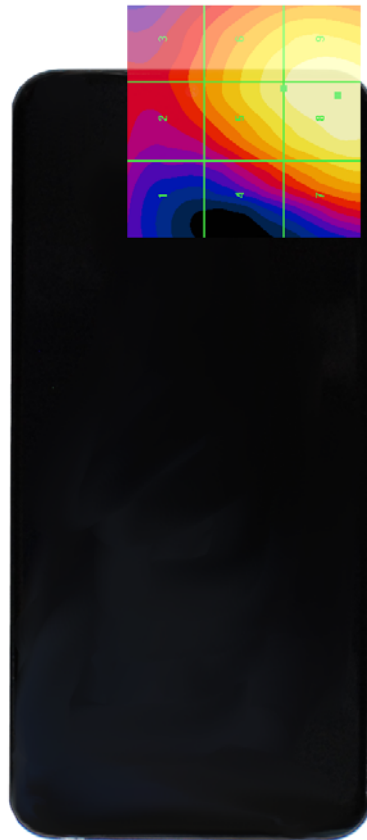
Figure 18-4 E-Field WD Scan overlay (T-Coil Centered scan area pictured)
