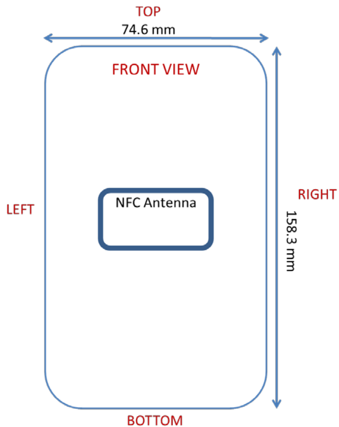
Figure F-2 NFC Antenna Location
