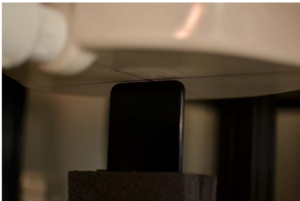
SAR Test Setup Photo 14: Bottom Edge at 0.2 cm
