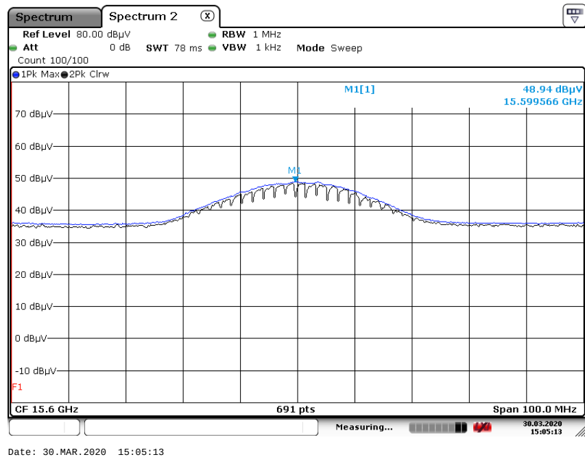
Peak Reading (802.11a, Ch.40 3rd Harmonic, Z-H)
