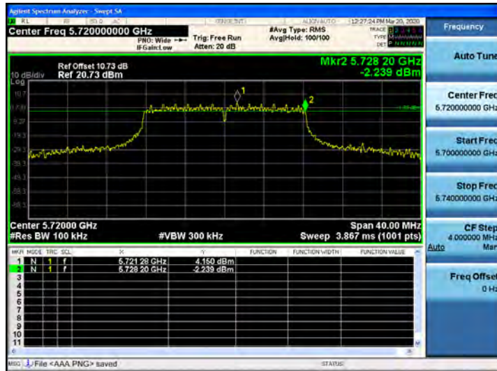
802.11ac_VHT20 CH.144
