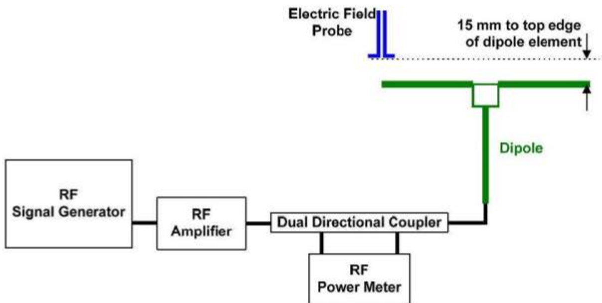
Setup diagram
