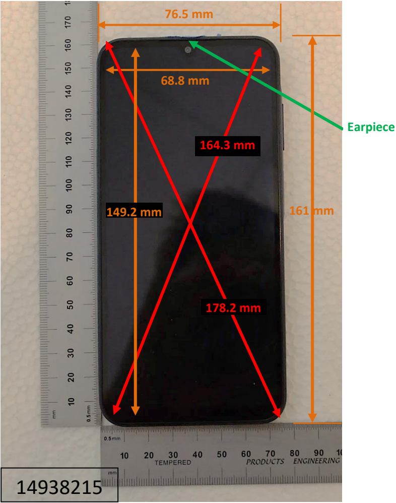
Photograph 1: Overall Dimensions
