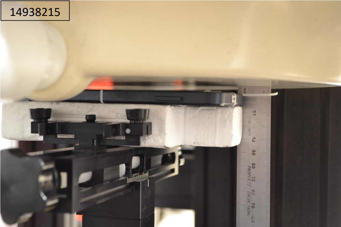
Photograph 22: Extremity, Back, 6 mm
