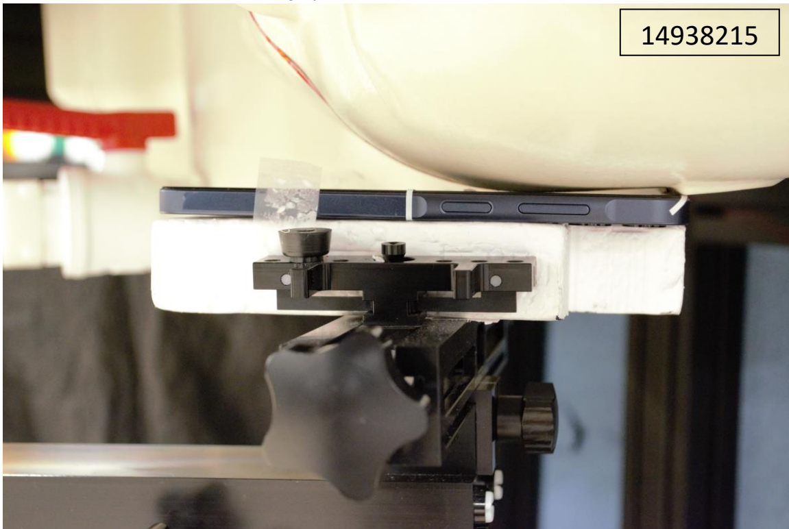
Photograph 5: Head, Left Cheek, 0 mm
