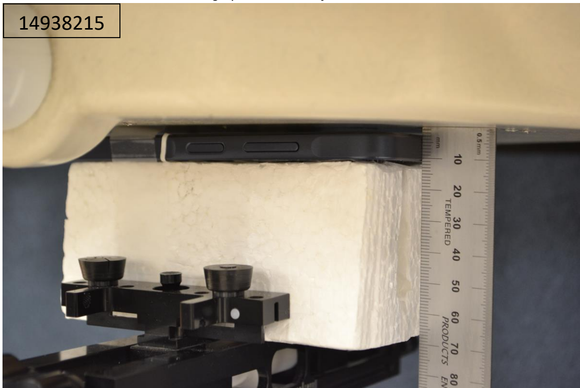
Photograph 23: Extremity, Front, 2 mm
