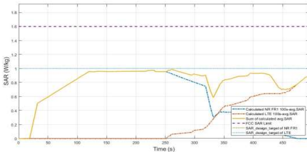
Figure 7.6-4 Total time-averaged SAR in TC07
