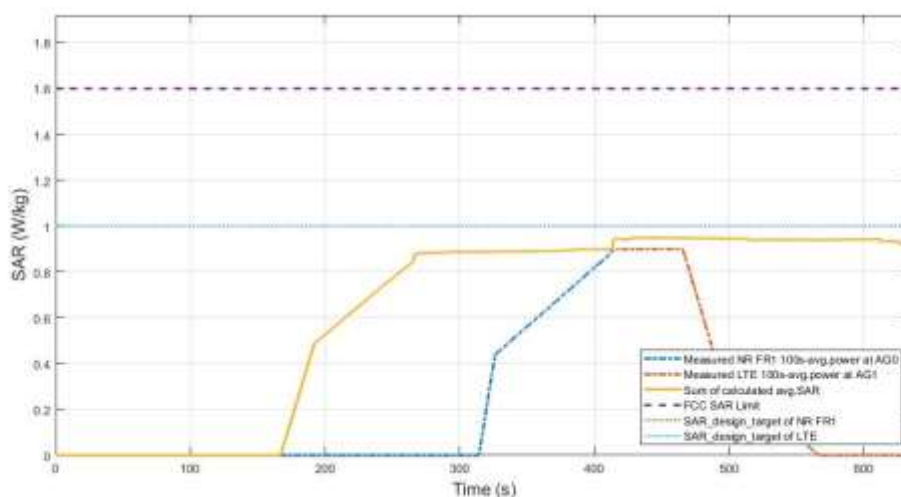
Figure 7.12-4 Total time-averaged SAR in TC13
