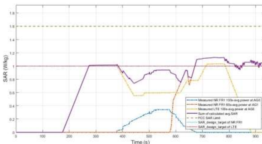
Figure 7.13-2 Total time-averaged SAR in TC14
