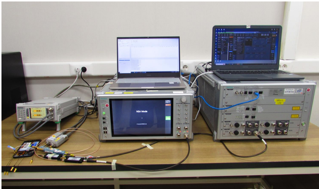
Test setup photo-5(TC 13-2)
