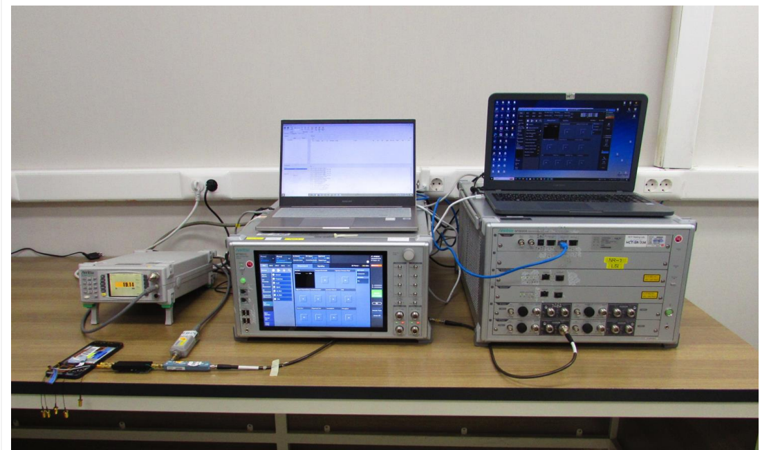
Test setup photo-4(TC 12-2)
