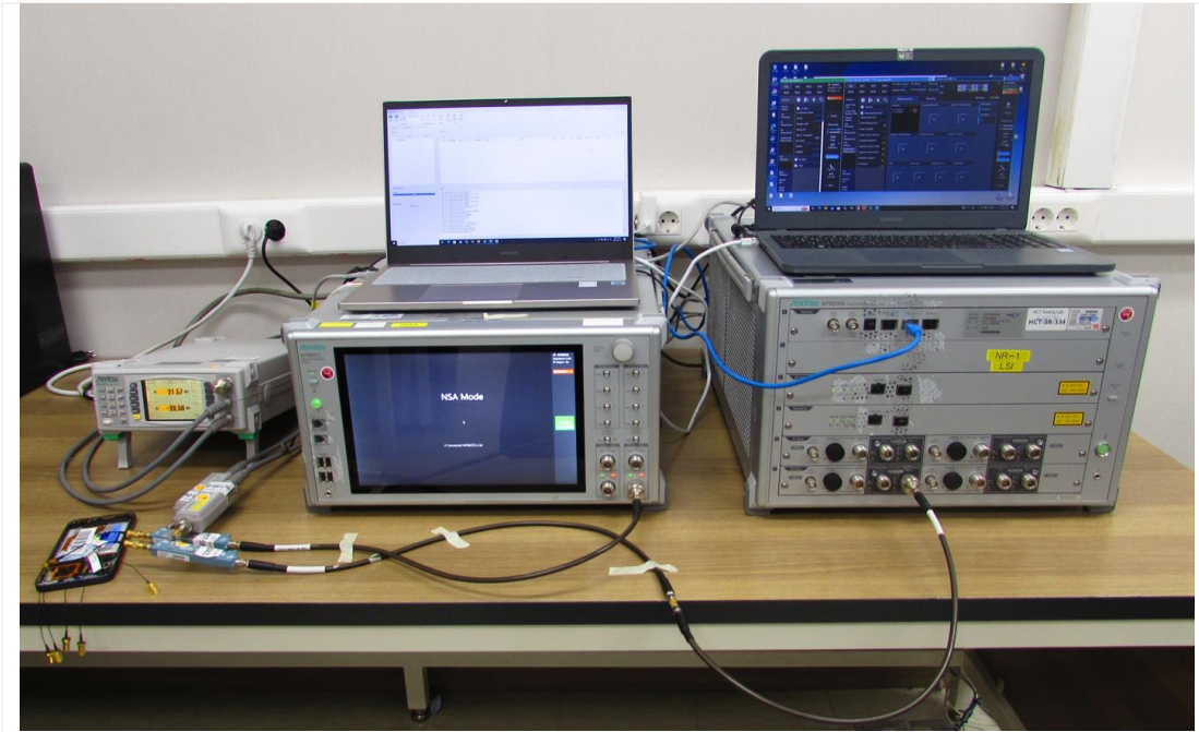
Test setup photo-3(TC 7-2)
