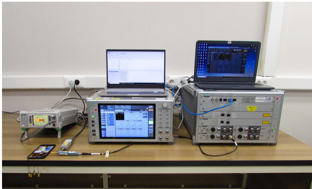
Test setup photo-1(TC 2-2, 4-2)
