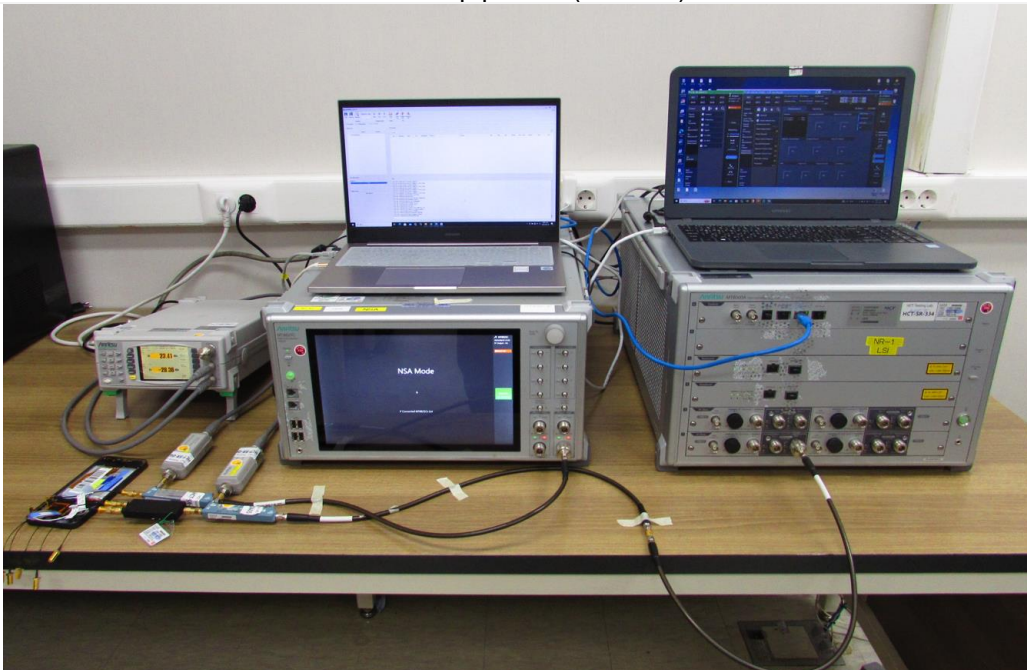
Test setup photo-6(TC 14)
