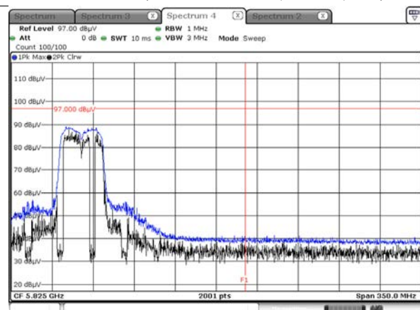
Peak Result (802.11ac_VHT40, Ch.142, Z-H)
