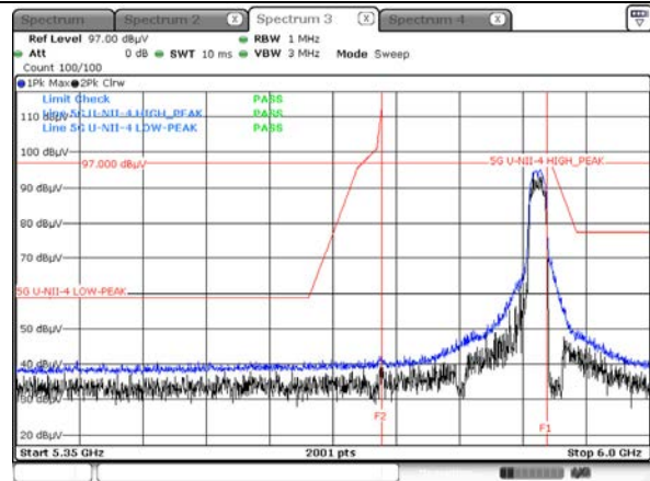
Peak Result (802.11n_HT40, Ch.175, Z-H)
