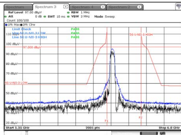
Peak Result (802.11ac_VHT20, Ch.149, X-H)
