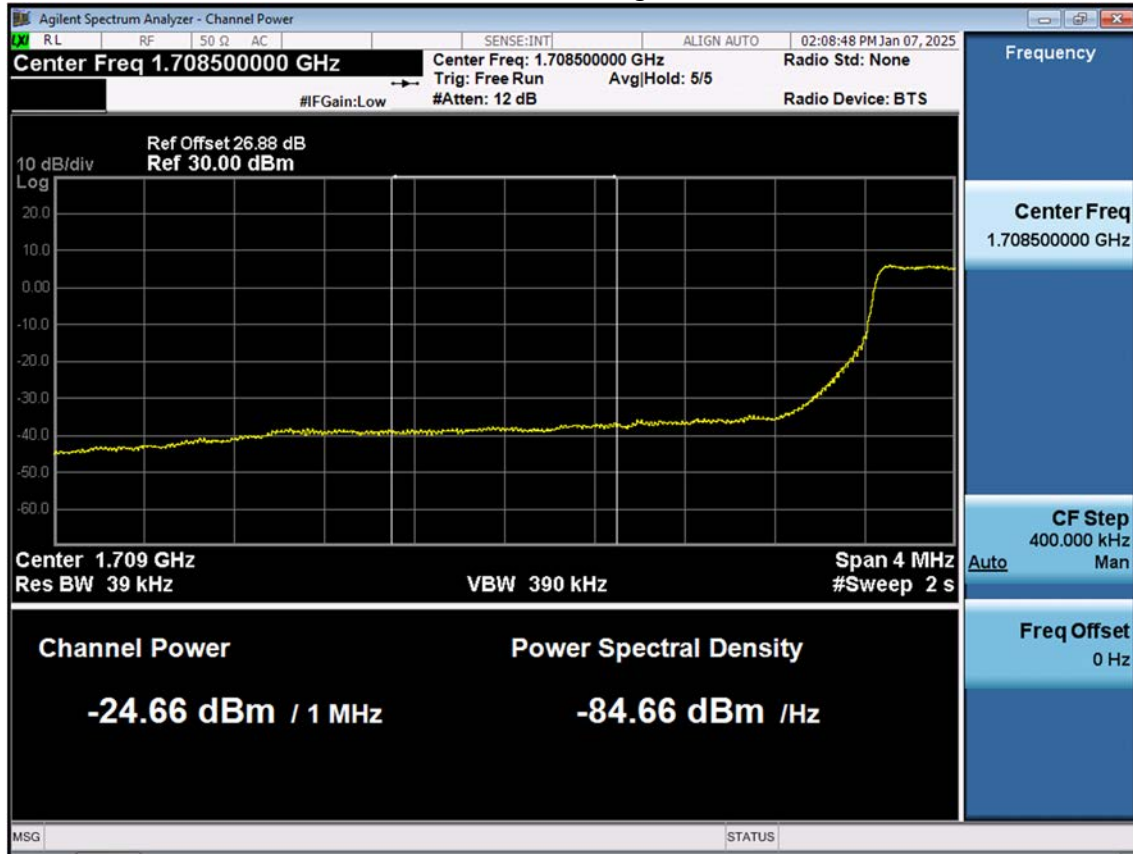
LTE B66_3 M_Extended Band Edge_Low_QPSK_FullIRB
