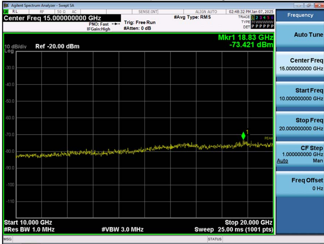
LTE B66_20 M_Conducted Spurious(Above10 G)_High_QPSK_1RB
