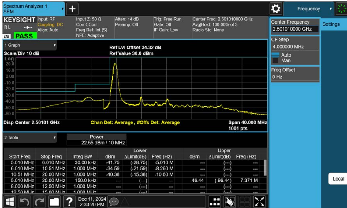
NR41_10 M_Band Edge_Lower_Low_BPSK_1RB
