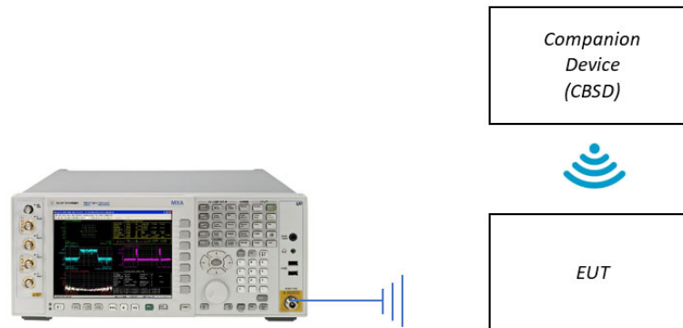
Test setup
