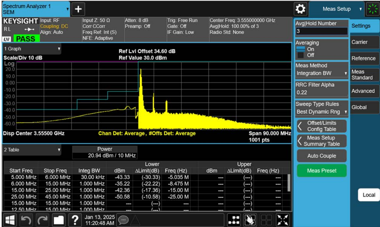
Sub6 n48. 10 M_BandEdge(Lower)_Low_ 3555.00 MHz_BPSK_1RB
