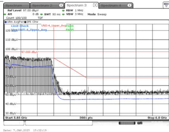
Average Result (802.11ac_VHT80, Ch.171, Y-H)
