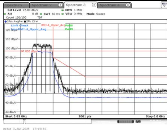
Average Result (802.11n_HT40, Ch.175, Y-H)
