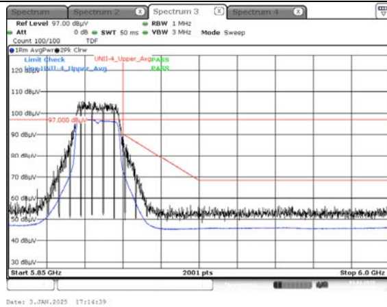
Average Result (802.11ac_VHT20, Ch.177, Y-H)
