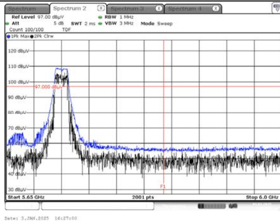
Peak Result (802.11ac_VHT20, Ch.144, Y-H)
