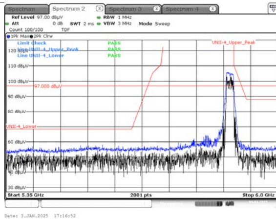
Peak Result (802.11ac_VHT40, Ch.175, Y-H)
