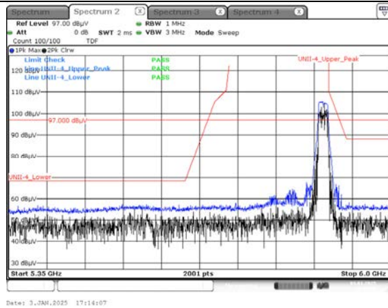
Peak Result (802.11ac_VHT20, Ch.177, Y-H)
