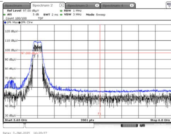
Peak Result (802.11ac_VHT40, Ch.142, Y-H)
