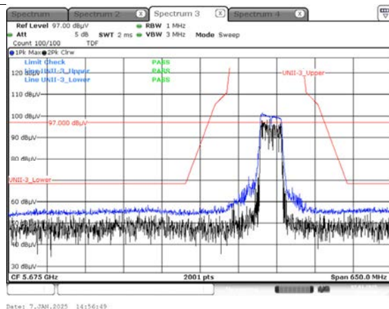
Peak Result (802.11ac_VHT40, Ch.159, Y-H)
