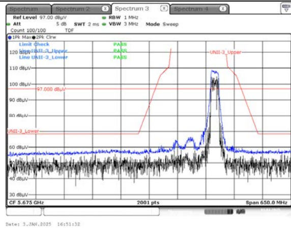
Peak Result (802.11n_HT40, Ch.159, Y-H)
