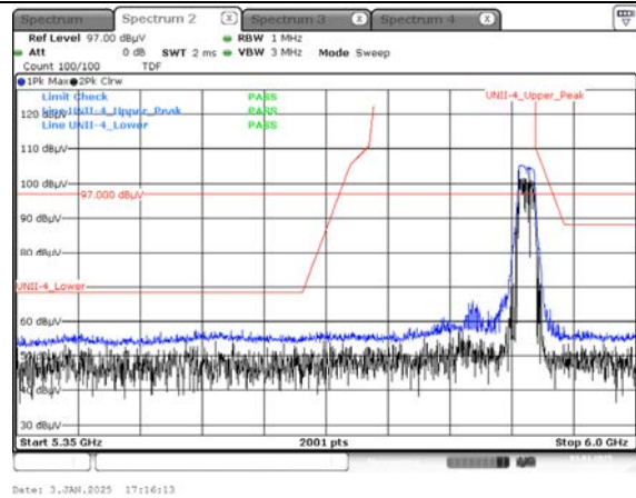
Peak Result (802.11n_HT40, Ch.175, Y-H)
