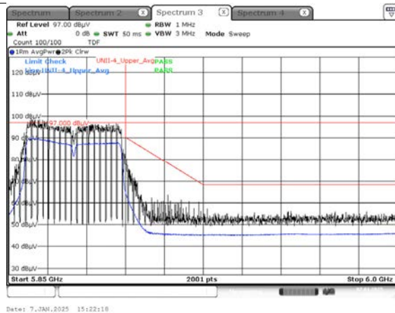
Average Result (802.11ac_VHT40, Ch.175, Y-H)
