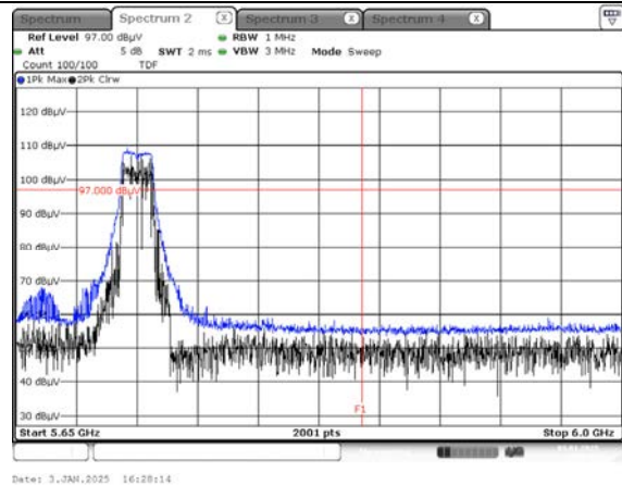
Peak Result (802.11n_HT40, Ch.142, Y-H)
