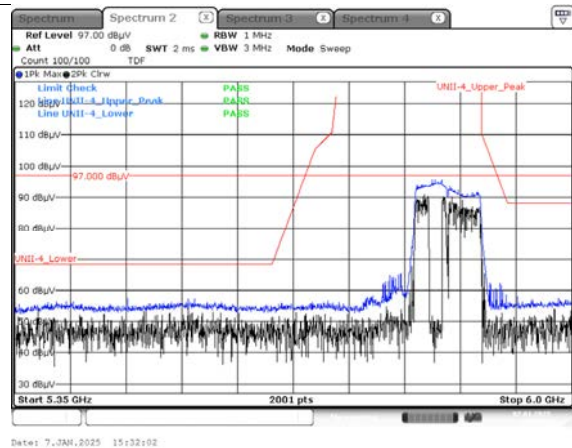
Peak Result (802.11ac_VHT80, Ch.171, Y-H)
