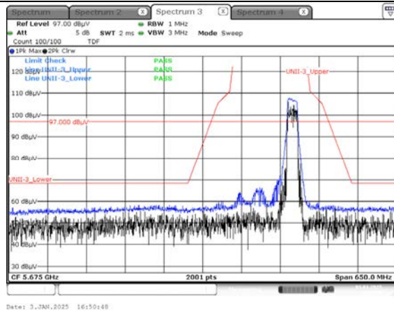
Peak Result (802.11ac_VHT20, Ch.165, Y-H)
