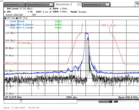
Peak Result (802.11ac_VHT40, Ch.151, Y-H)
