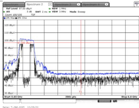
Peak Result (802.11ac_VHT80, Ch.138, Y-H)
