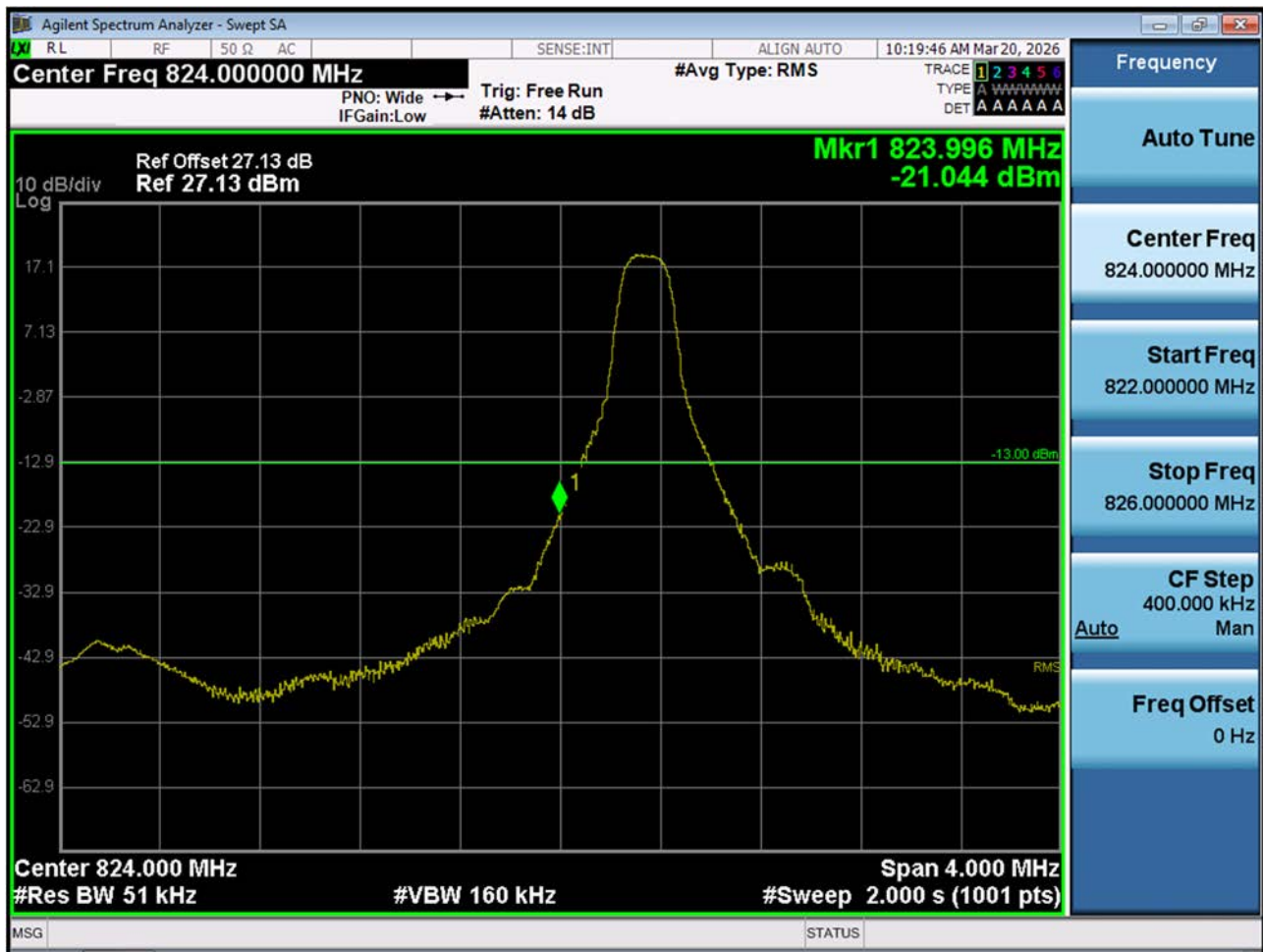
LTE B26_Lower Band Edge Plot (5 M BW Ch.26815 QPSK_RB1_Offset 0)
