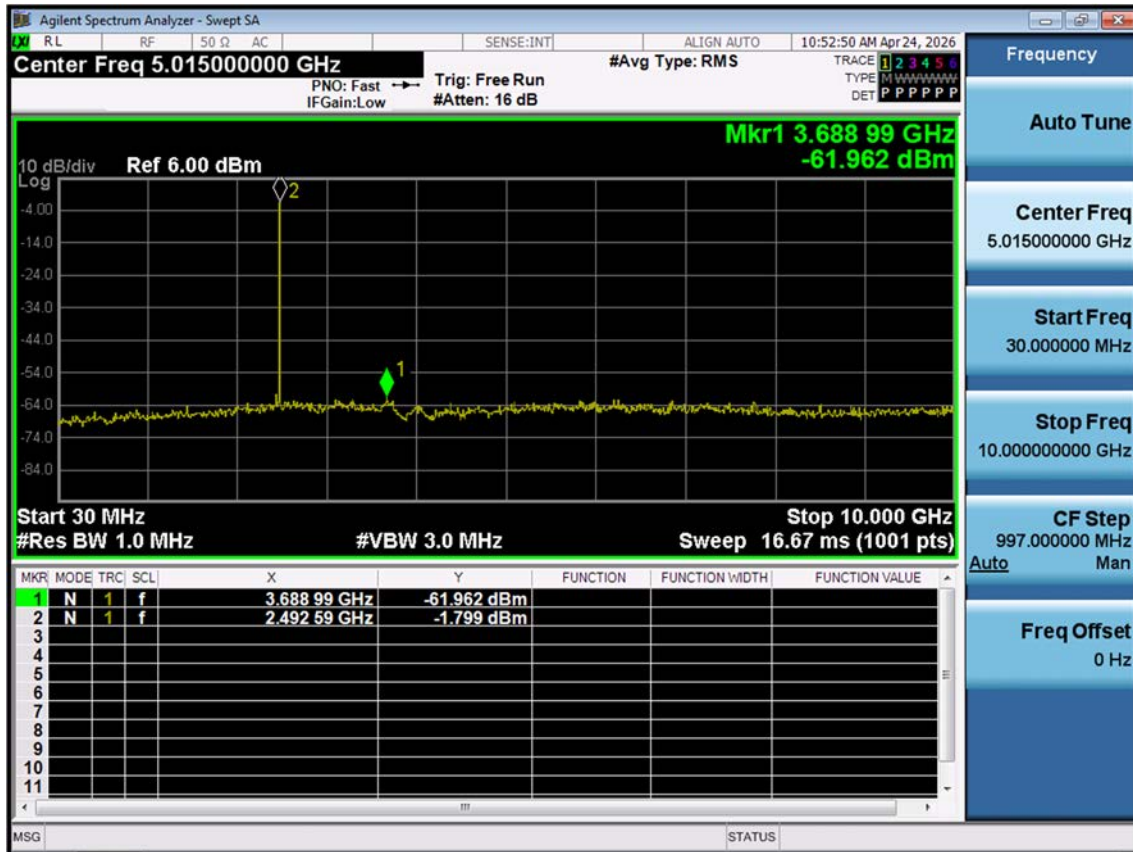
LTE B41_5 M_Conducted Spurious Emissions(30 M-10 G)_Low_QPSK_1RB
