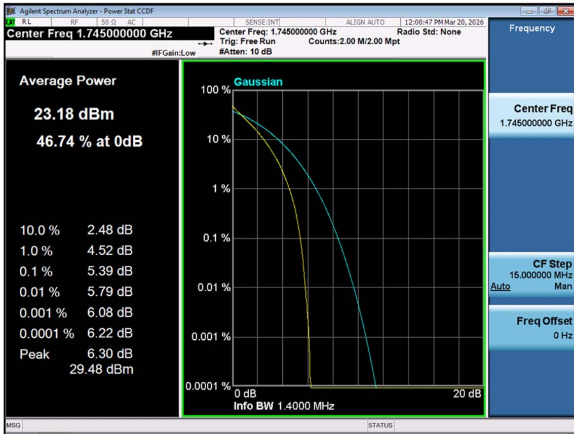
LTE B66_1.4M_PAR_Mid_QPSK_FullRB
