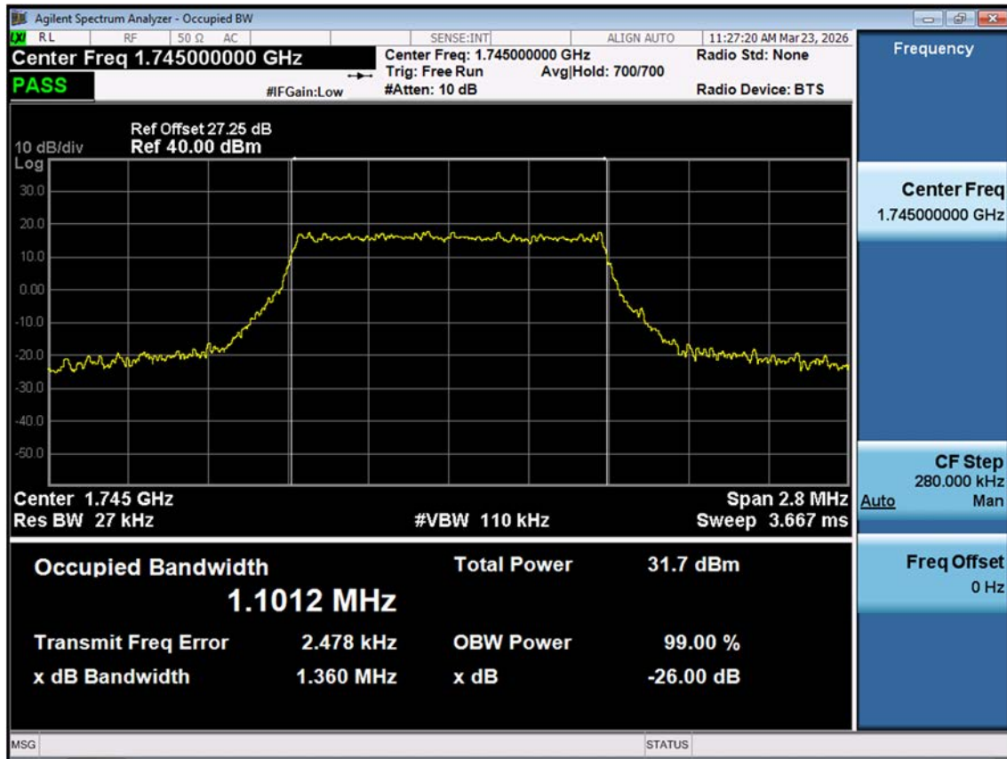
LTE B66_1.4M_OBW_Mid_QPSK_FullRB
