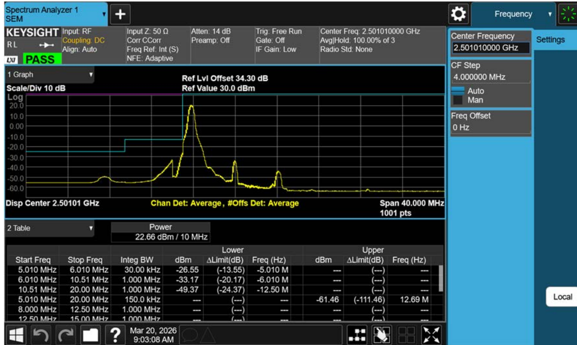
NR n41_10 M_Channel Edge_Lower_Low_PI/2 BPSK_1RB
