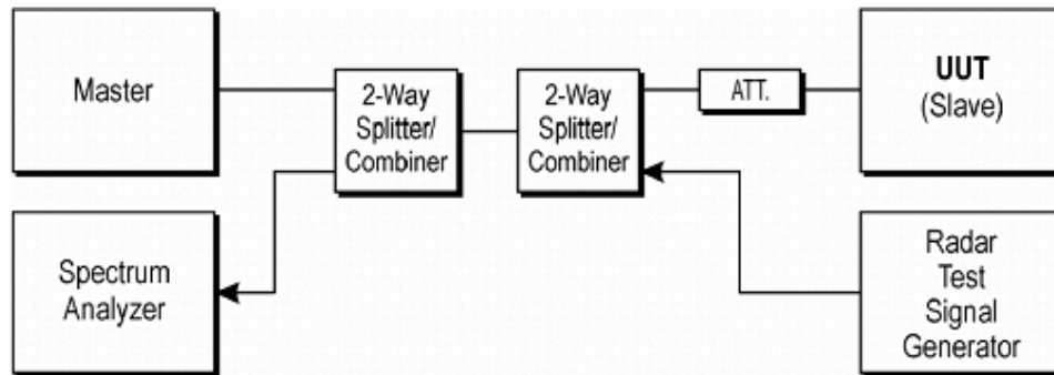
Figure 7-1. Test Setup
