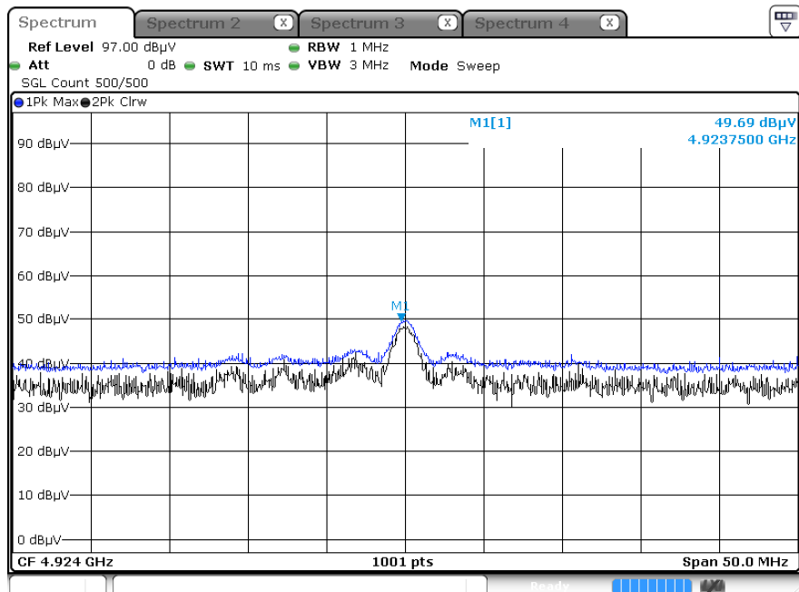
Radiated Spurious Emissions plot – Peak Result (802.11b_1 Mbps, Ch.11 2nd Harmonic, X-V)
