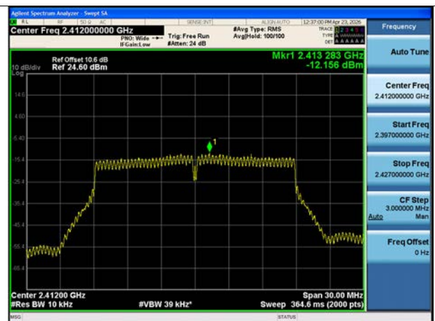
802.11ac_VHT20-CH 1
