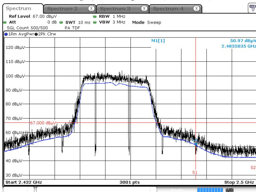
Radiated Restricted Band Edges plot – Average Result (802.11n(HT20)_ MCS0, Ch.11, X-H)
