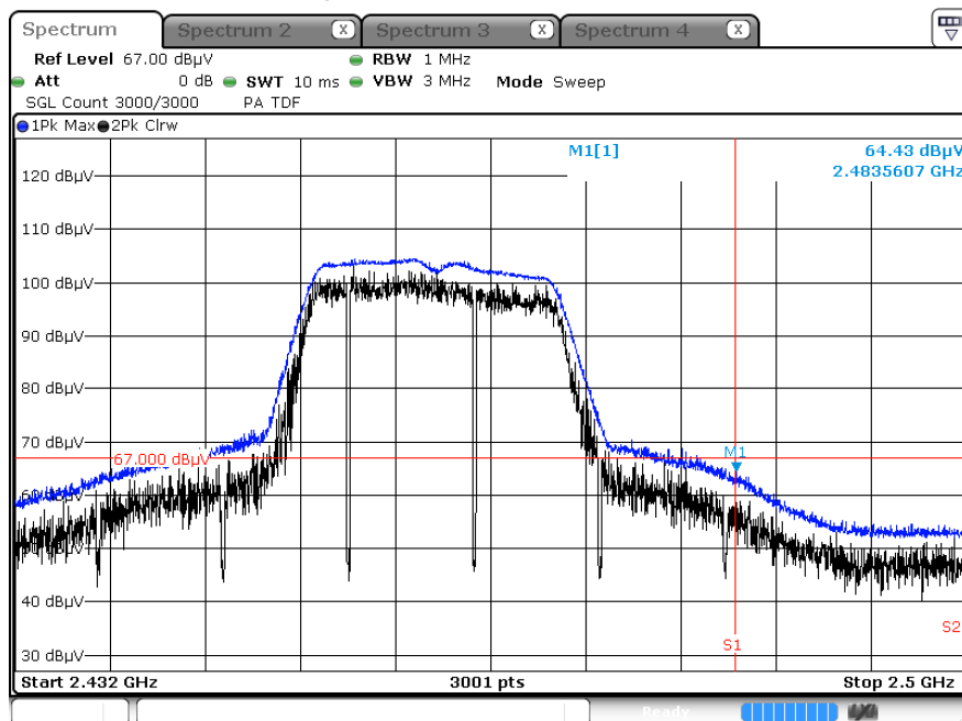
Radiated Restricted Band Edges plot – Peak Result (802.11n(HT20)_ MCS0, Ch.11, X-H)
