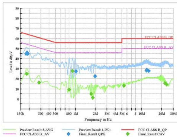
Full Spectrum
