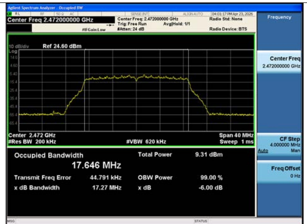
802.11ac_VHT20-CH 13
