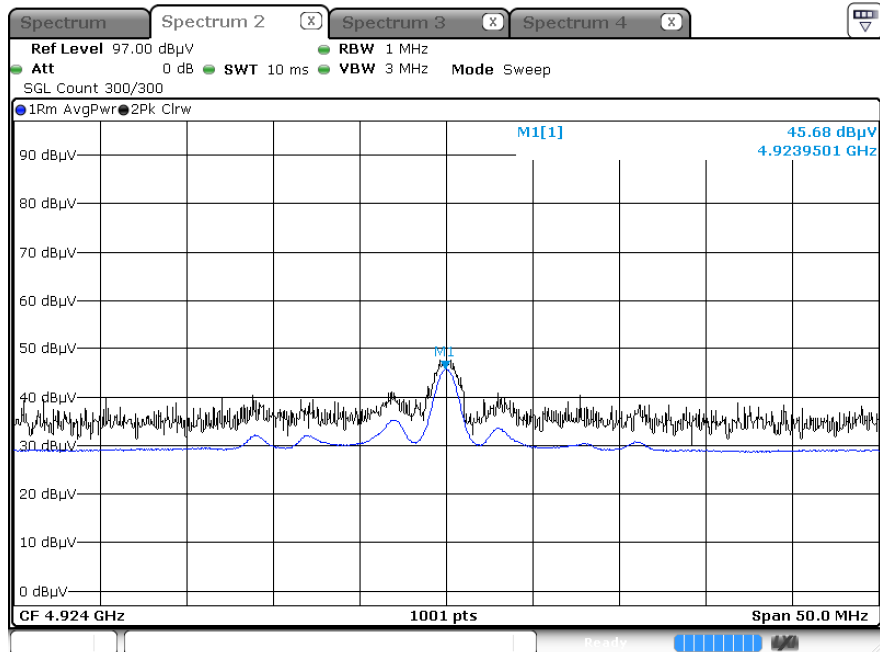
Radiated Spurious Emissions plot – Average Result (802.11b_1 Mbps, Ch.11 2nd Harmonic, X-V)
