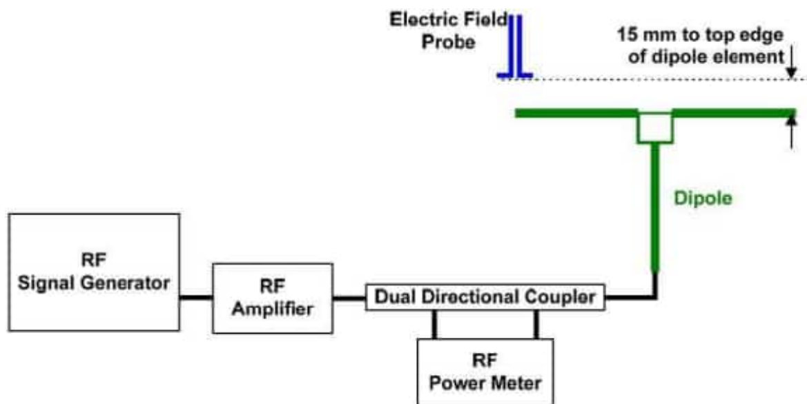
Figure 3. Setup diagram
