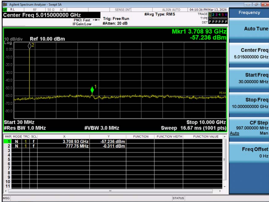
LTE B13_5 M_Conducted Spurious Emissions(30 M-10 G)_Low_QPSK_1RB
