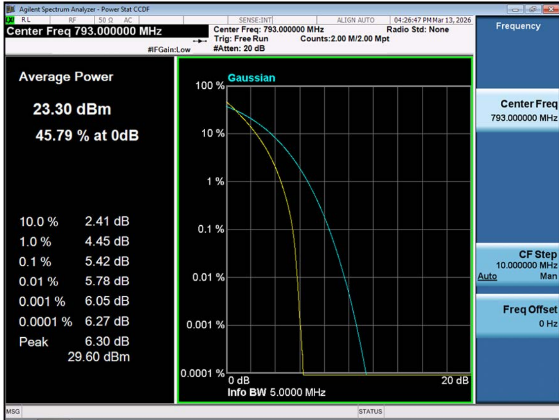
LTE B14_5 M_PAR_Mid_QPSK_FullRB
