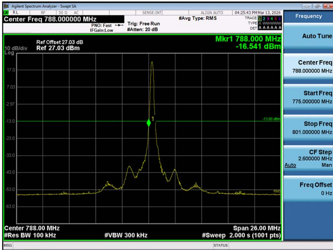
LTE B14_5 M_Band Edge_Low_QPSK_1RB
