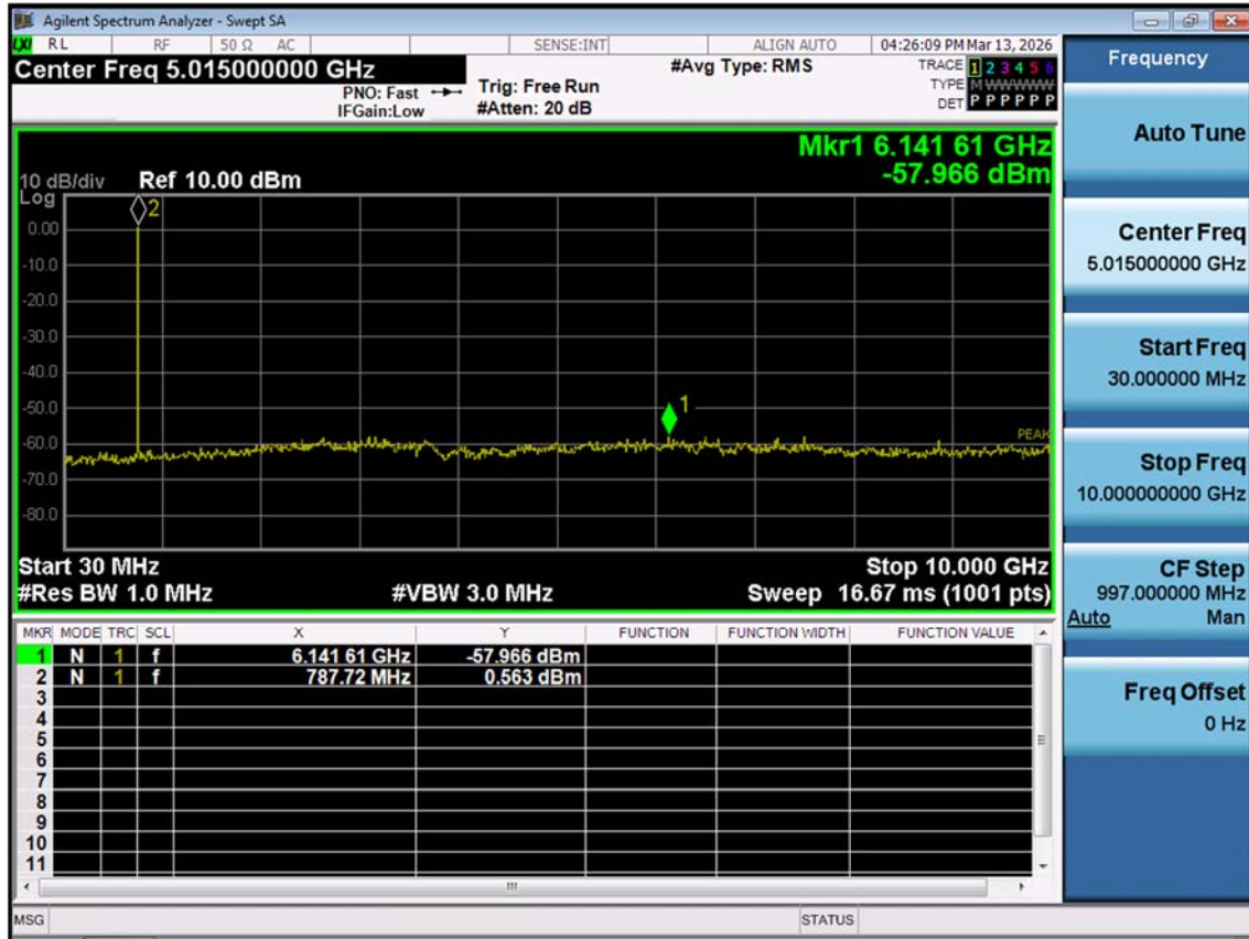
LTE B14_5 M_Conducted Spurious Emissions(30 M-10 G)_Low_QPSK_1RB
