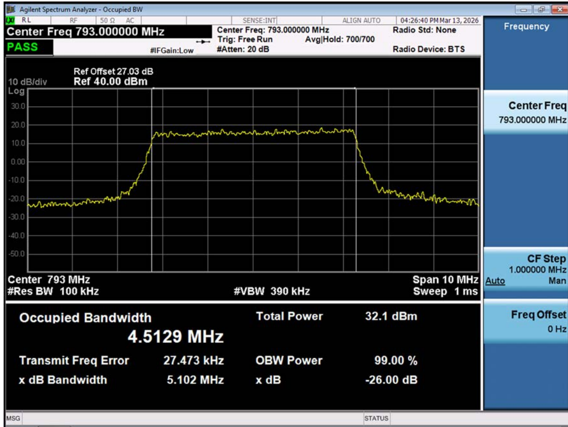
LTE B14_5 M_OBW_Mid_QPSK_FullRB
