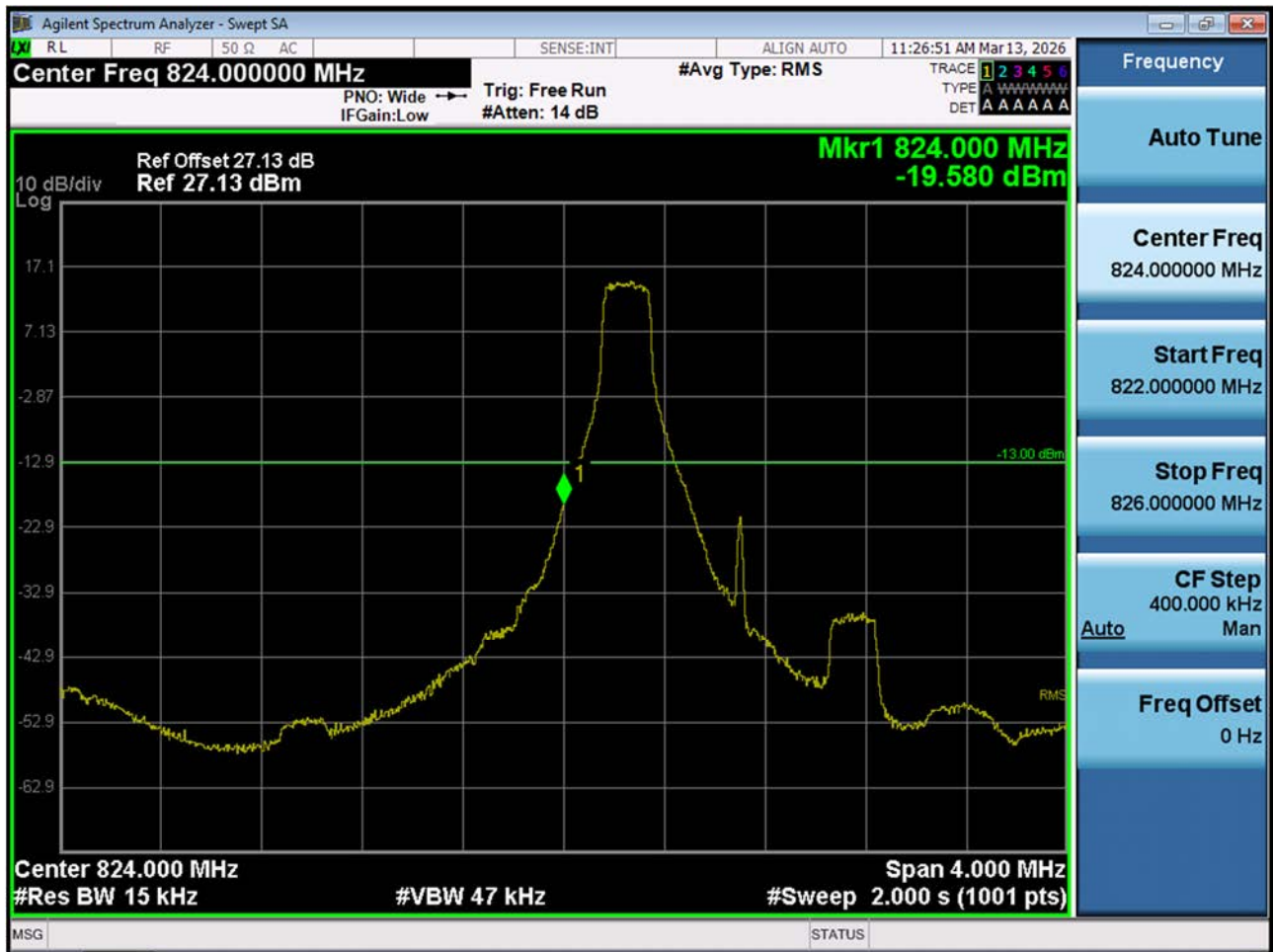
LTE B26(5)_Lower Band Edge Plot (1.4 M BW Ch.26797 QPSK_RB1_Offset 0)
