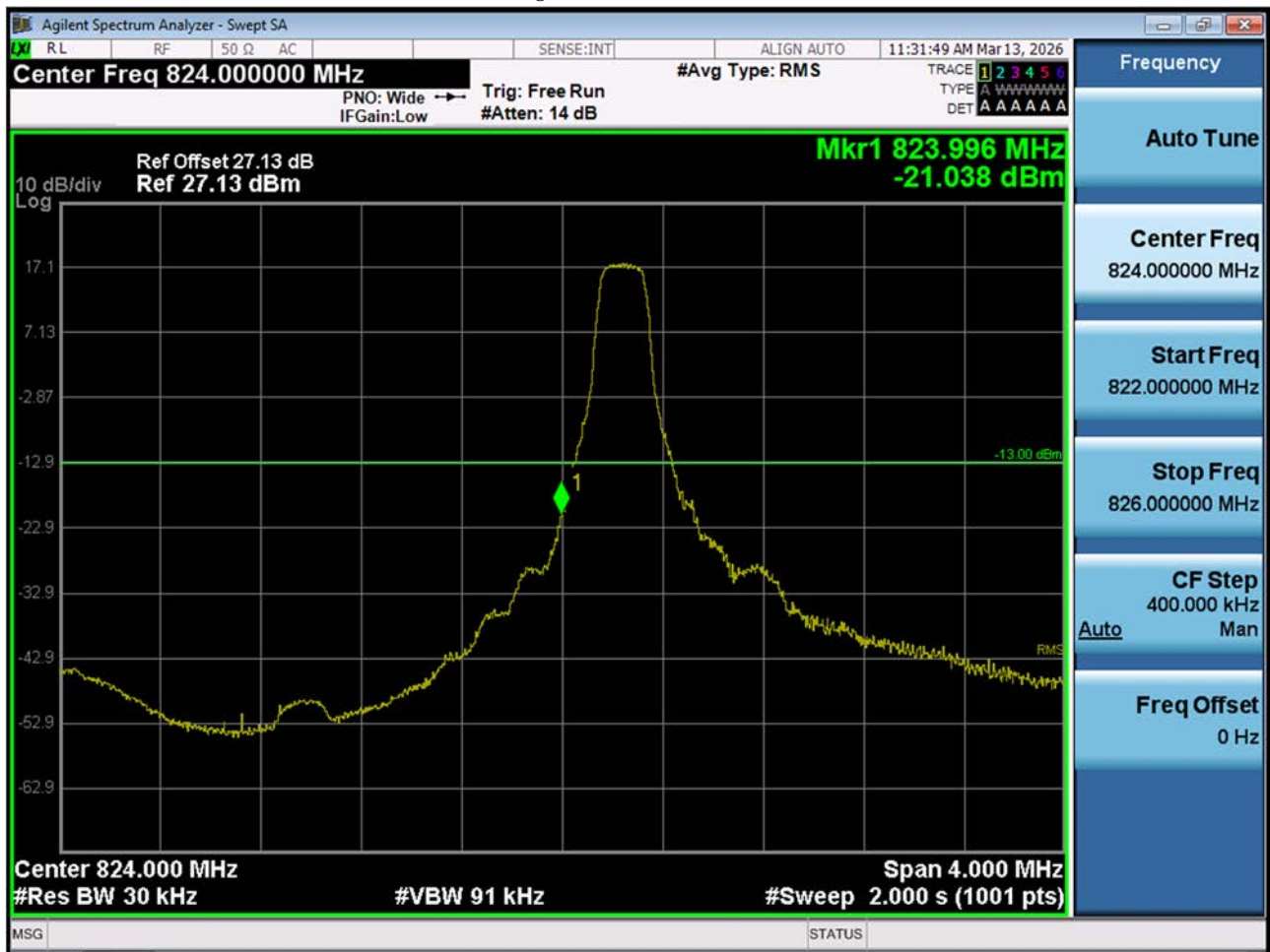
LTE B26(5)_Lower Band Edge Plot (3 M BW Ch.26805 QPSK_RB1_Offset 0)
