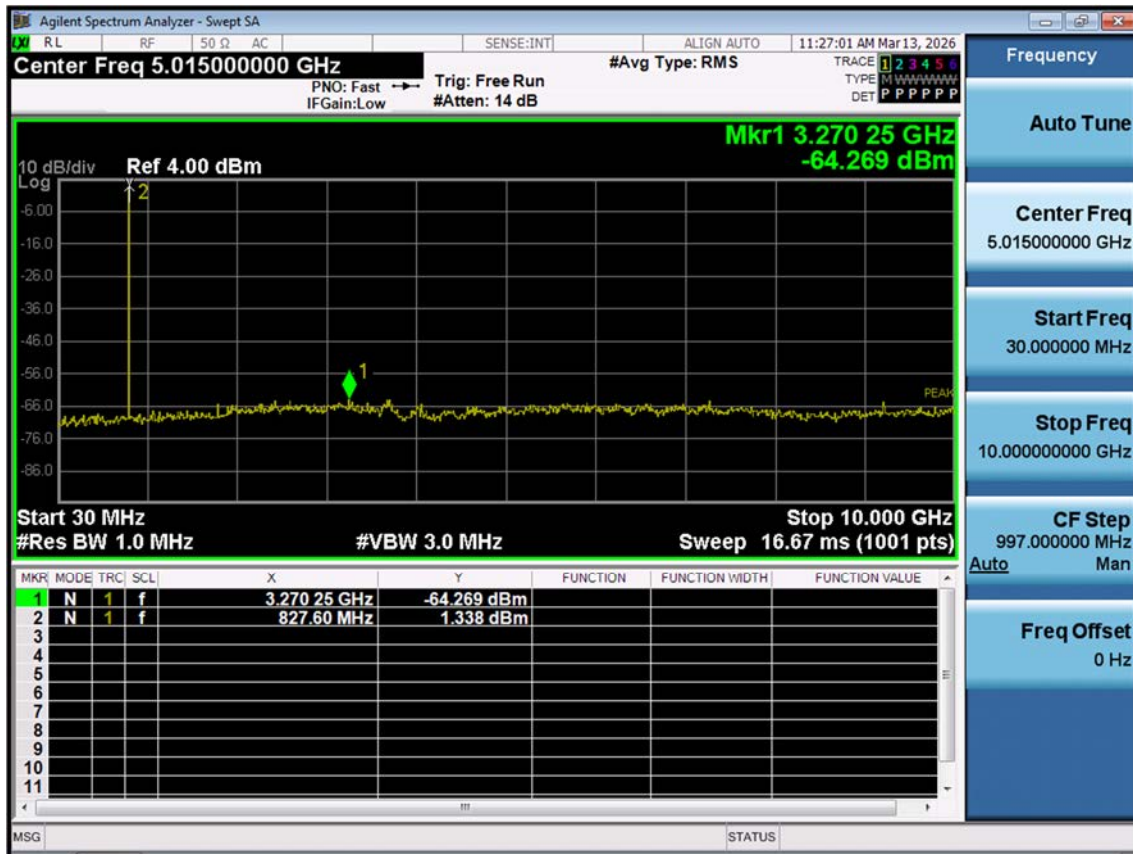
LTE B26(5)_1.4 M_Conducted Spurious Emissions(30 M-10 G)_Low_QPSK_1RB
