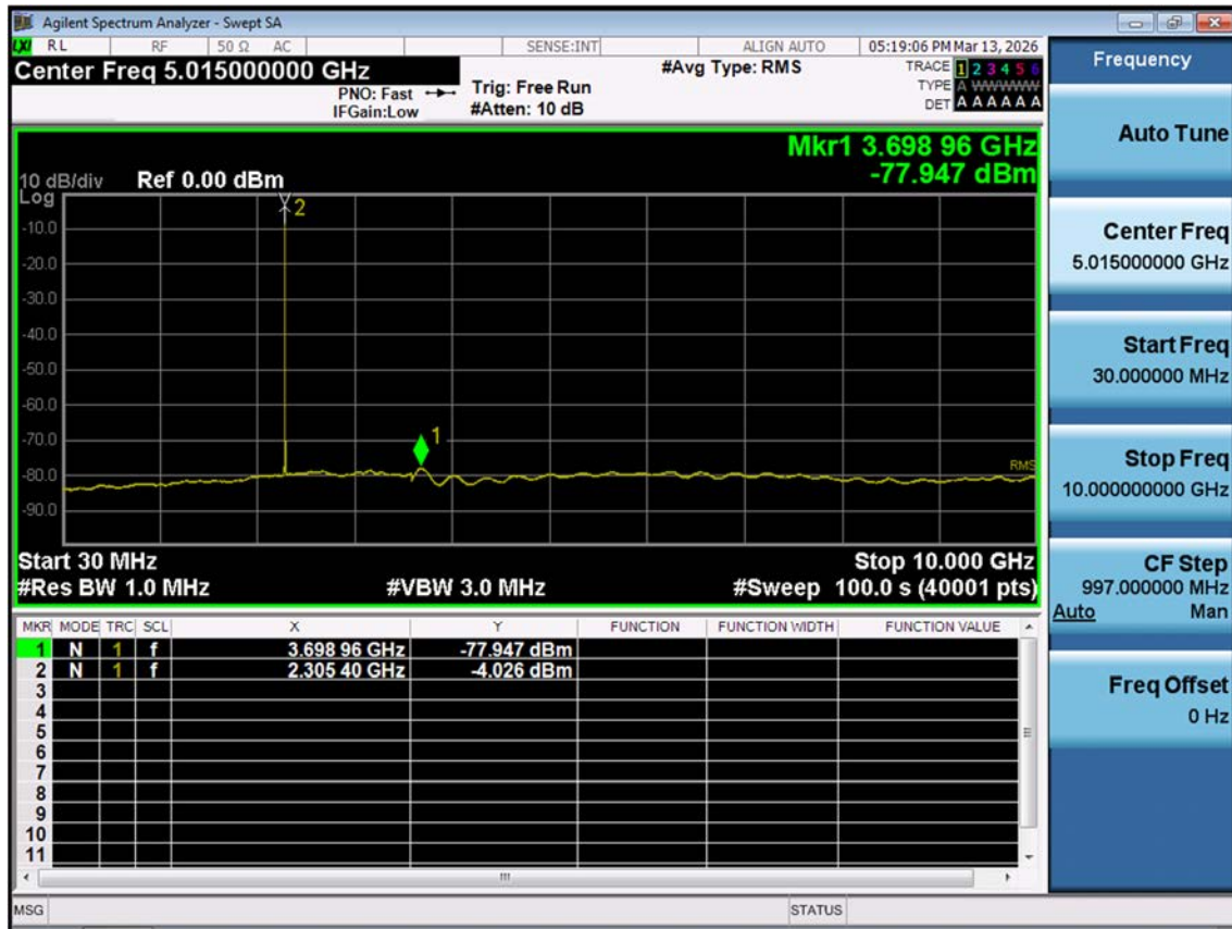
LTE B30_5 M_Conducted Spurious Emissions(30 M-10 G)_Low_QPSK_1RB
