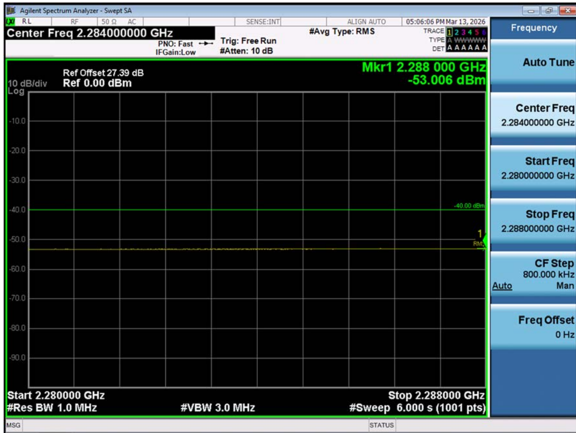
LTE B30_5 M_Band Edge(2280MHz-2288MHz)_Low_QPSK_FullRB
