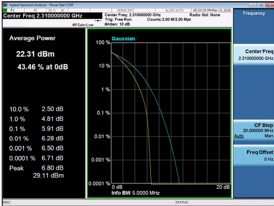
LTE B30_5 M_PAR_Mid_QPSK_FullRB
