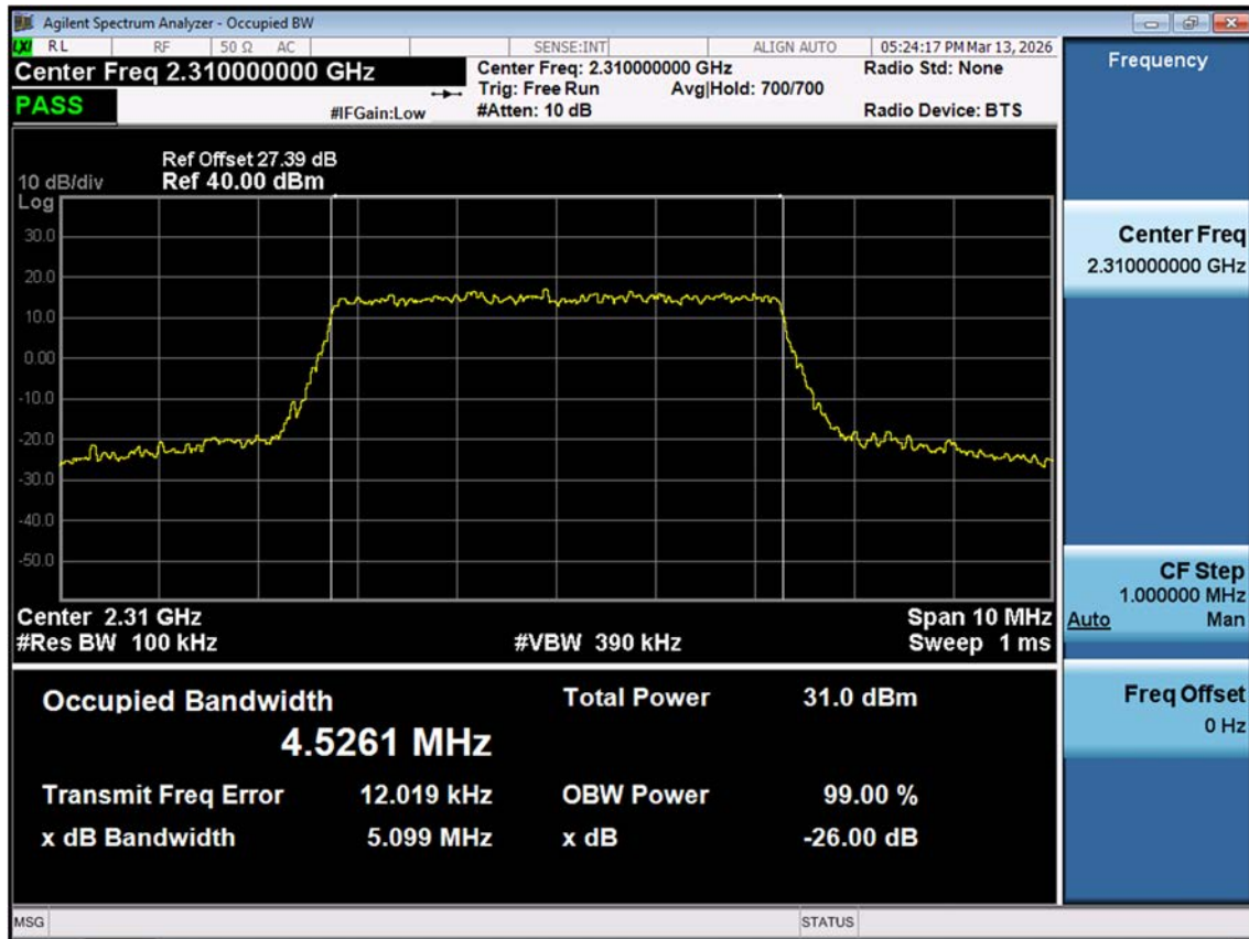
LTE B30_5 M_OBW_Mid_QPSK_FullRB
