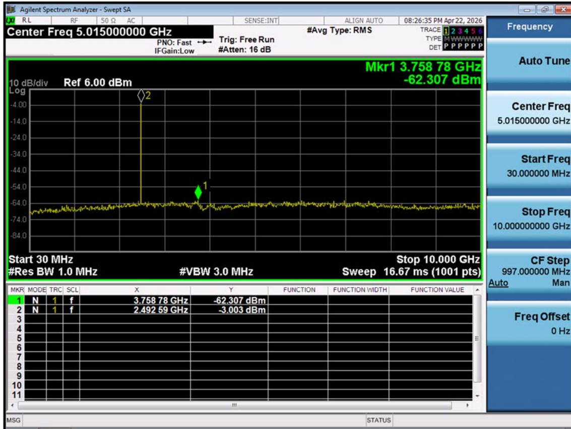
LTE B41(38)_5 M_Conducted Spurious Emissions(30 M-10 G)_Low_QPSK_1RB
