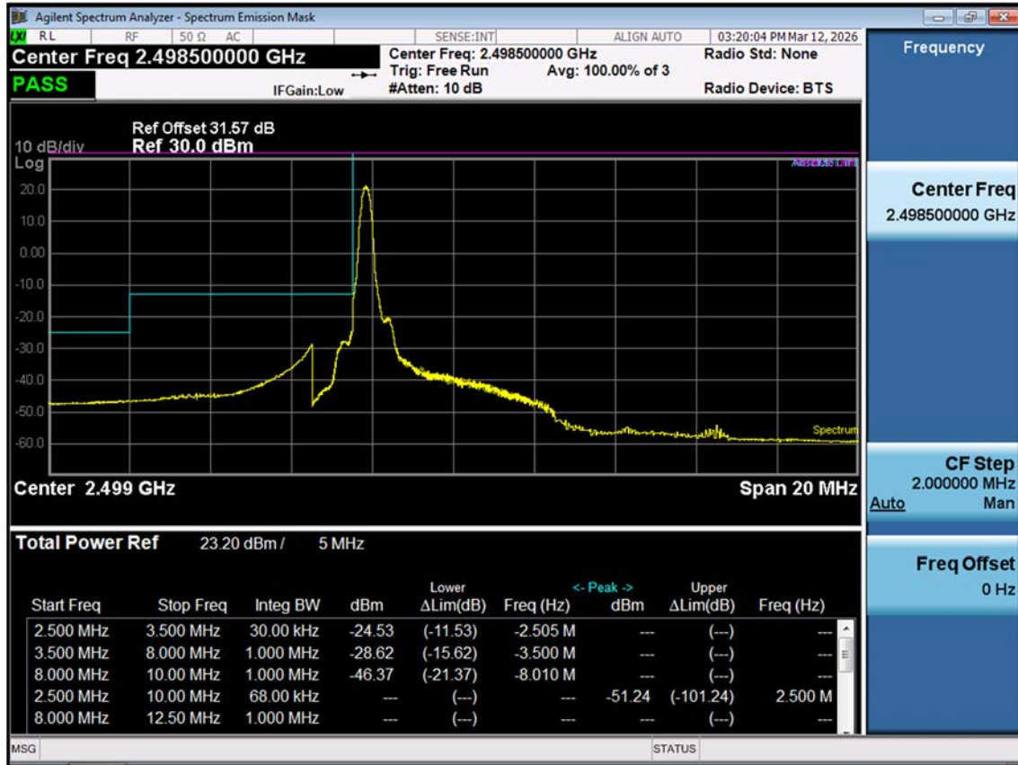
LTE B41(38)_5 M_Channel Edge_Lower_Low_QPSK_1RB
