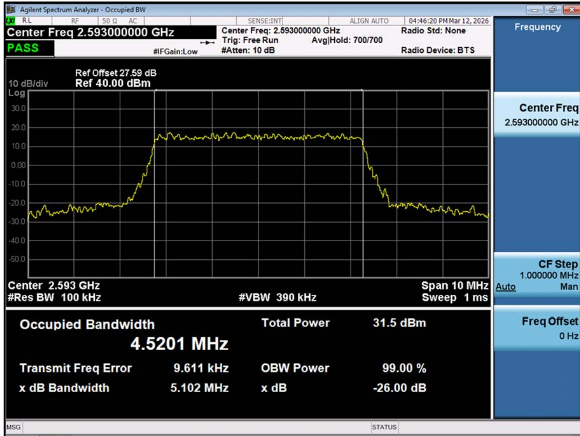
LTE B41(38)_5 M_OBW_Mid_QPSK_FullRB
