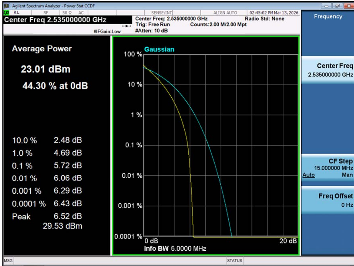
LTE B7_5 M_PAR_Mid_QPSK_FullRB
