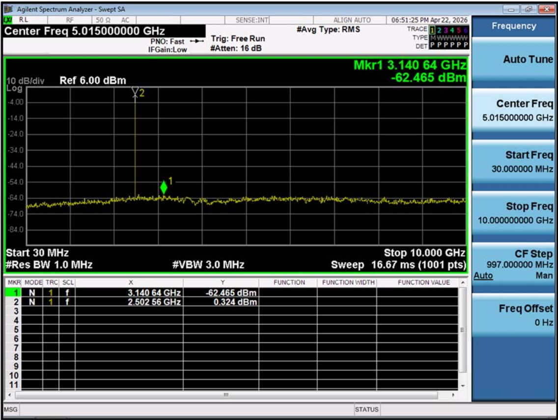
LTE B7_5 M_Conducted Spurious Emissions(30 M-10 G)_Low_QPSK_1RB
