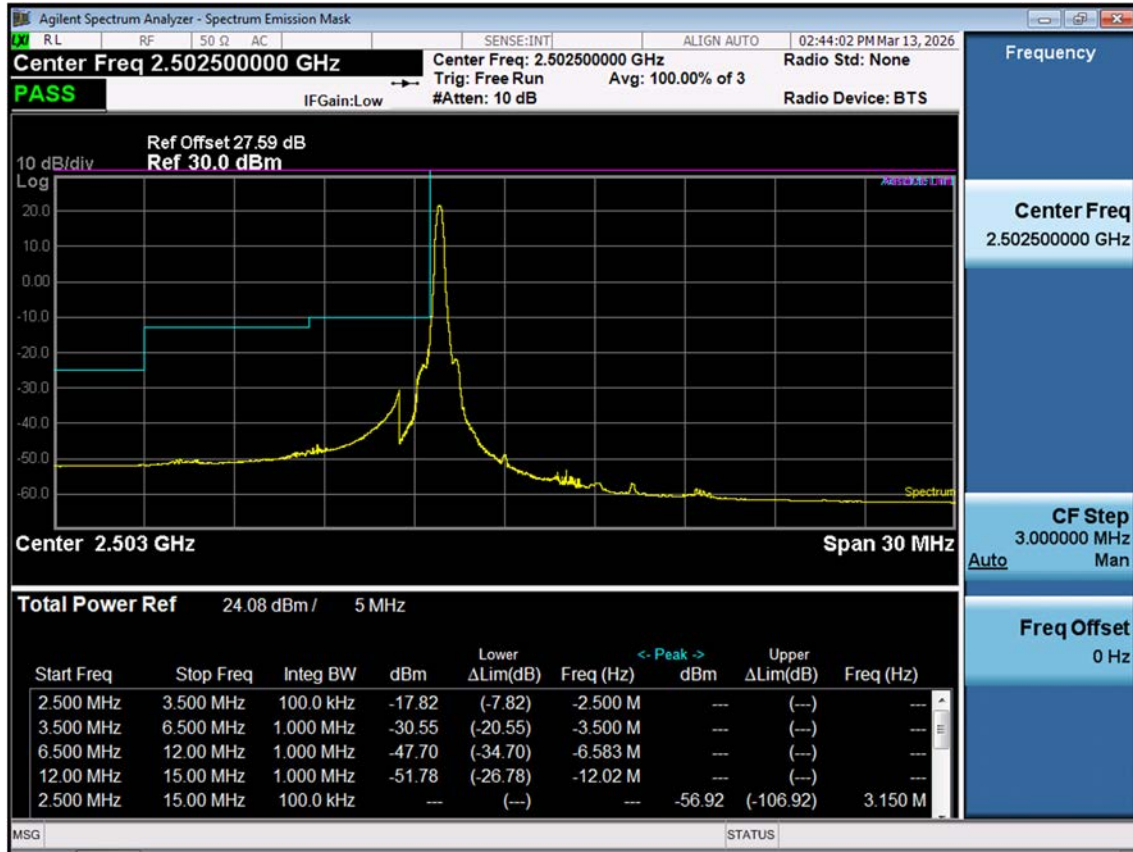
LTE B7_5 M_Channel Edge_Lower_Low_QPSK_1RB
