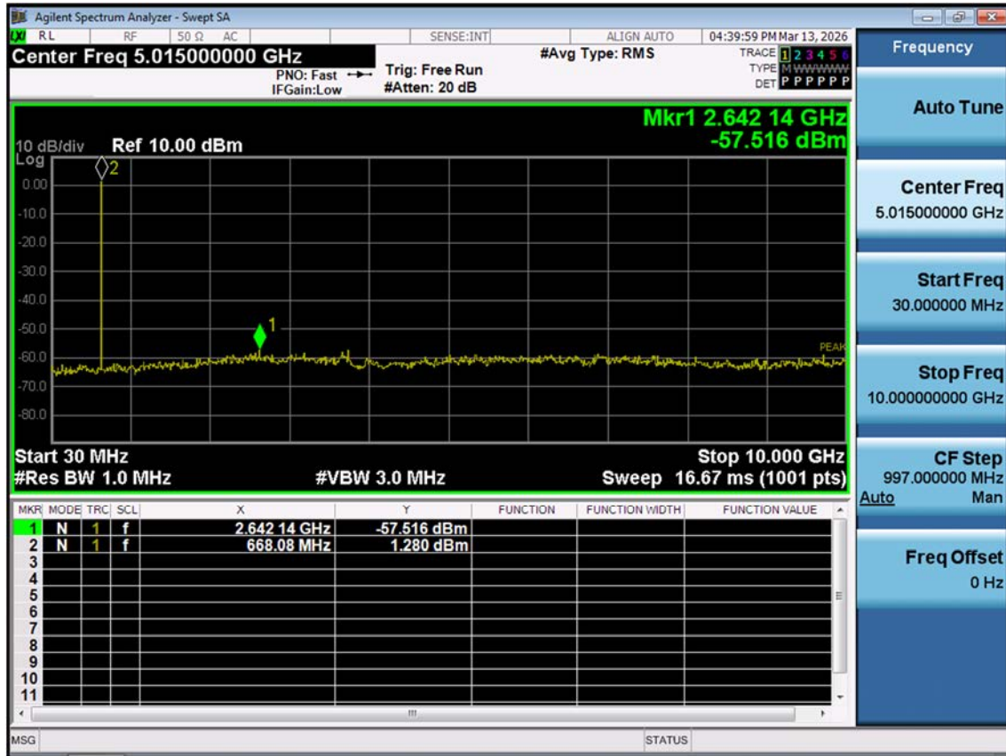
LTE B71_5 M_Conducted Spurious Emissions(30 M-10 G)_Low_QPSK_1RB
