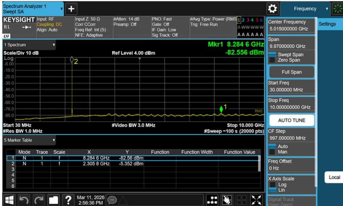
NR n30_5 M_Conducted Spurious Emissions(30 M-10 G)_Low_PI/2 BPSK_1RB
