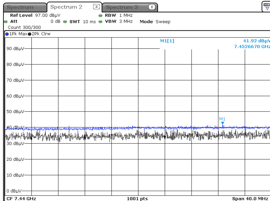
Radiated Spurious Emissions plot – Peak &amp; Average Result (2-DH5, Ch. 78 3rd Harmonic, Z-H)
