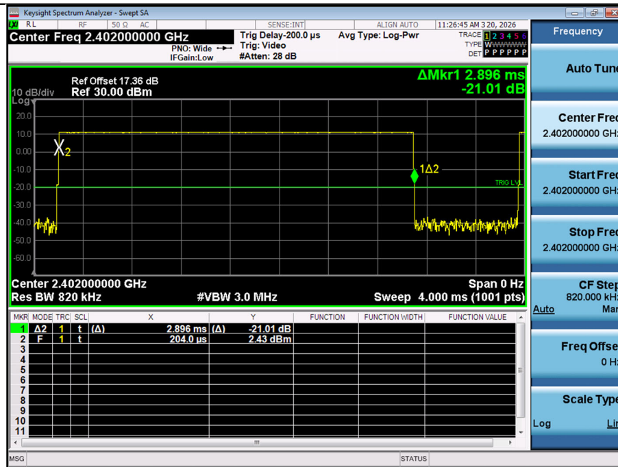
GFSK : Dwell Time(Ch. 0)
