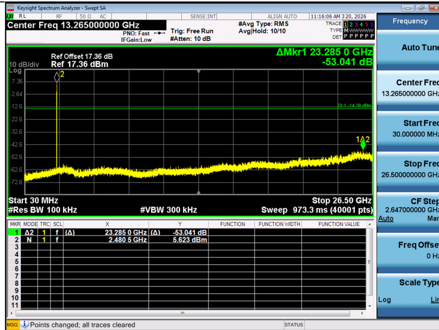
Conducted Spurious Emissions (30 MHz - 26.50 GHz) \pi /4DQPSK Ch. 78
