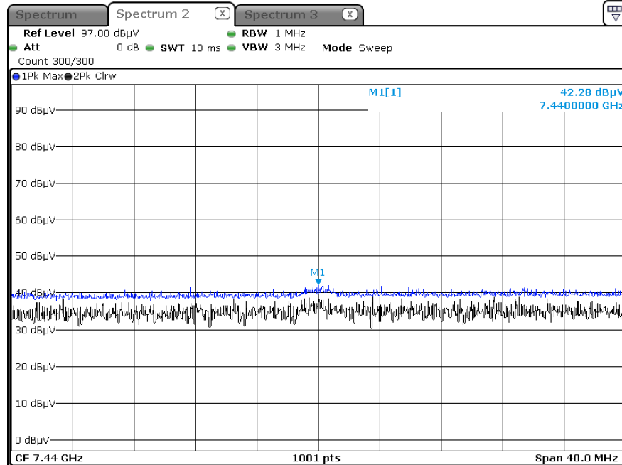
Radiated Spurious Emissions plot – Peak &amp; Average Result (DH5, Ch. 78 3rd Harmonic, Z-H)
