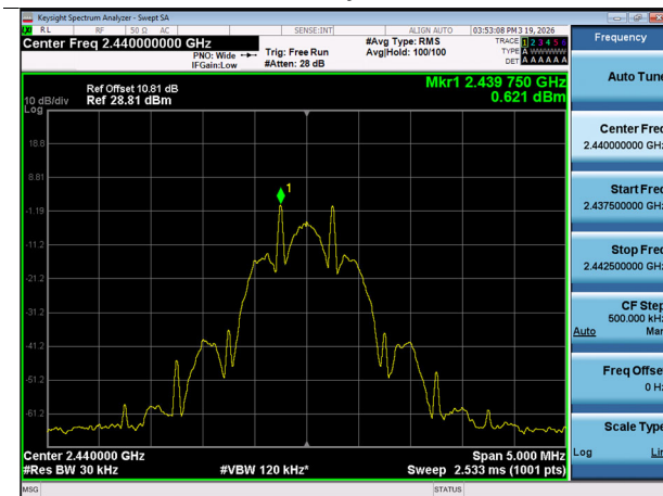
125k Bit/s 37 Byte (Mid-CH 17)
