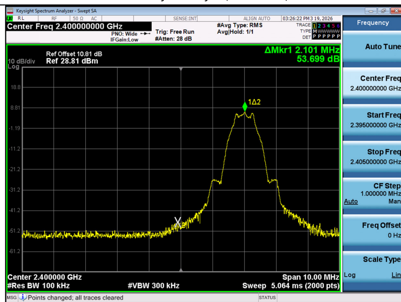
1M 37Byte 37 Byte (Low-CH 37)
