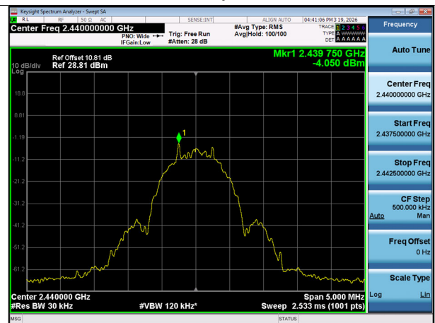
500k Bit/s 37 Byte (Mid-CH 17)
