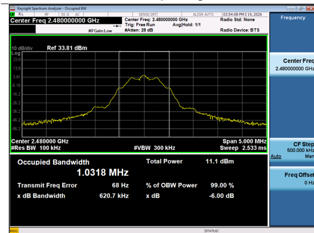
125k Bit/s 37 Byte (High-CH 39)
