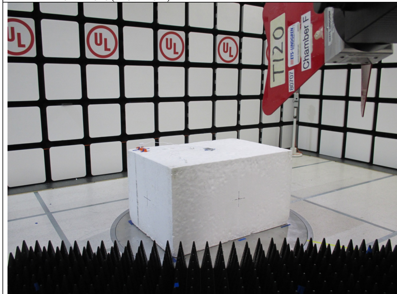
RADIATED FRONT PHOTO (ABOVE 1 GHz)
