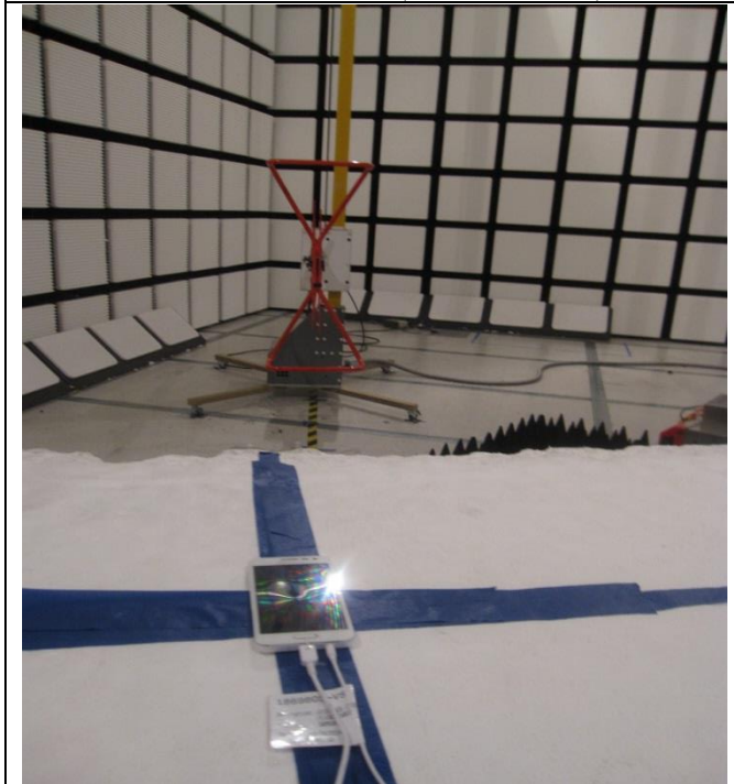
RADIATED FRONT=PHOTO (BELOW 1 GHz)
