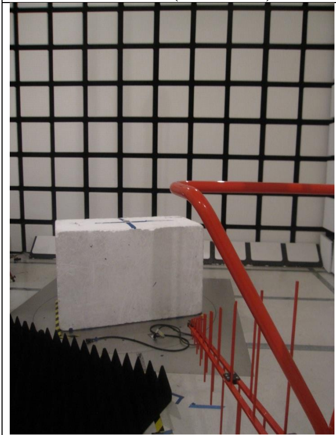
RADIATED BACK PHOTO (BELOW 1 GHz)
