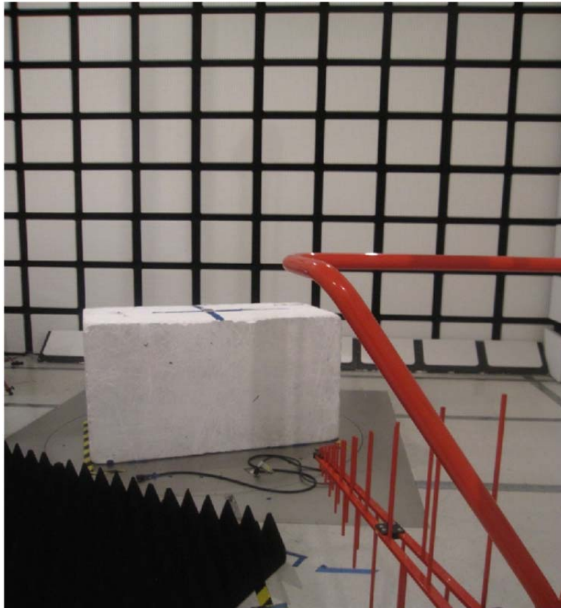
RADIATED FRONT PHOTO (BELOW 1 GHz)
