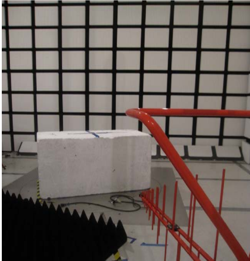
RADIATED FRONT PHOTO (BELOW 1 GHz)
