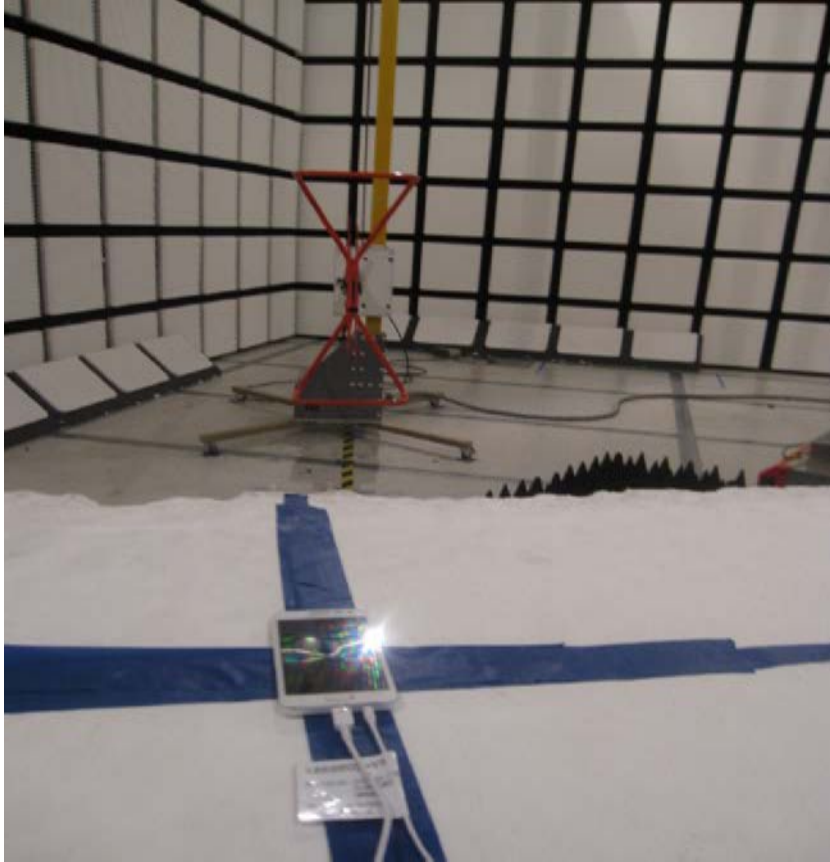
RADIATED BACK PHOTO (BELOW 1 GHz)
