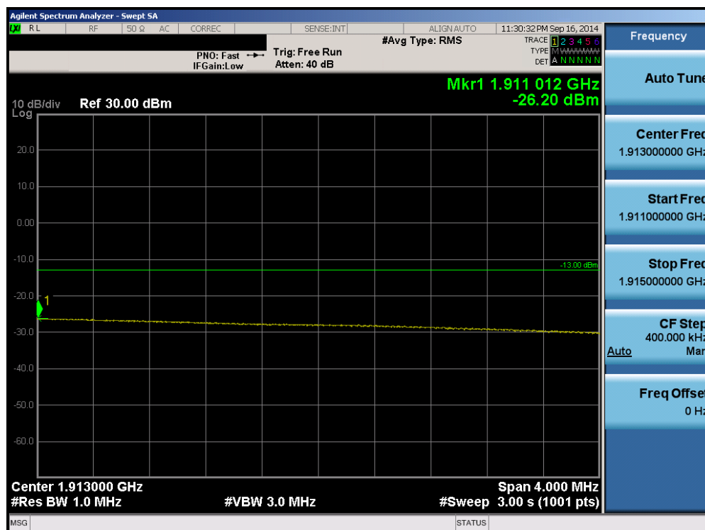
Plot 6-120. Upper Extended Band Edge Plot (Band 2 - 20.0MHz QPSK - RB Size 100)
