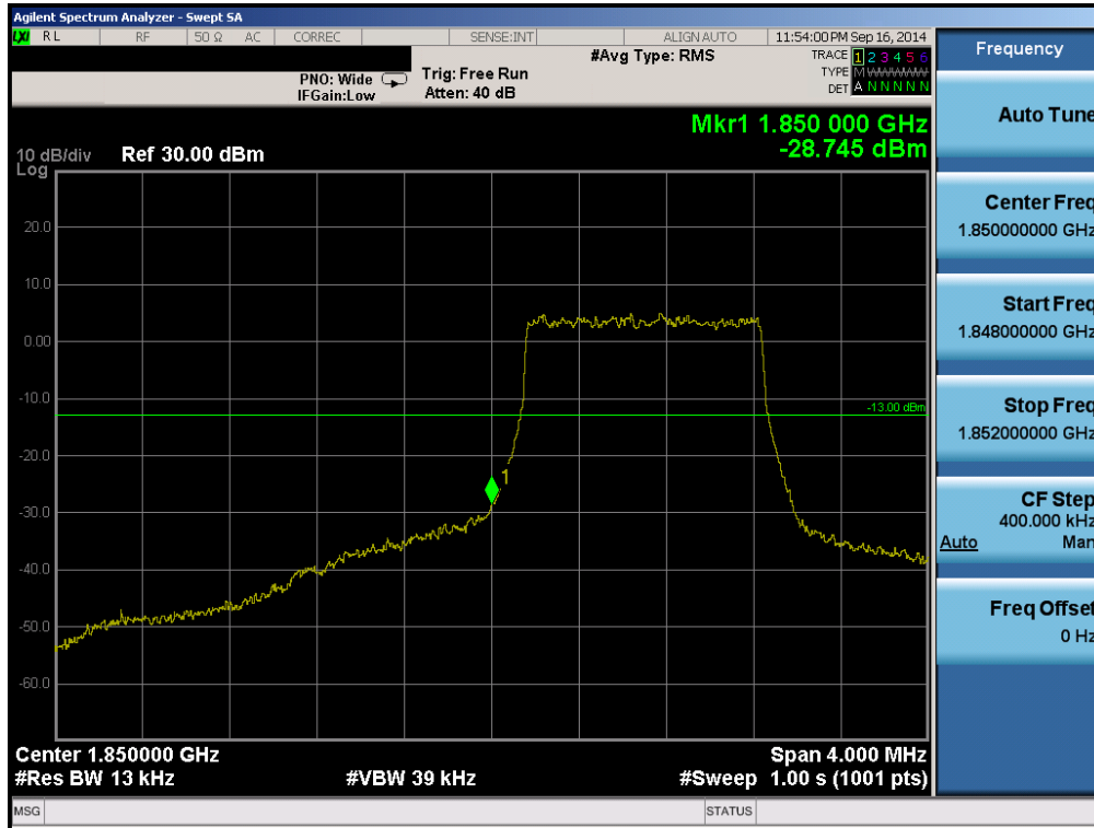
Plot 6-97. Lower Band Edge Plot (Band 2 – 1.4MHz QPSK – RB Size 6)
