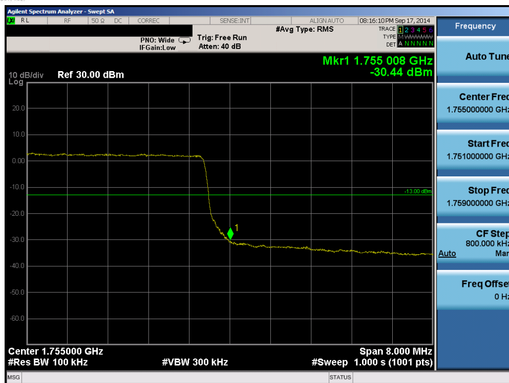
Plot 6-87. Upper Band Edge Plot (Band 4 – 10.0MHz QPSK – RB Size 50)
