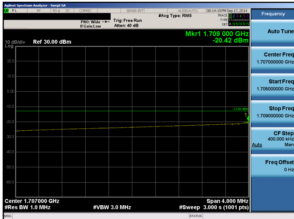
Plot 6-86. Lower Extended Band Edge Plot (Band 4 – 10.0MHz QPSK – RB Size 50)
