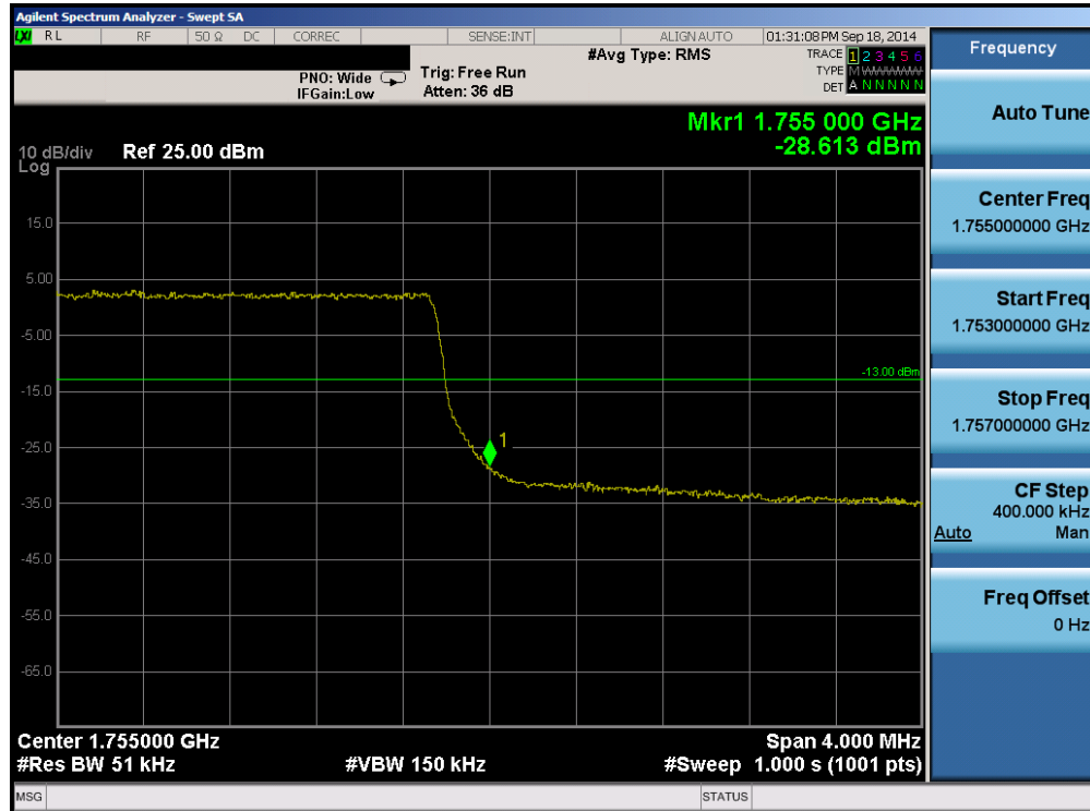
Plot 6-83. Upper Band Edge Plot (Band 4 - 5.0MHz QPSK - RB Size 25)
