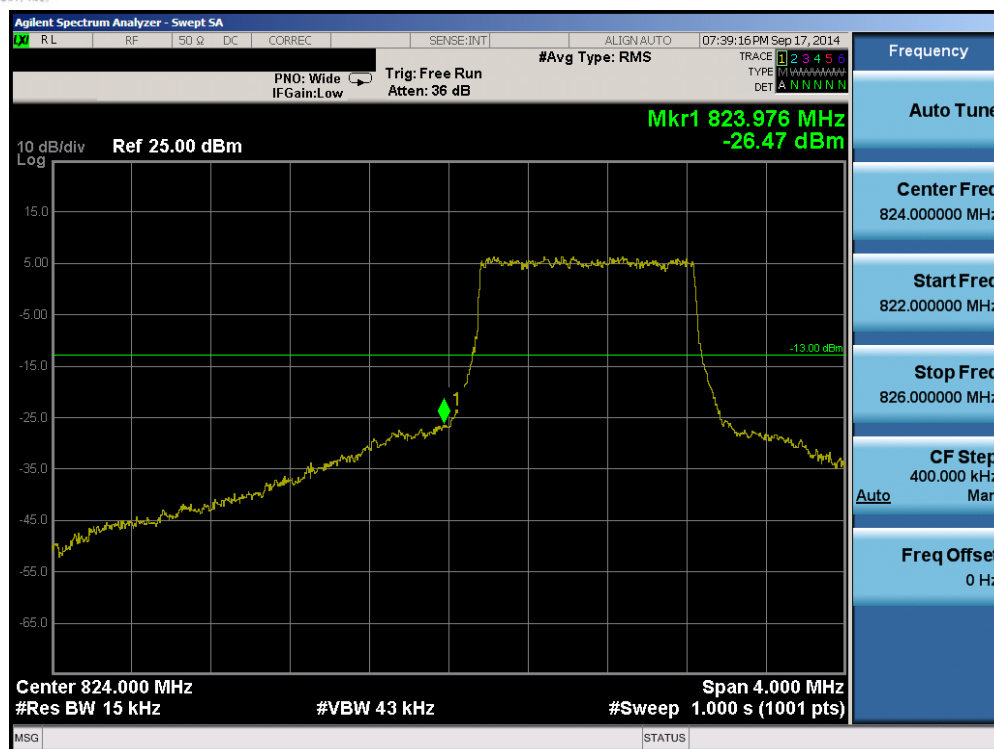
Plot 6-65. Lower Band Edge Plot (Band 5 – 1.4MHz QPSK – RB Size 6)
