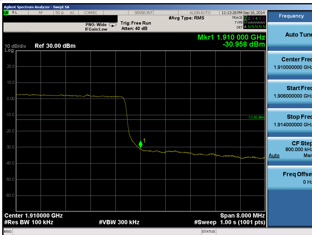
Plot 6-111. Upper Band Edge Plot (Band 2 – 10.0MHz QPSK – RB Size 50)
