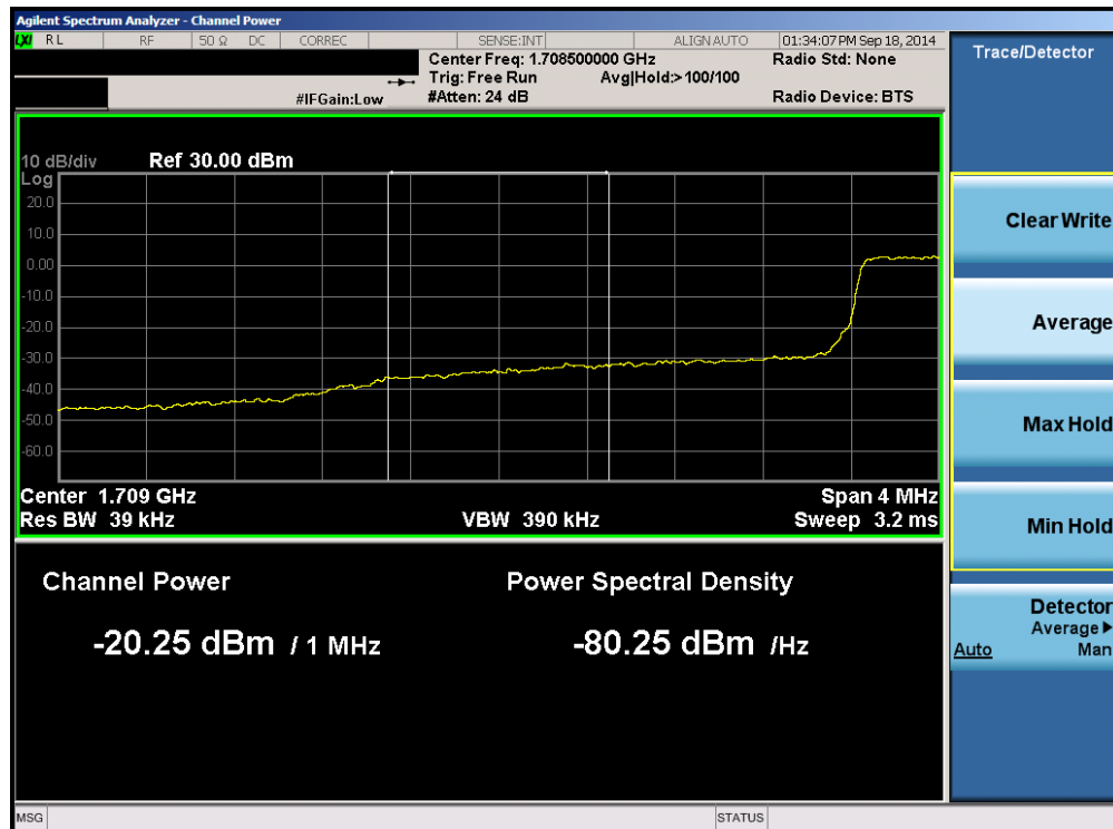
Plot 6-78. Lower Extended Band Edge Plot (Band 4 – 3.0MHz QPSK – RB Size 15)
