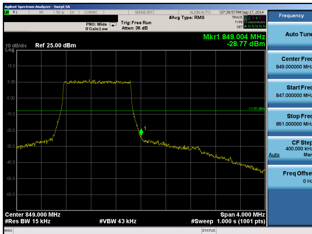
Plot 6-66. Upper Band Edge Plot (Band 5 – 1.4MHz QPSK – RB Size 6)
