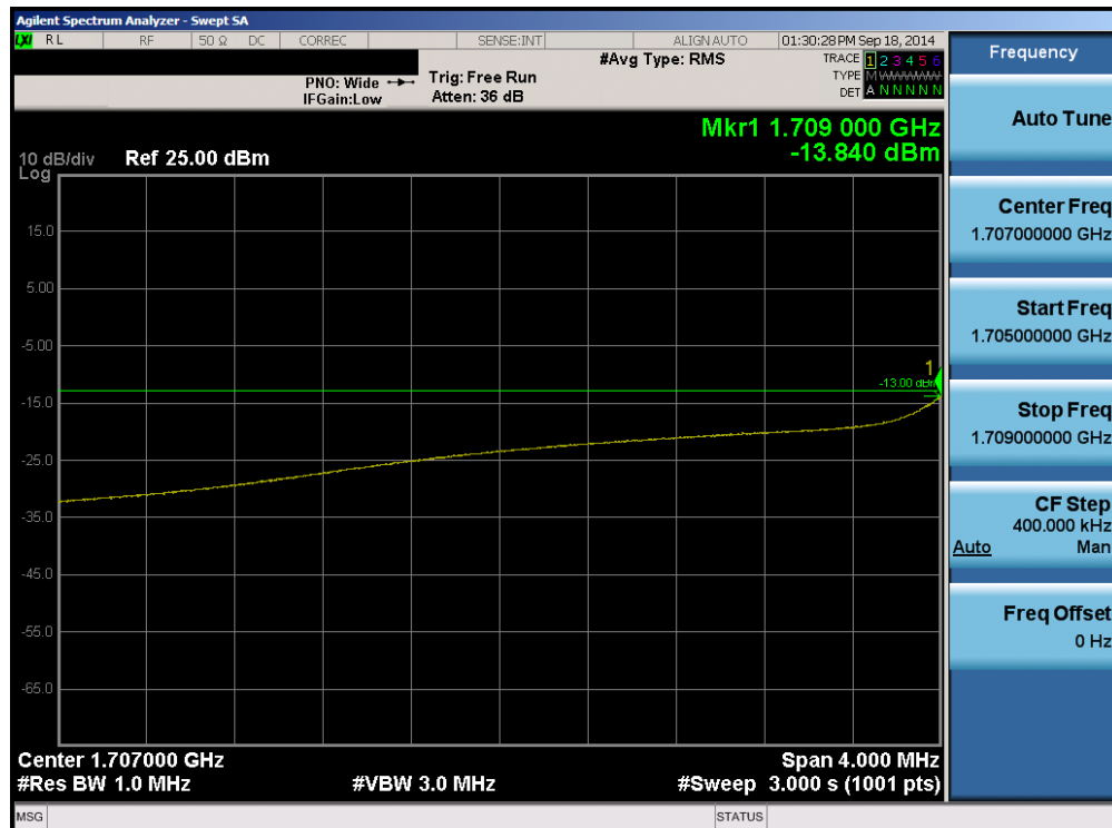
Plot 6-82. Lower Extended Band Edge Plot (Band 4 – 5.0MHz QPSK – RB Size 25)
