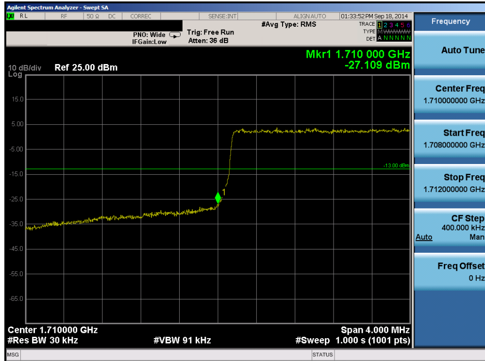
Plot 6-77. Lower Band Edge Plot (Band 4 – 3.0MHz QPSK – RB Size 15)
