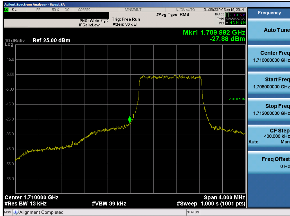
Plot 6-73. Lower Band Edge Plot (Band 4 – 1.4MHz QPSK – RB Size 6)
