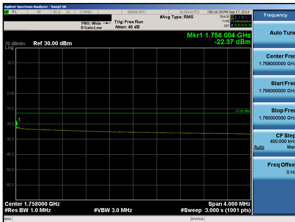
Plot 6-88. Upper Extended Band Edge Plot (Band 4 – 10.0MHz QPSK – RB Size 50)
