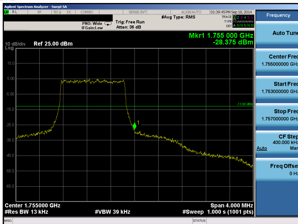
Plot 6-75. Upper Band Edge Plot (Band 4 – 1.4MHz QPSK – RB Size 6)
