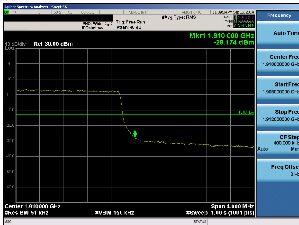
Plot 6-107. Upper Band Edge Plot (Band 2 - 5.0MHz QPSK - RB Size 25)
