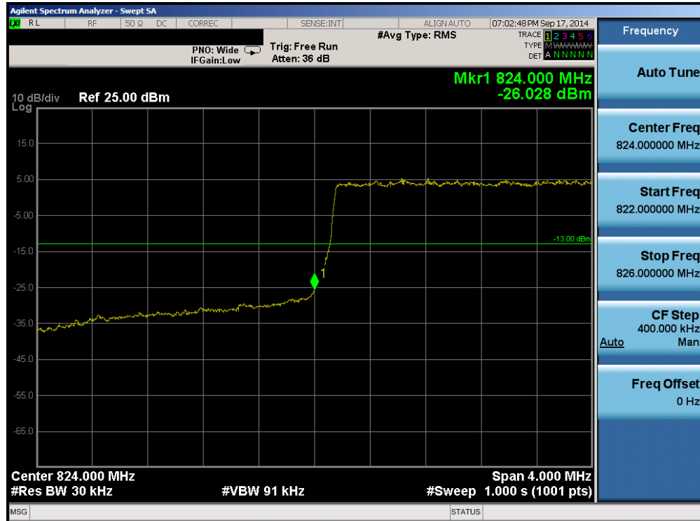
Plot 6-67. Lower Band Edge Plot (Band 5 – 3.0MHz QPSK – RB Size 15)
