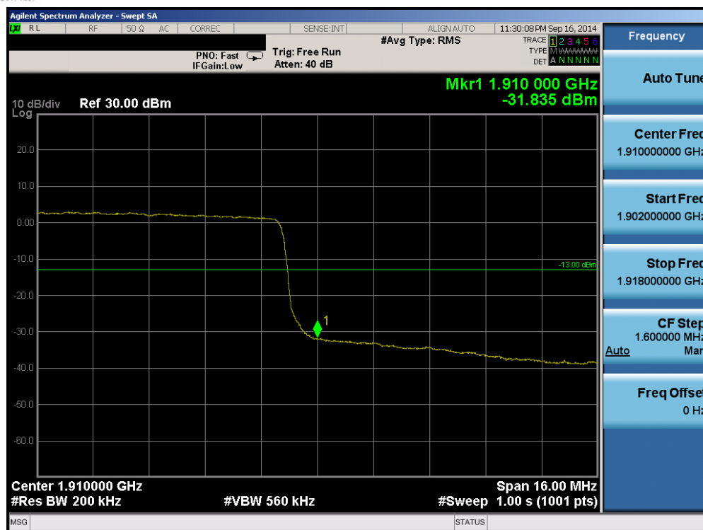
Plot 6-119. Upper Band Edge Plot (Band 2 - 20.0MHz QPSK - RB Size 100)
