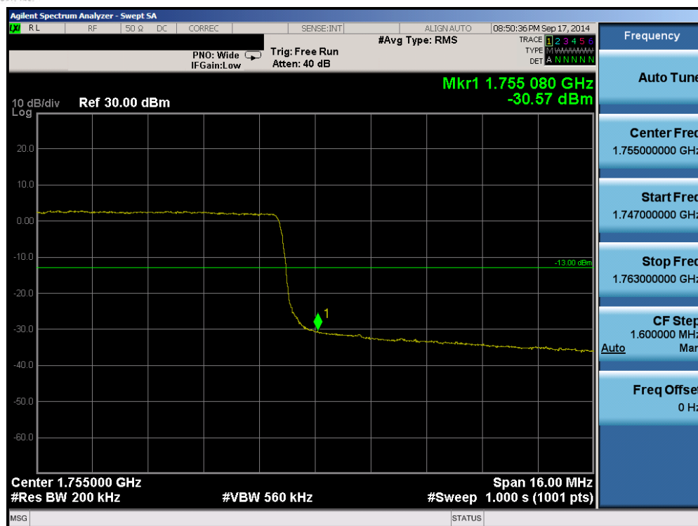
Plot 6-95. Upper Band Edge Plot (Band 4 – 20.0MHz QPSK – RB Size 100)
