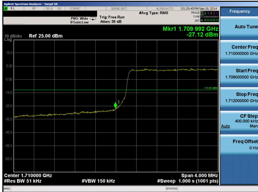
Plot 6-81. Lower Band Edge Plot (Band 4 – 5.0MHz QPSK – RB Size 25)
