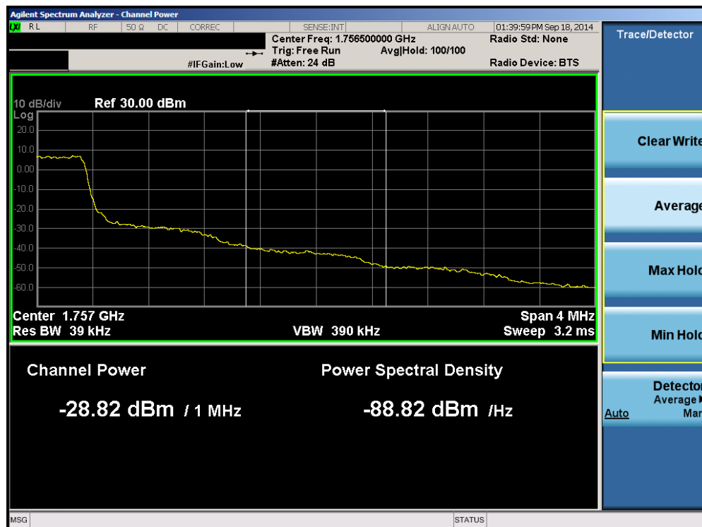
Plot 6-76. Upper Extended Band Edge Plot (Band 4 – 1.4MHz QPSK – RB Size 6)
