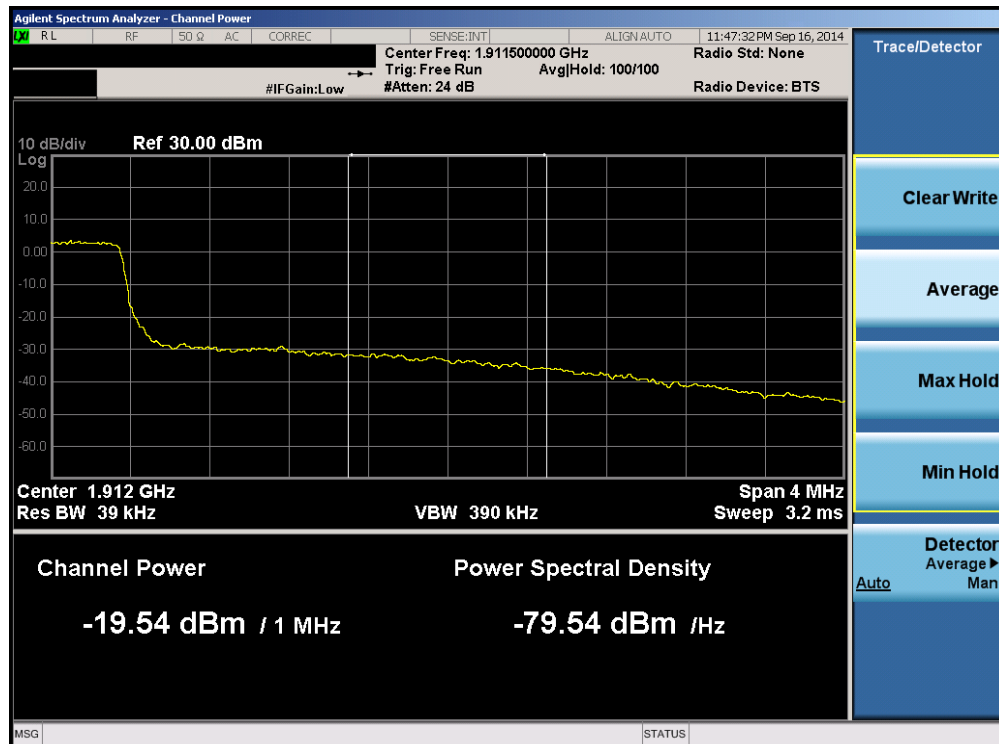
Plot 6-104. Upper Extended Band Edge Plot (Band 2 – 3.0MHz QPSK – RB Size 15)
