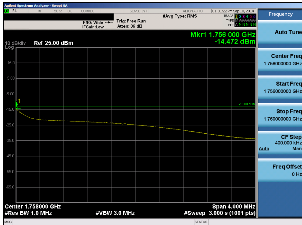
Plot 6-84. Upper Extended Band Edge Plot (Band 4 - 5.0MHz QPSK - RB Size 25)
