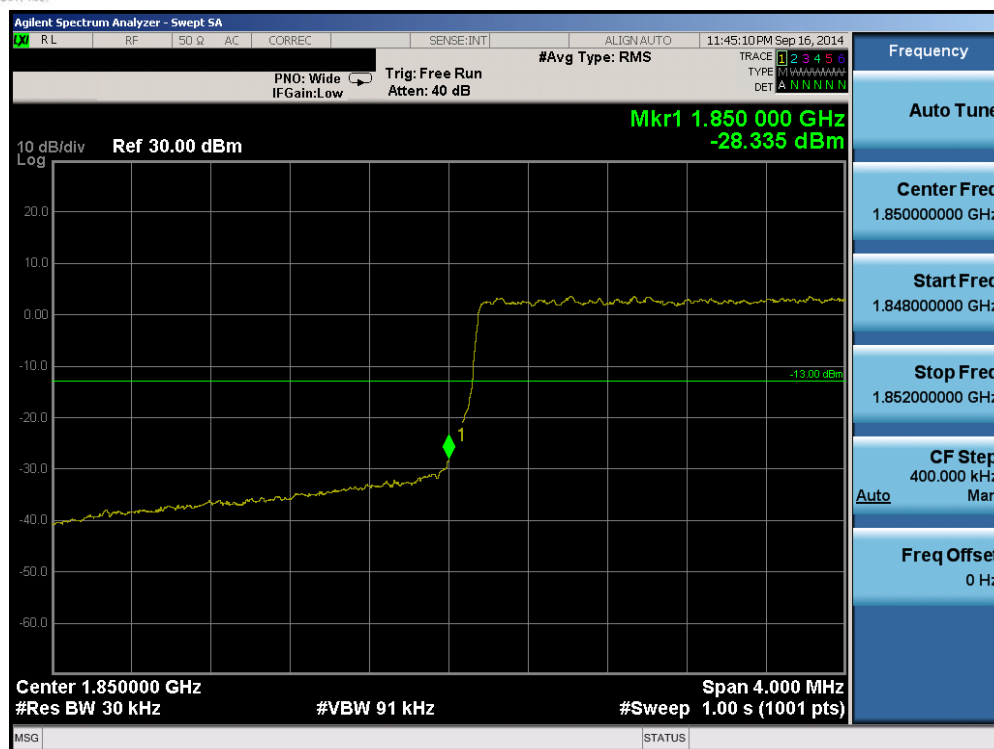
Plot 6-101. Lower Band Edge Plot (Band 2 – 3.0MHz QPSK – RB Size 15)
