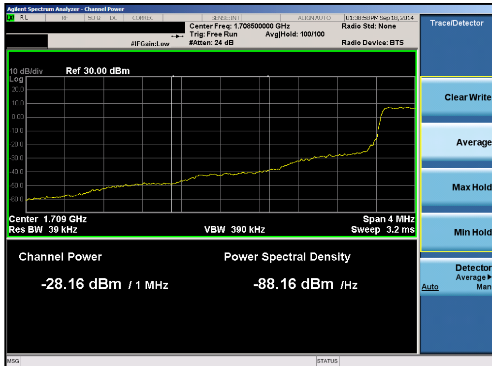
Plot 6-74. Lower Extended Band Edge Plot (Band 4 – 1.4MHz QPSK – RB Size 6)
