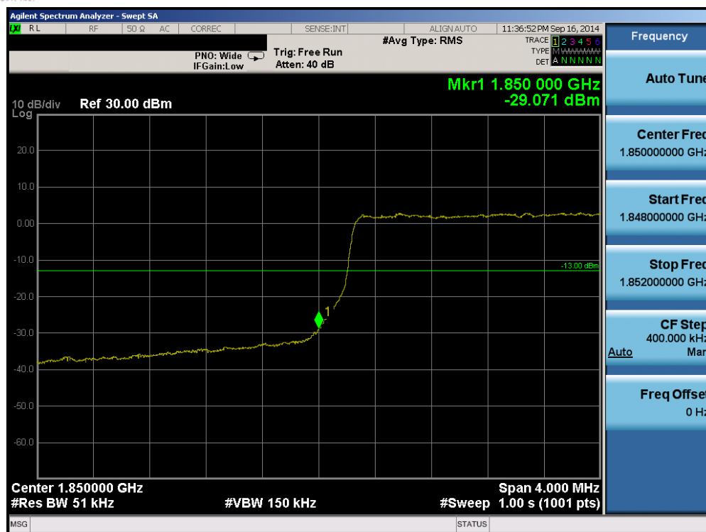
Plot 6-105. Lower Band Edge Plot (Band 2 – 5.0MHz QPSK – RB Size 25)
