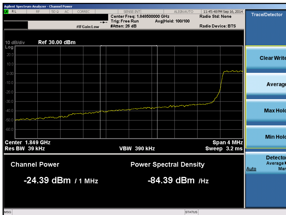
Plot 6-102. Lower Extended Band Edge Plot (Band 2 – 3.0MHz QPSK – RB Size 15)
