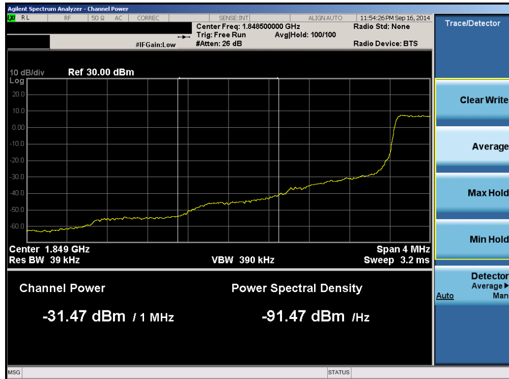
Plot 6-98. Lower Extended Band Edge Plot (Band 2 – 1.4MHz QPSK – RB Size 6)
