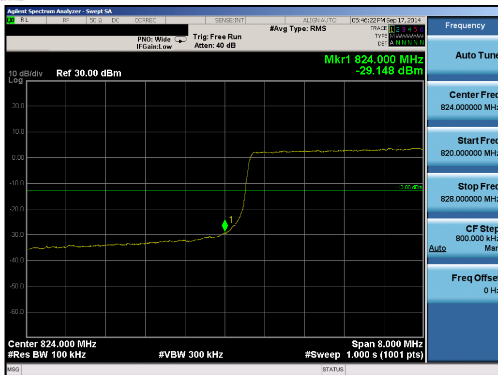
Plot 6-71. Lower Band Edge Plot (Band 5 – 10.0MHz QPSK – RB Size 50)
