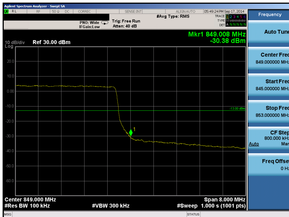
Plot 6-72. Upper Band Edge Plot (Band 5 – 10.0MHz QPSK – RB Size 50)
