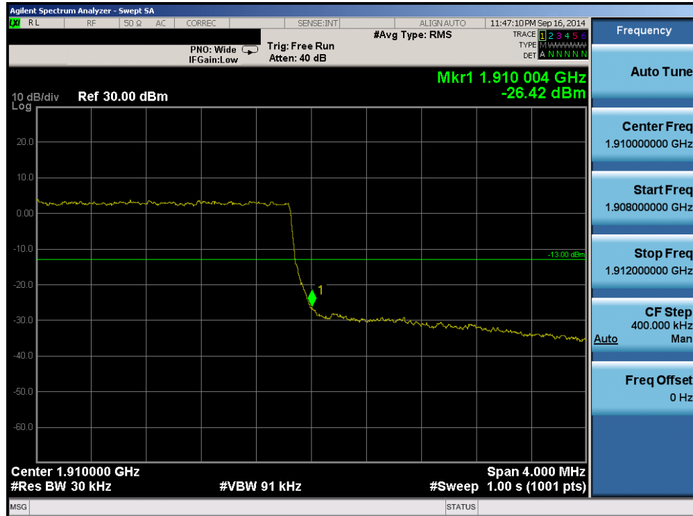
Plot 6-103. Upper Band Edge Plot (Band 2 – 3.0MHz QPSK – RB Size 15)
