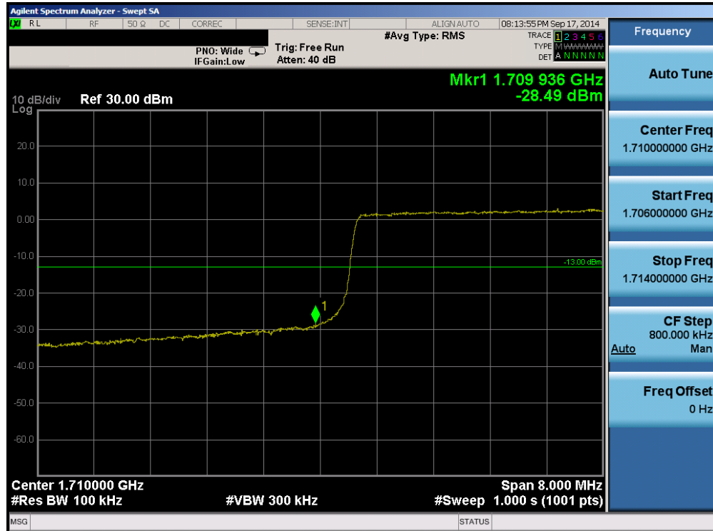
Plot 6-85. Lower Band Edge Plot (Band 4 – 10.0MHz QPSK – RB Size 50)
