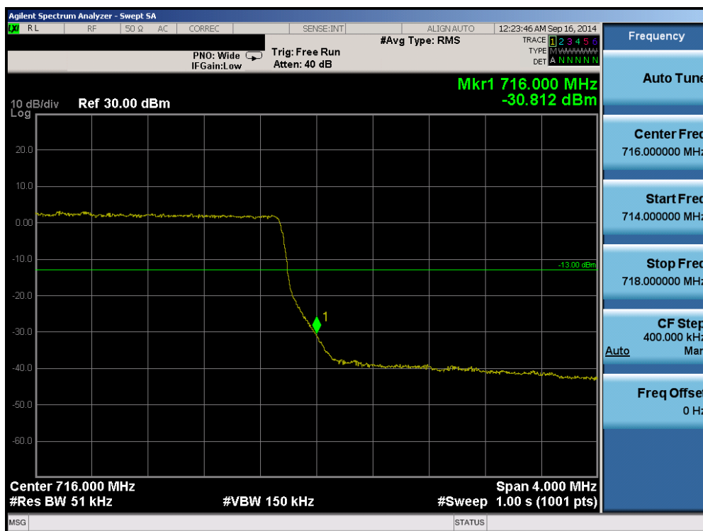
Plot 6-62. Upper Band Edge Plot (Band 17 – 5.0MHz QPSK – RB Size 25)
