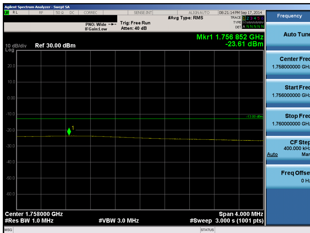
Plot 6-92. Upper Extended Band Edge Plot (Band 4 – 15.0MHz QPSK – RB Size 75)
