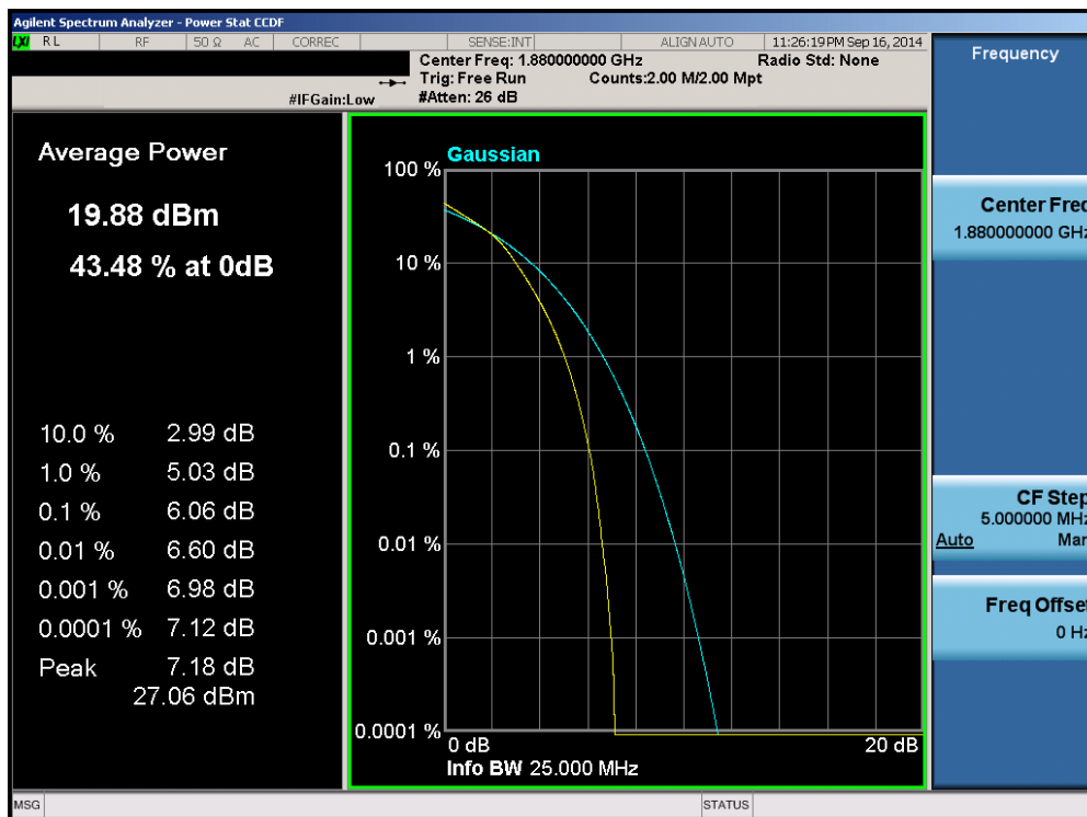
Plot 6-132. PAR Plot (Band 2 – 20.0MHz 16-QAM – RB Size 100)
