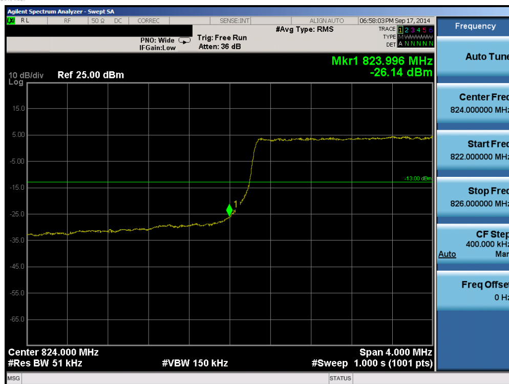
Plot 6-69. Lower Band Edge Plot (Band 5 – 5.0MHz QPSK – RB Size 25)
