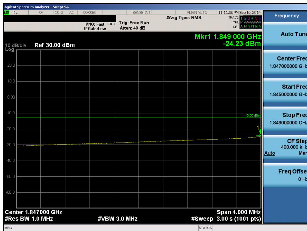
Plot 6-110. Lower Extended Band Edge Plot (Band 2 – 10.0MHz QPSK – RB Size 50)
