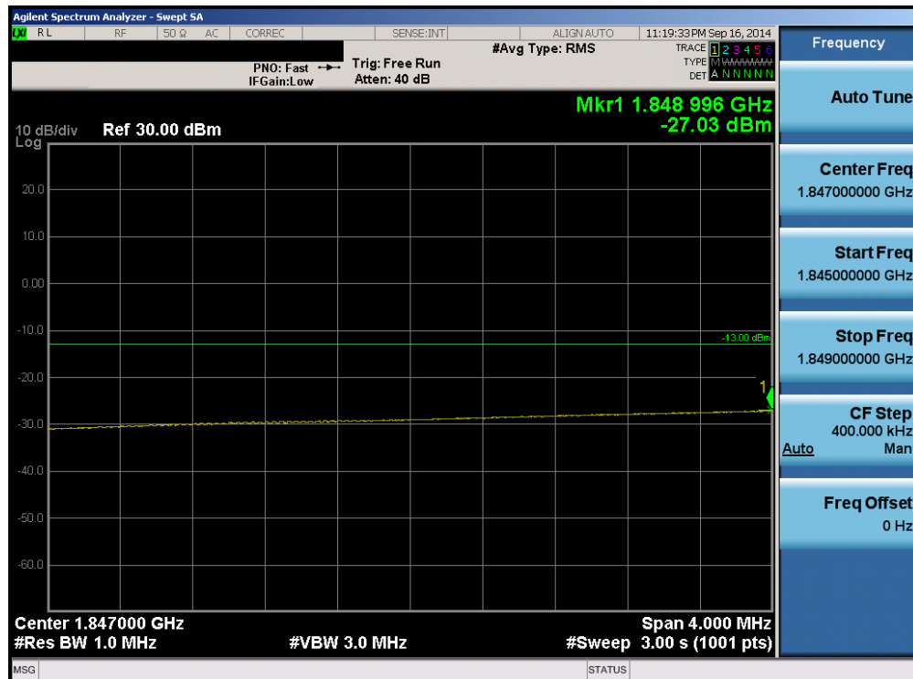
Plot 6-114. Lower Extended Band Edge Plot (Band 2 – 15.0MHz QPSK – RB Size 75)
