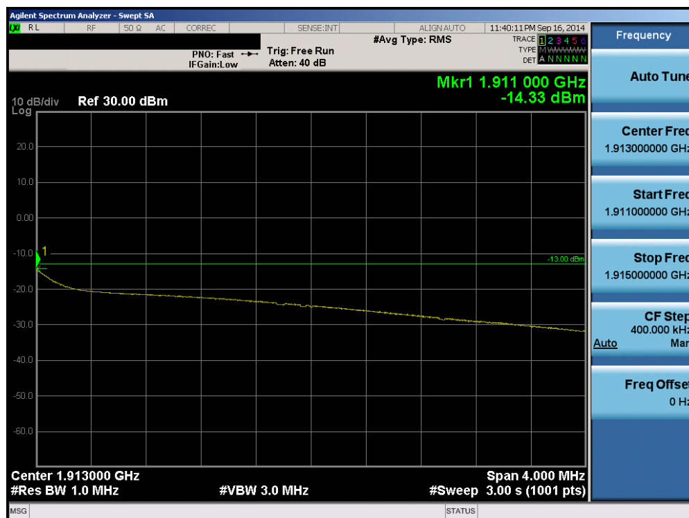
Plot 6-108. Upper Extended Band Edge Plot (Band 2 - 5.0MHz QPSK - RB Size 25)
