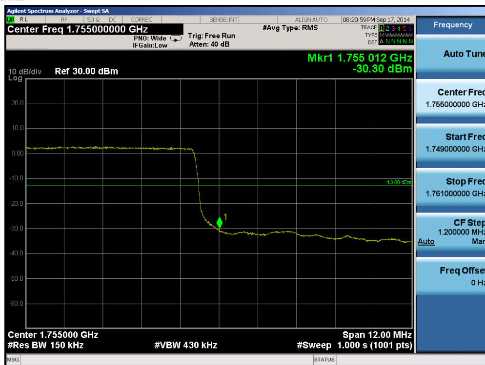
Plot 6-91. Upper Band Edge Plot (Band 4 – 15.0MHz QPSK – RB Size 75)
