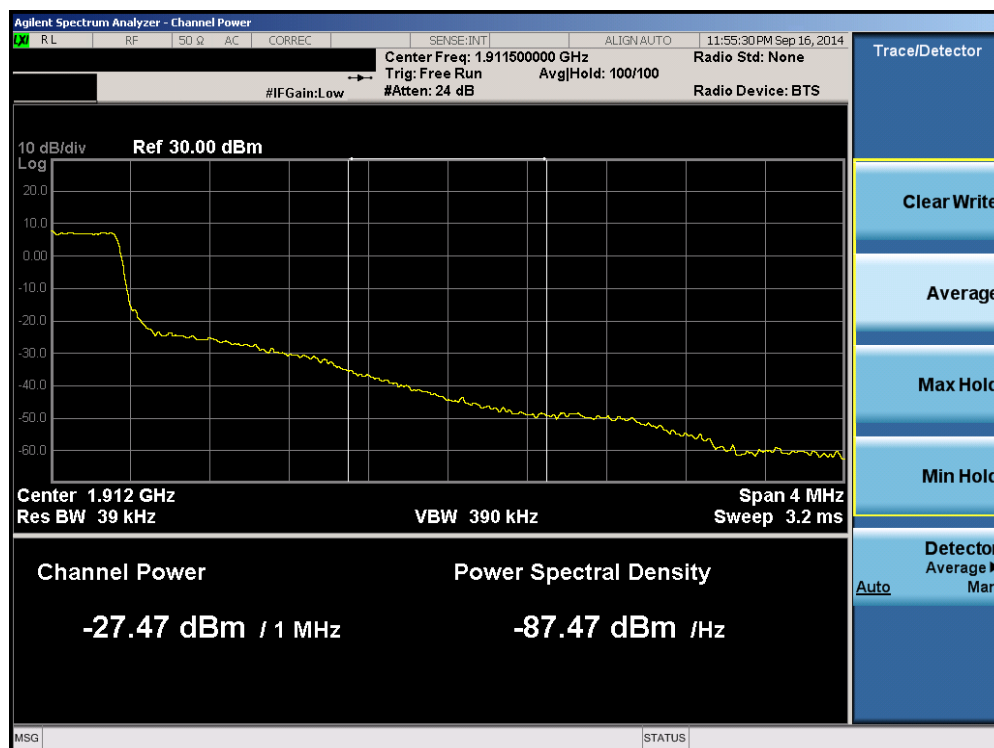
Plot 6-100. Upper Extended Band Edge Plot (Band 2 – 1.4MHz QPSK – RB Size 6)
