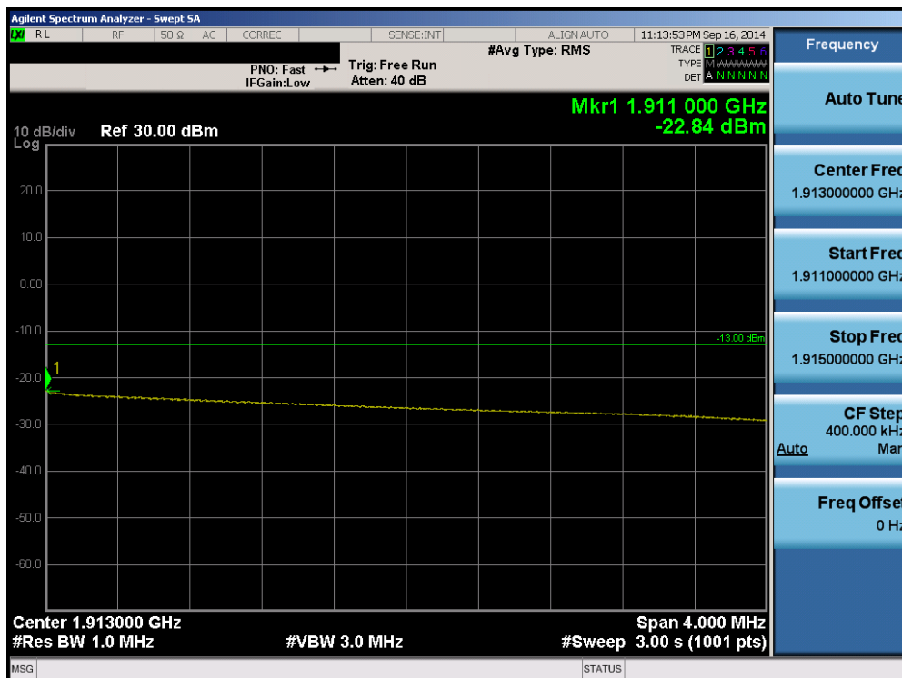
Plot 6-112. Upper Extended Band Edge Plot (Band 2 – 10.0MHz QPSK – RB Size 50)
