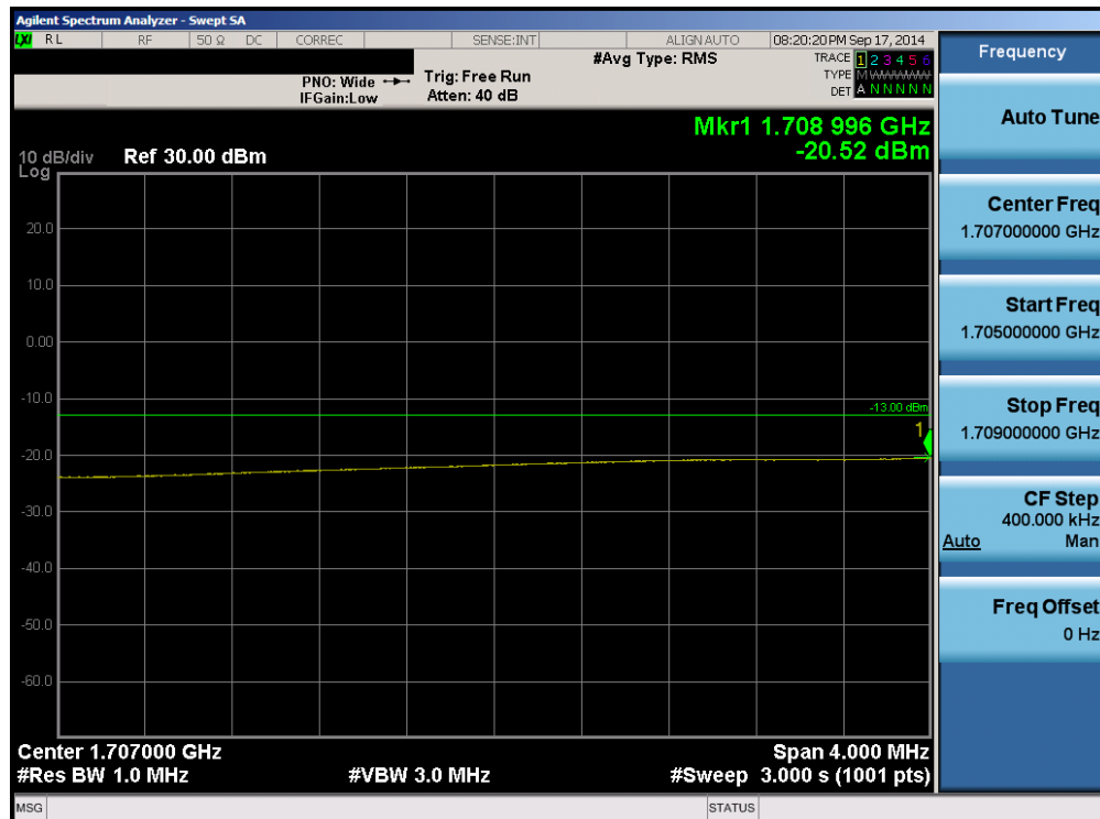
Plot 6-90. Lower Extended Band Edge Plot (Band 4 – 15.0MHz QPSK – RB Size 75)
