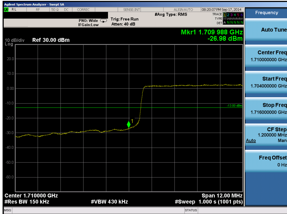
Plot 6-89. Lower Band Edge Plot (Band 4 – 15.0MHz QPSK – RB Size 75)
