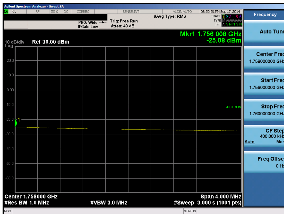
Plot 6-96. Upper Extended Band Edge Plot (Band 4 – 20.0MHz QPSK – RB Size 100)
