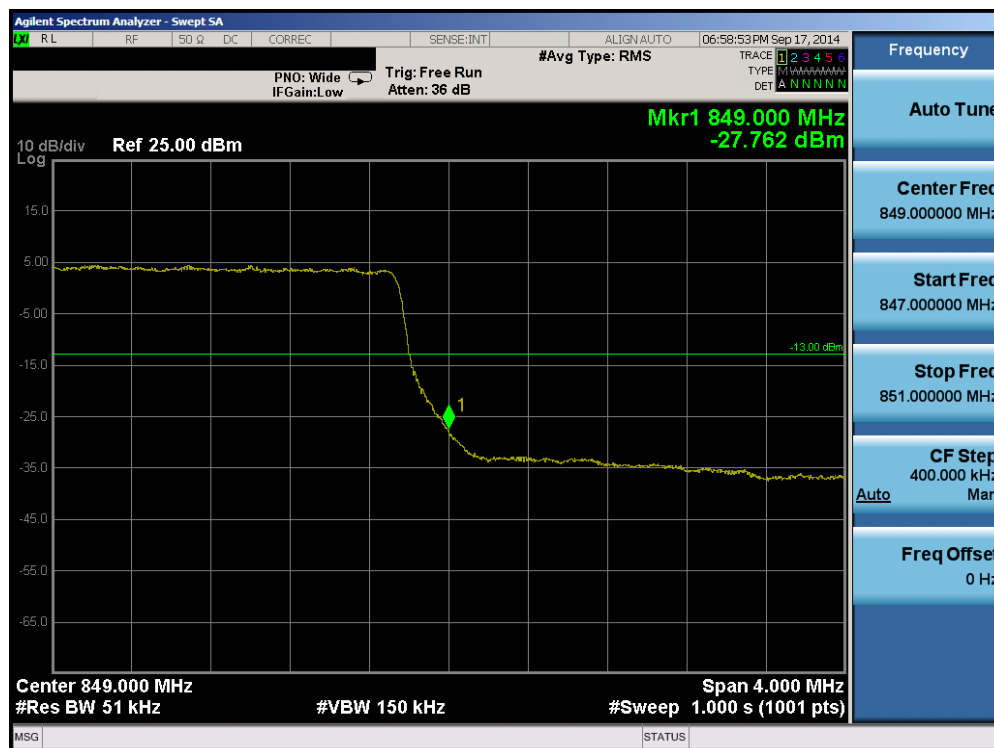
Plot 6-70. Upper Band Edge Plot (Band 5 – 5.0MHz QPSK – RB Size 25)
