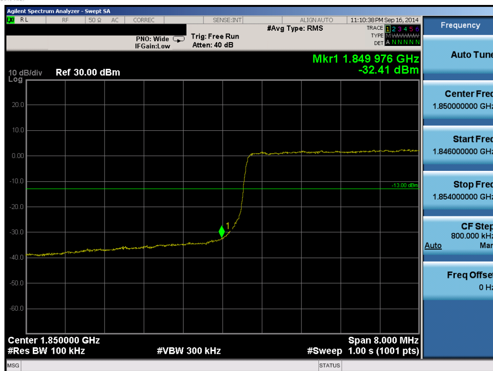
Plot 6-109. Lower Band Edge Plot (Band 2 – 10.0MHz QPSK – RB Size 50)
