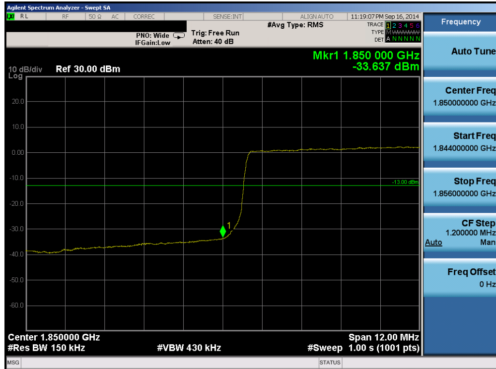
Plot 6-113. Lower Band Edge Plot (Band 2 – 15.0MHz QPSK – RB Size 75)
