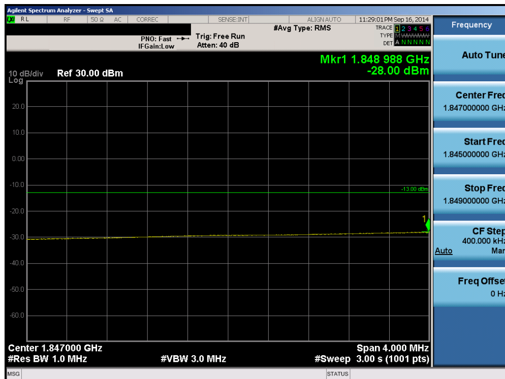
Plot 6-118. Lower Extended Band Edge Plot (Band 2 – 20.0MHz QPSK – RB Size 100)
