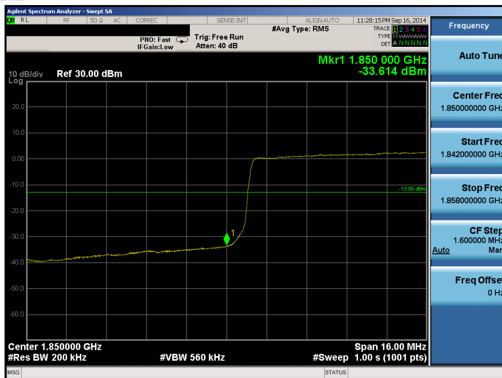
Plot 6-117. Lower Band Edge Plot (Band 2 – 20.0MHz QPSK – RB Size 100)
