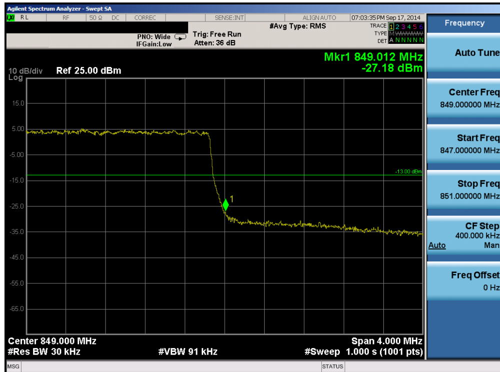
Plot 6-68. Upper Band Edge Plot (Band 5 – 3.0MHz QPSK – RB Size 15)
