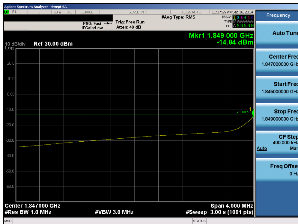
Plot 6-106. Lower Extended Band Edge Plot (Band 2 – 5.0MHz QPSK – RB Size 25)
