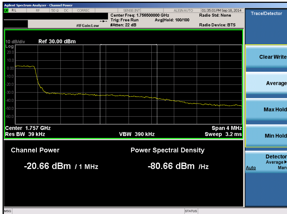
Plot 6-80. Upper Extended Band Edge Plot (Band 4 – 3.0MHz QPSK – RB Size 15)
