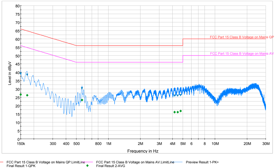
Plot 6-45. Line-Conducted Test Plot (N)
