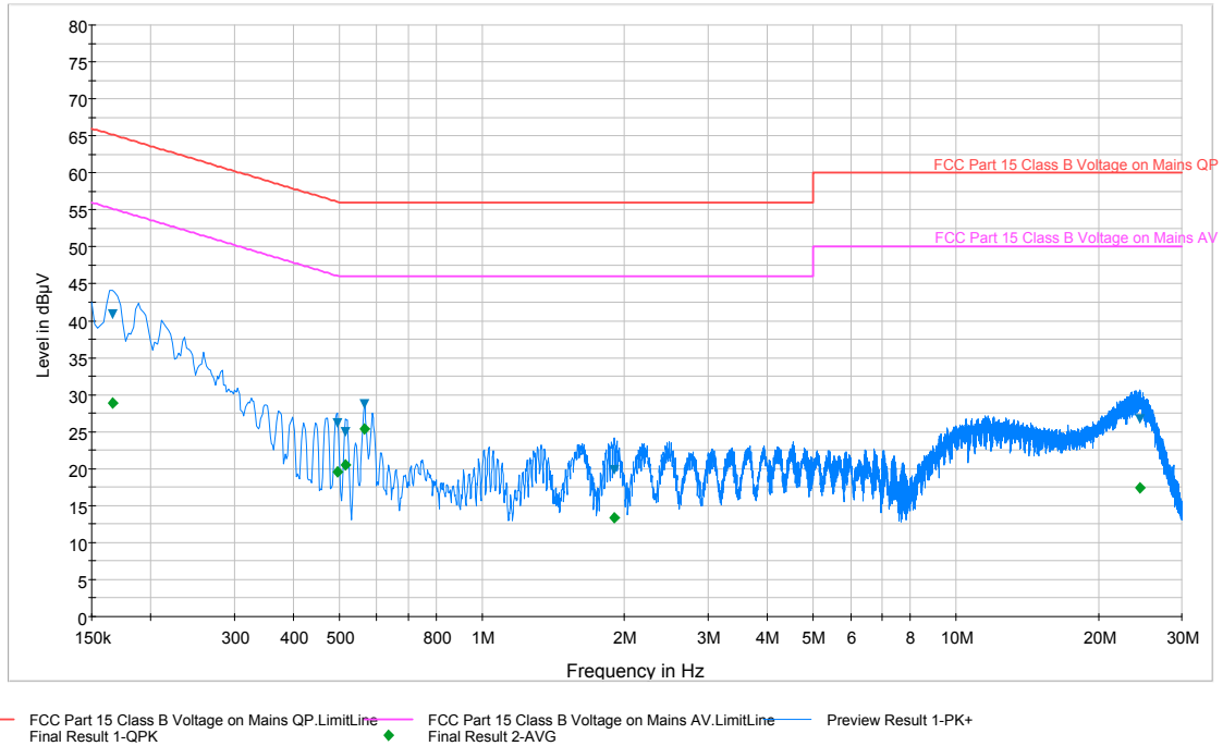
Plot 6-44. Line-Conducted Test Plot (L1)
