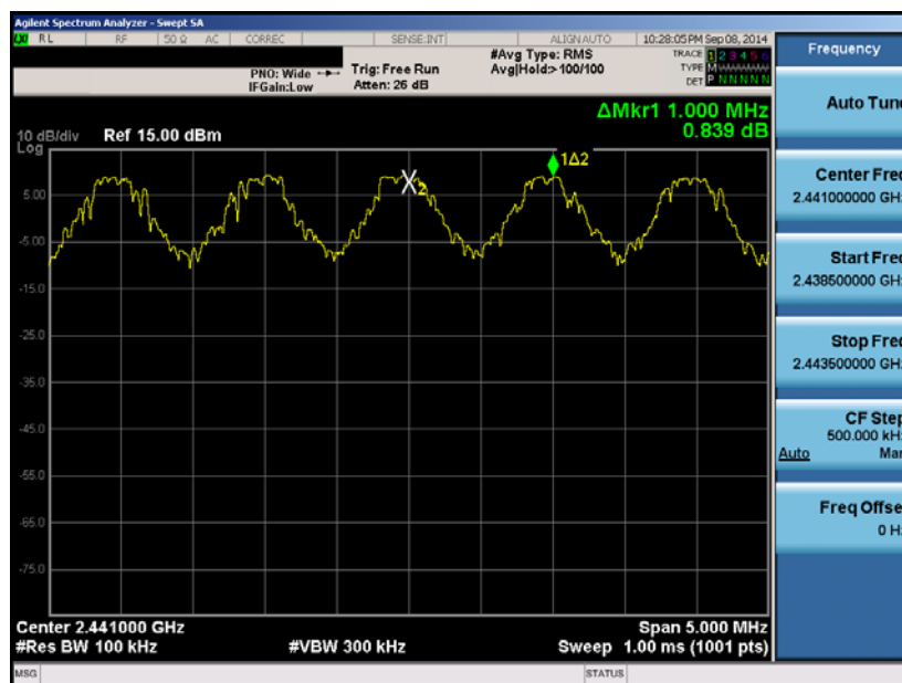
Plot 6-32. Channel Spacing Plot (Bluetooth)
