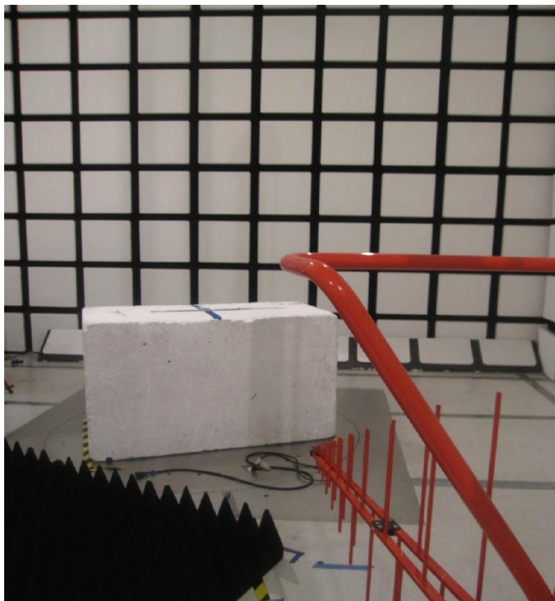
RADIATED FRONT PHOTO (BELOW 1 GHz)
