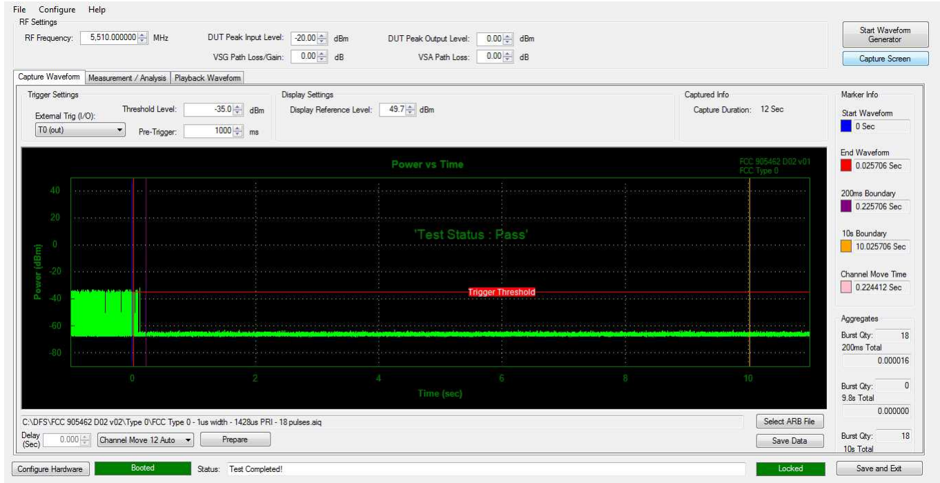
Figure 5-2. Band 2C Move Time and Aggregate Time
