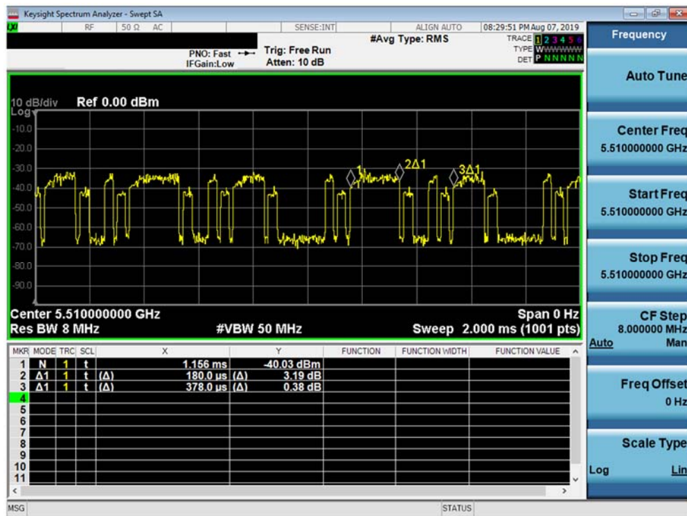
Figure 5-1. Band 2C Pulse Width and period
