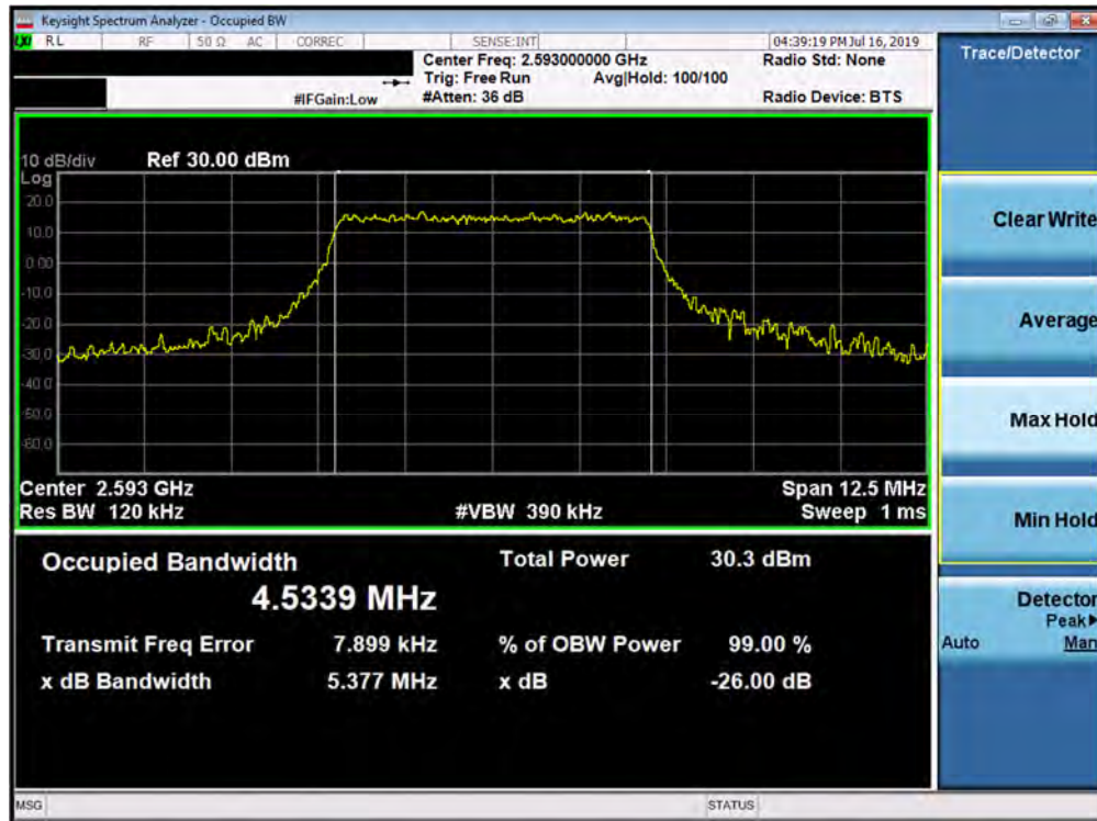
Plot 7-9. Occupied Bandwidth Plot (Band 41 - 5.0MHz QPSK - Full RB Configuration)
