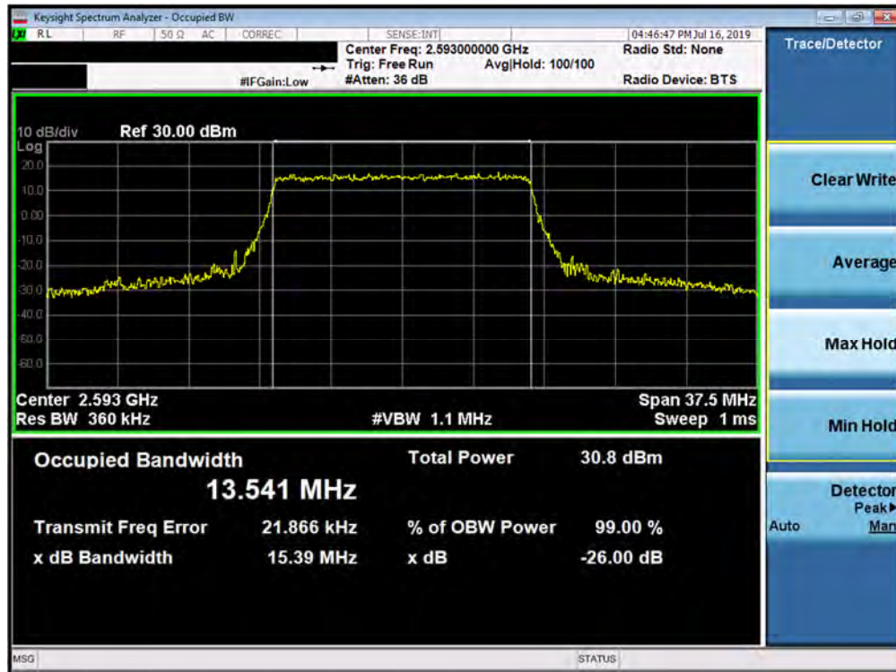
Plot 7-13. Occupied Bandwidth Plot (Band 41 - 15.0MHz QPSK - Full RB Configuration)
