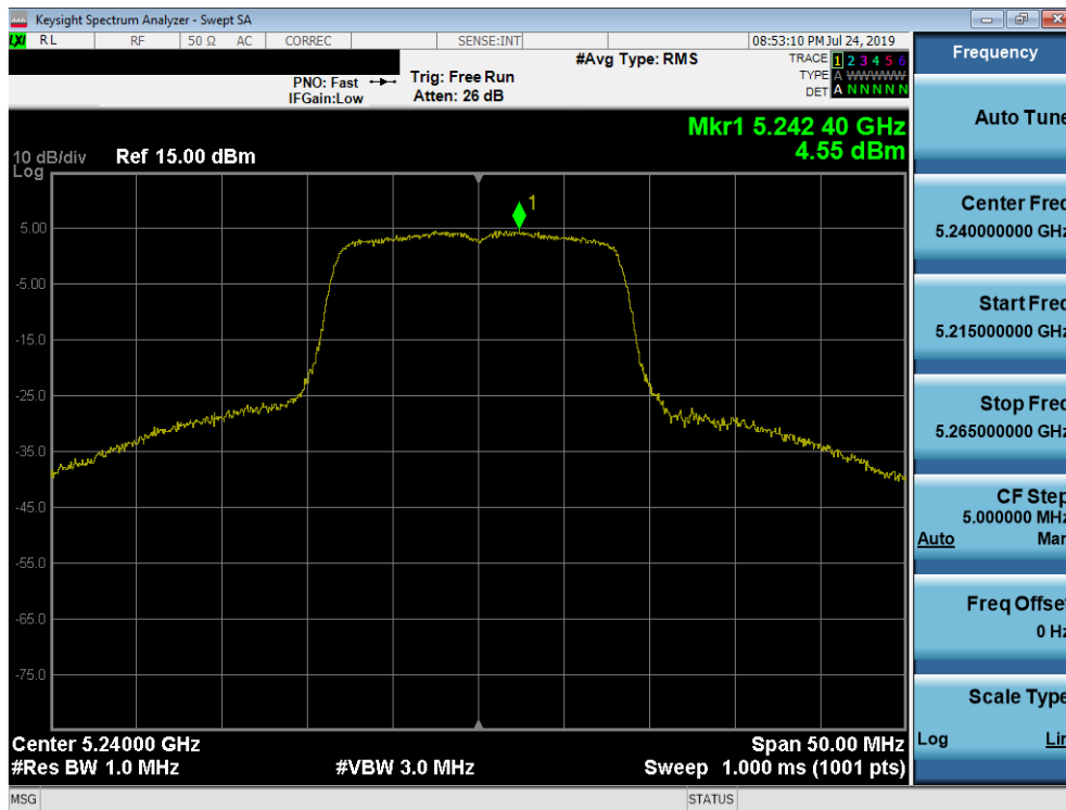
Plot 7-42. Power Spectral Density Plot (802.11a (UNII Band 1) – Ch. 48)
