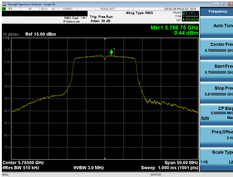
Plot 7-71. Power Spectral Density Plot (802.11a (UNII Band 3) – Ch. 157)
