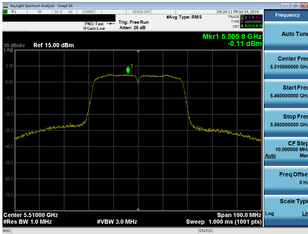
Plot 7-64. Power Spectral Density Plot (40MHz BW 802.11n (UNII Band 2C) – Ch. 102)
