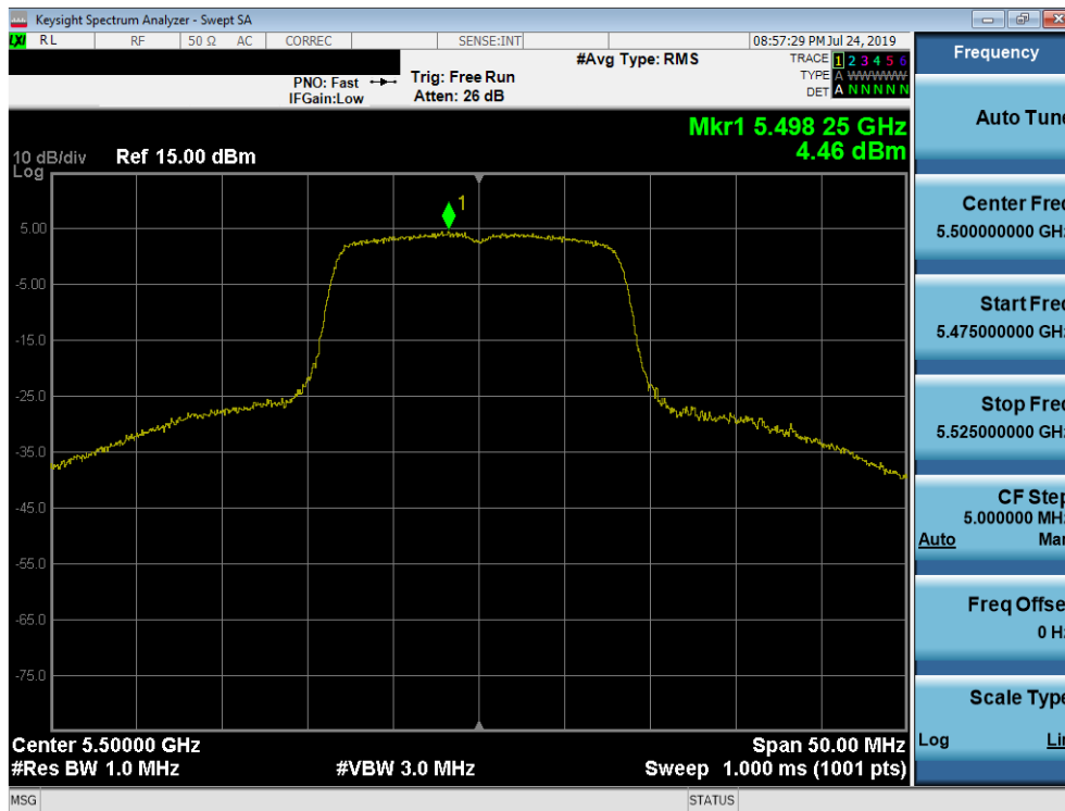
Plot 7-58. Power Spectral Density Plot (802.11a (UNII Band 2C) – Ch. 100)
