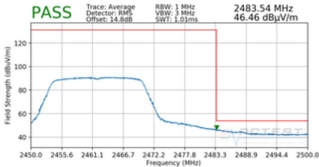
Plot 7-43. Radiated Restricted Upper Band Edge Measurement (Average)
