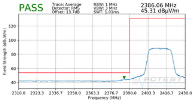
Plot 7-41. Radiated Restricted Lower Band Edge Measurement (Average)
