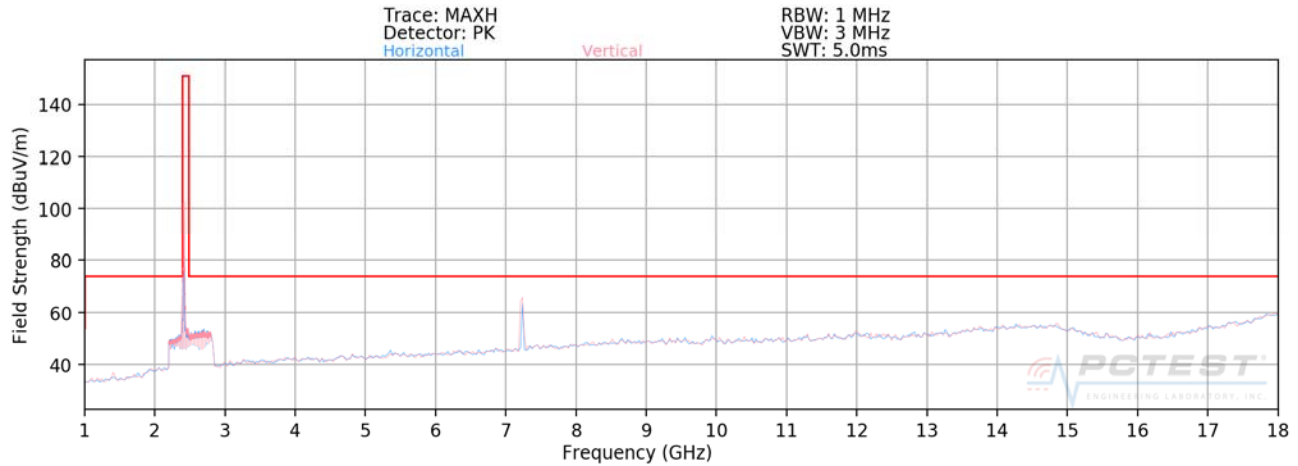
Plot 7-37. Radiated Spurious Plot above 1GHz (802.11b – Ch. 1)
