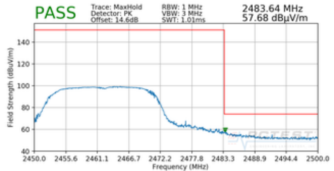
Plot 7-44. Radiated Restricted Upper Band Edge Measurement (Peak)
