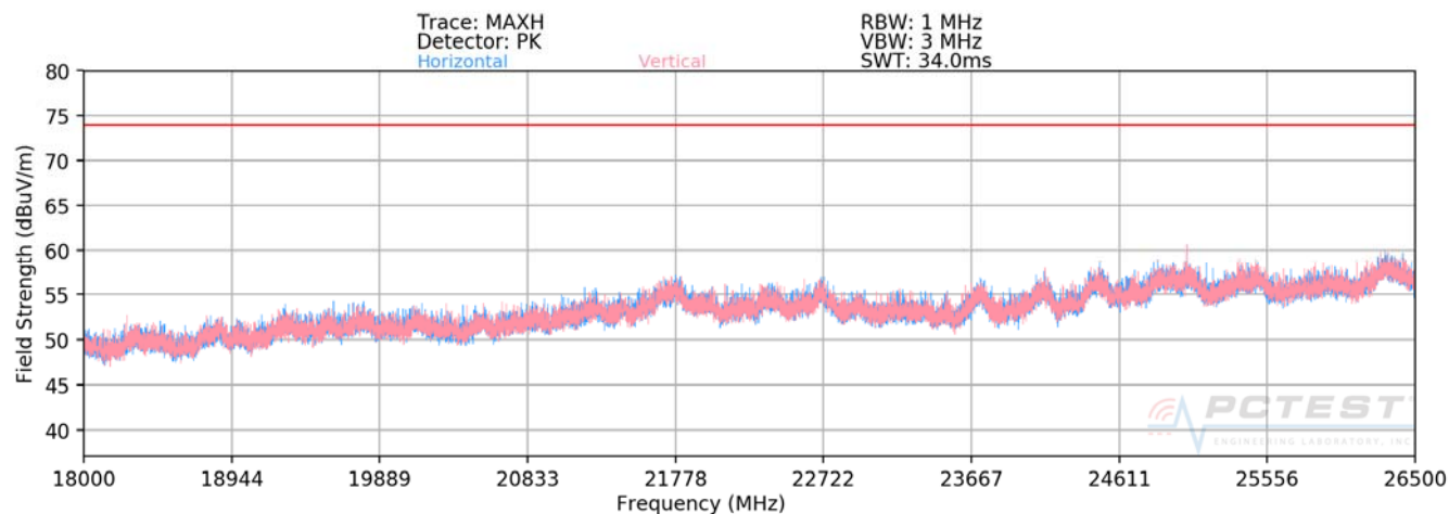
Plot 7-40. Radiated Spurious Plot above 18GHz
