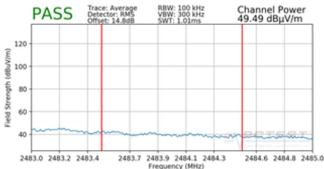
Plot 7-47. Radiated Restricted Upper Band Edge Measurement (Average)
