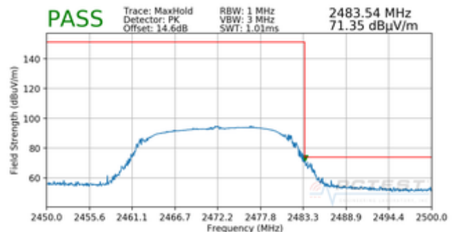
Plot 7-48. Radiated Restricted Upper Band Edge Measurement (Peak)
