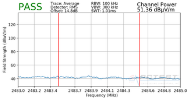
Plot 7-45. Radiated Restricted Upper Band Edge Measurement (Average)
