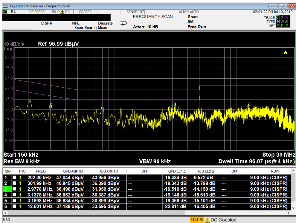
Plot 7-50. Line Conducted Plot with 802.11b (L1)
