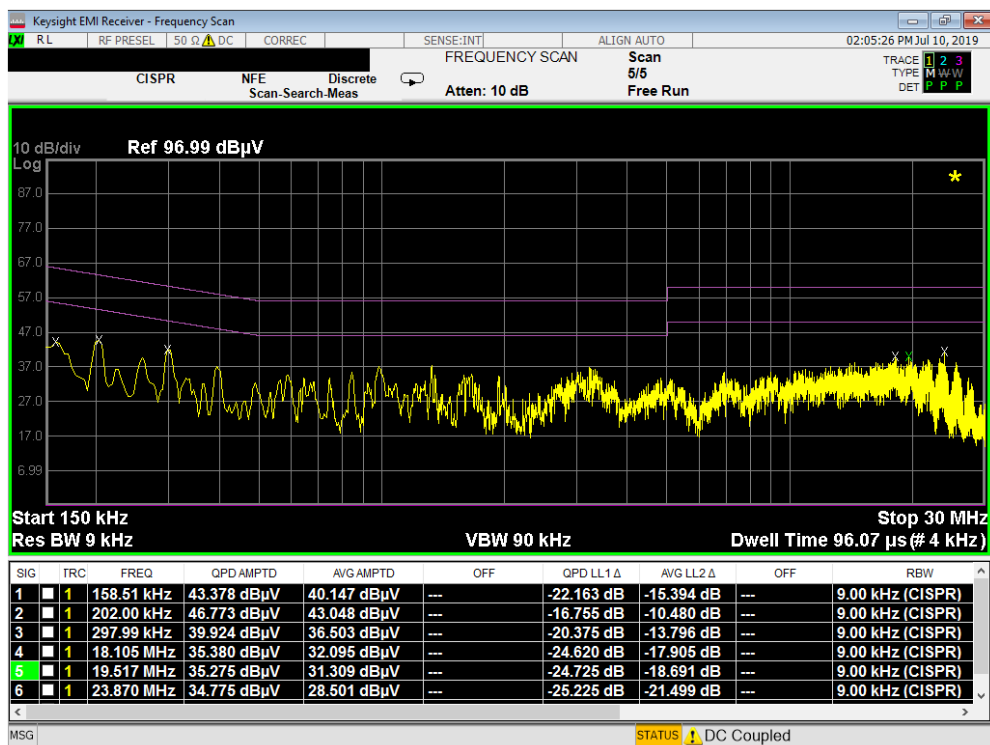
Plot 7-51. Line Conducted Plot with 802.11b (N)
