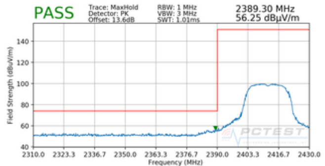
Plot 7-42. Radiated Restricted Lower Band Edge Measurement (Peak)
