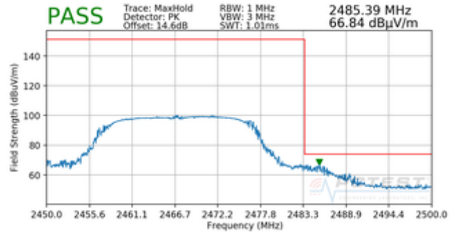
Plot 7-46. Radiated Restricted Upper Band Edge Measurement (Peak)
