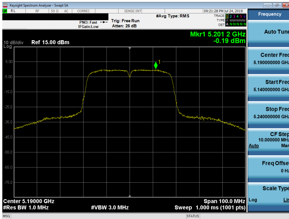
Plot 7-46. Power Spectral Density Plot (40MHz BW 802.11n (UNII Band 1) – Ch. 38)
