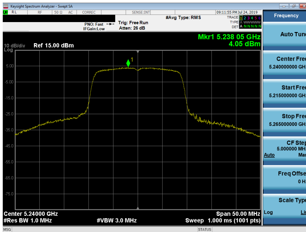
Plot 7-45. Power Spectral Density Plot (20MHz BW 802.11n (UNII Band 1) – Ch. 48)
