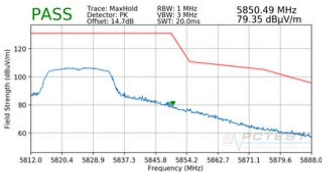
Plot 7-91. Radiated Upper Band Edge Plot (Peak – UNII Band 3)
